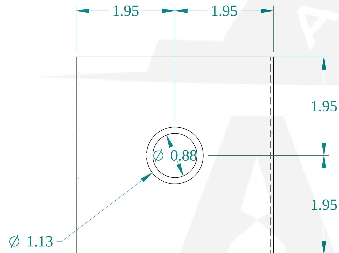
FRONT VIEW
