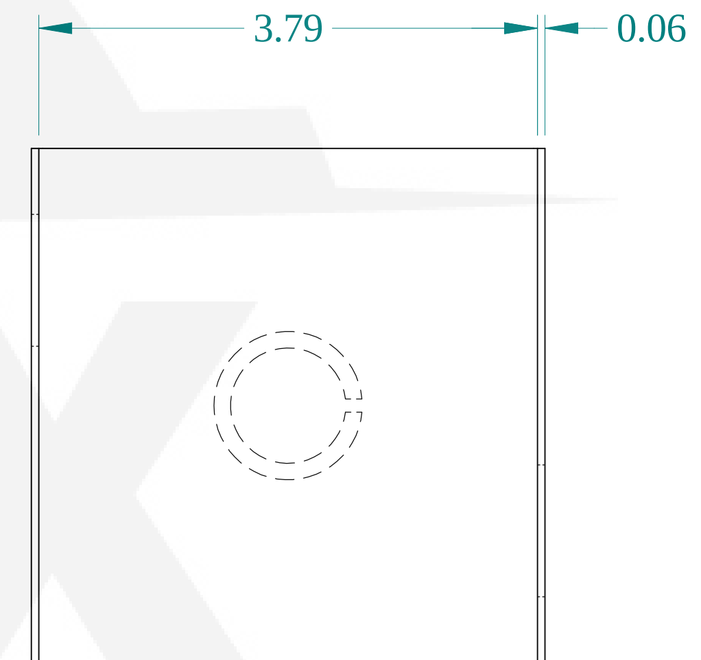
BACK VIEW
