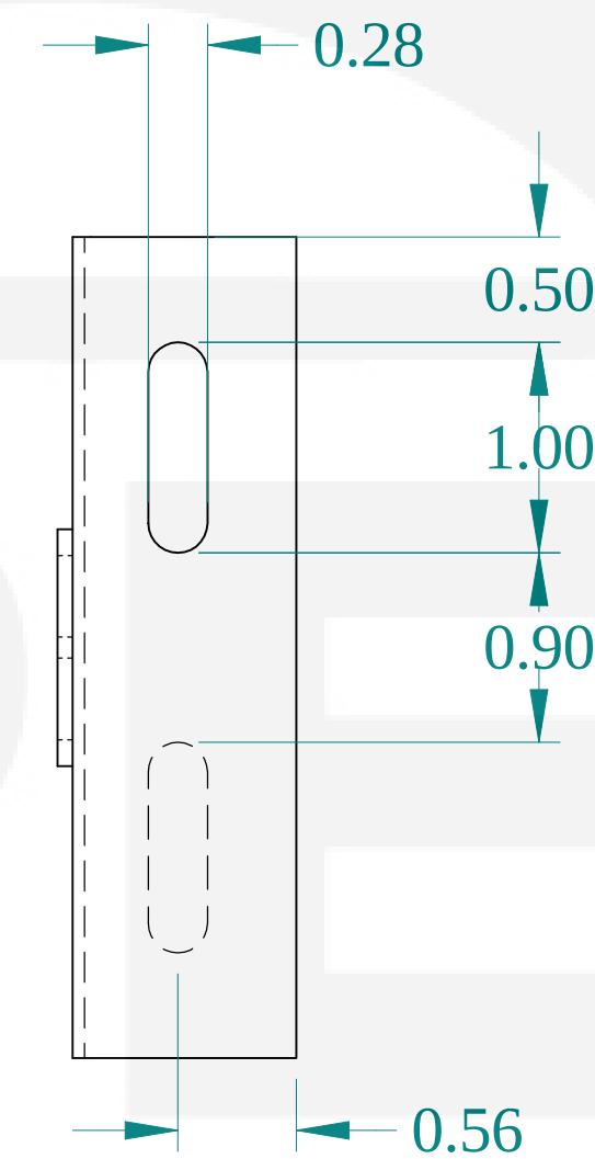
SIDE VIEW
