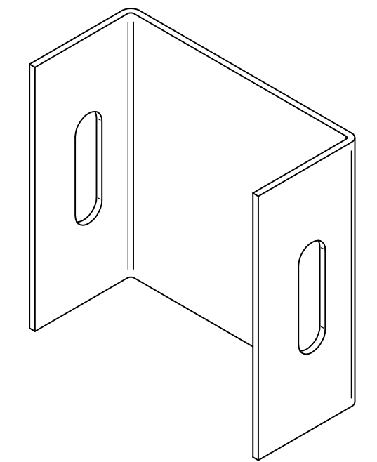
ISOMETRIC VIEWS
