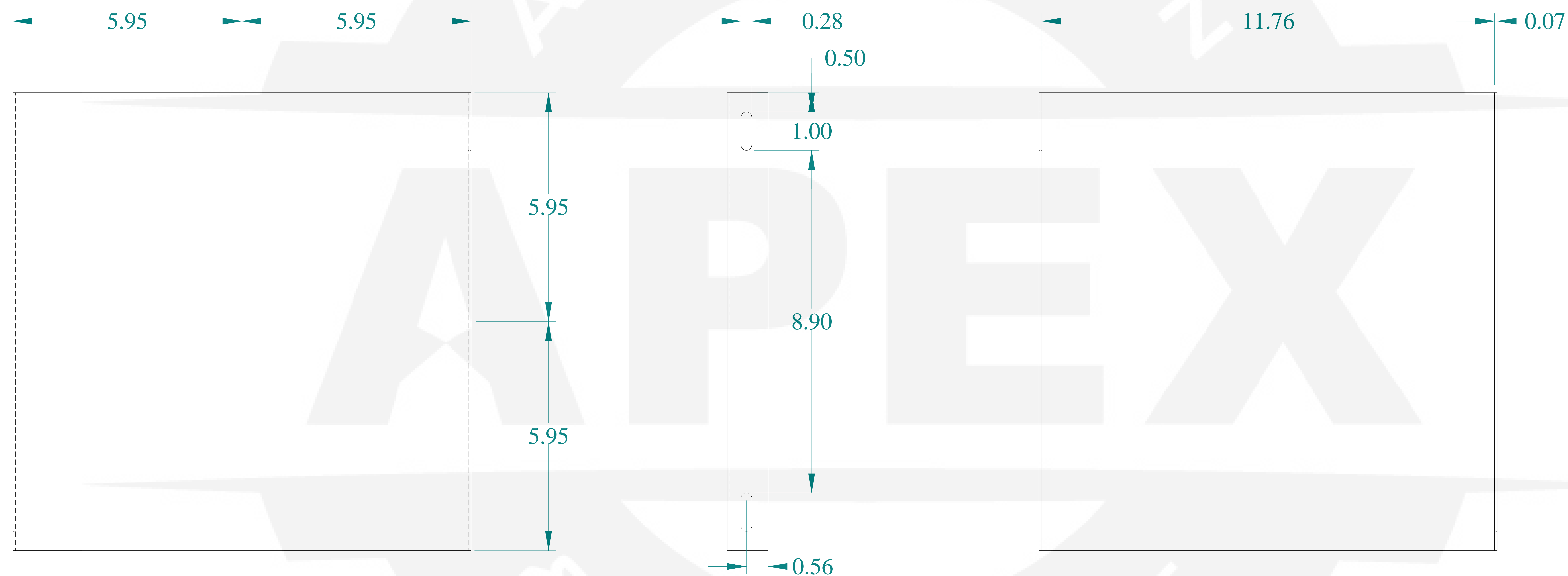
BACK VIEW
