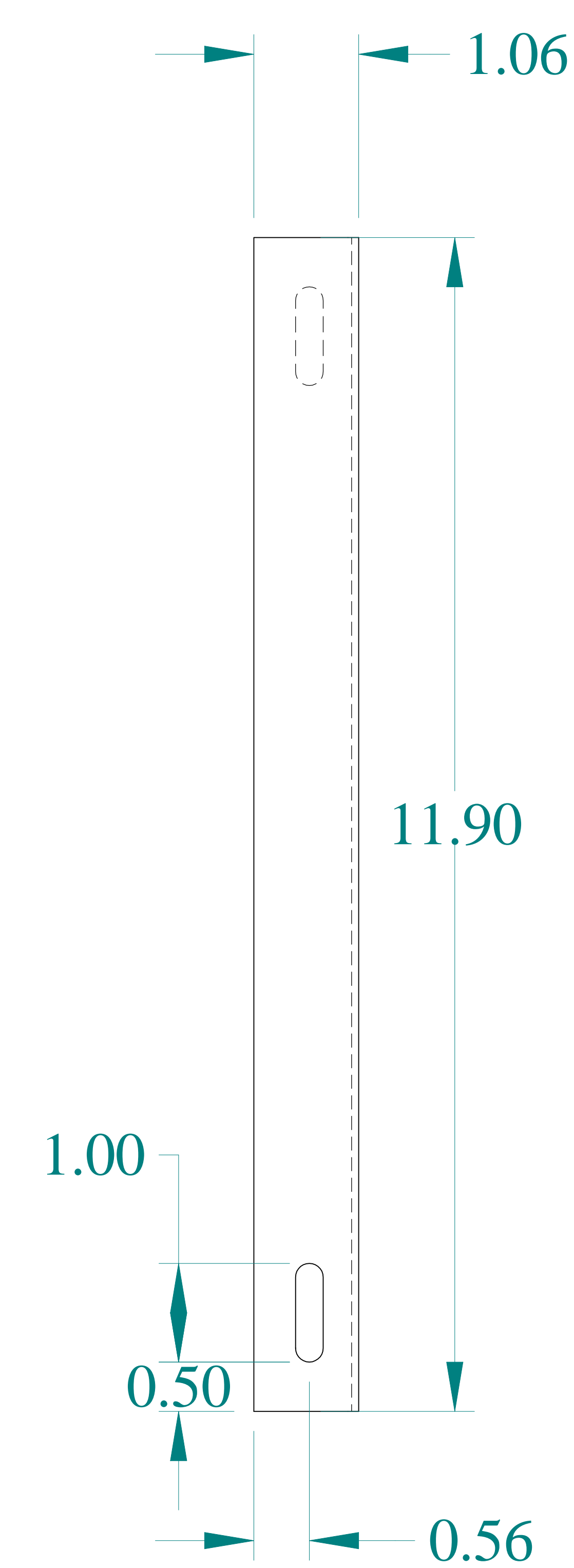
SIDE VIEW
