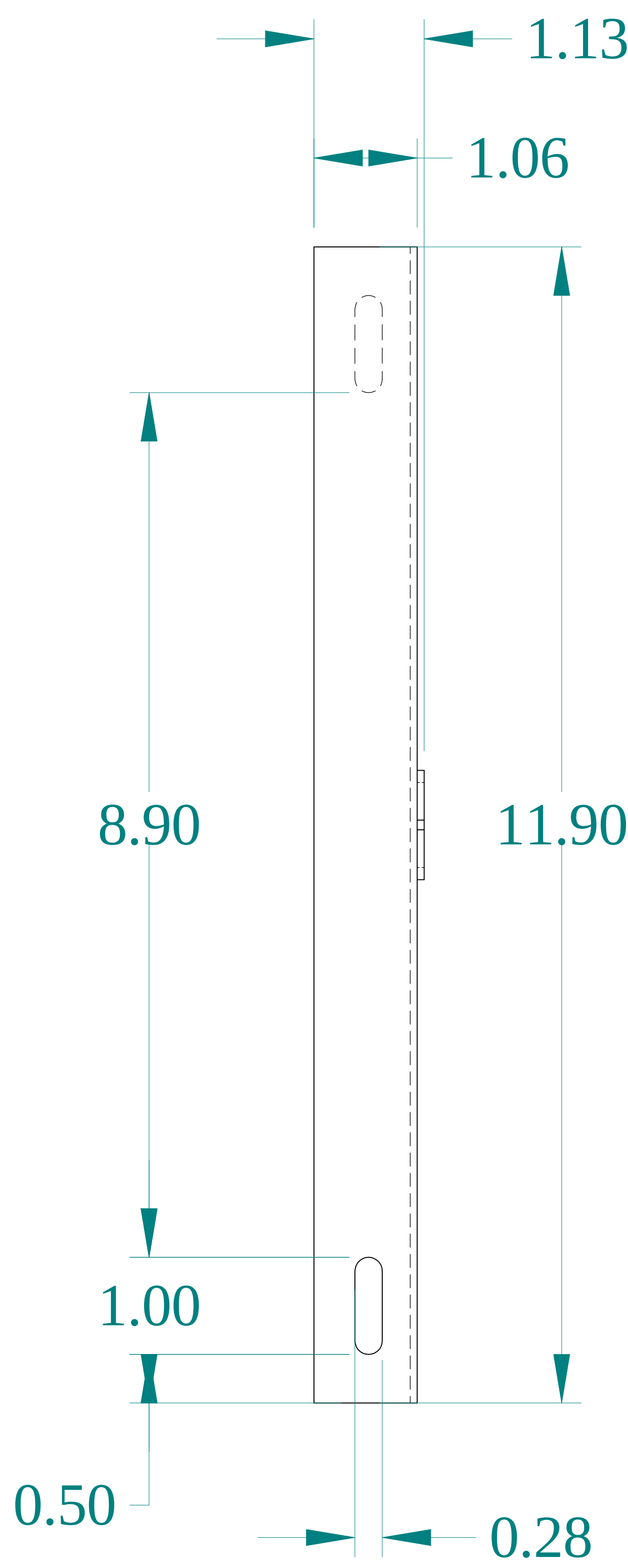
SIDE VIEW
