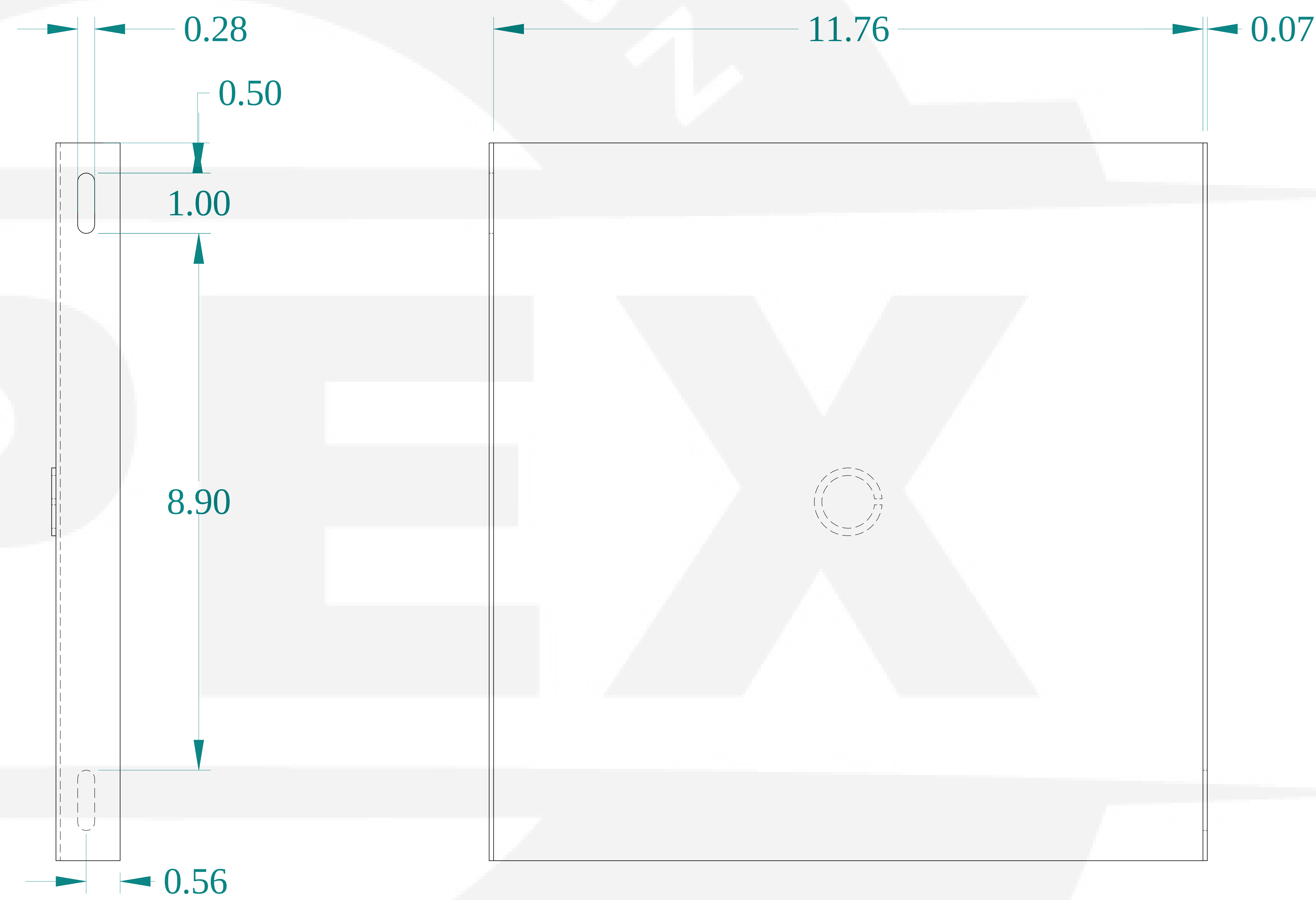
BACK VIEW
