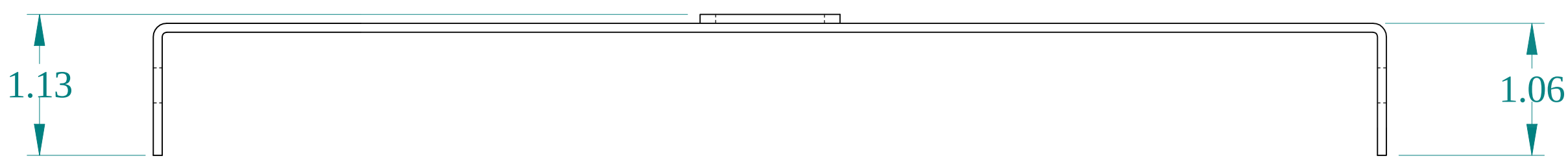
BOTTOM VIEW
