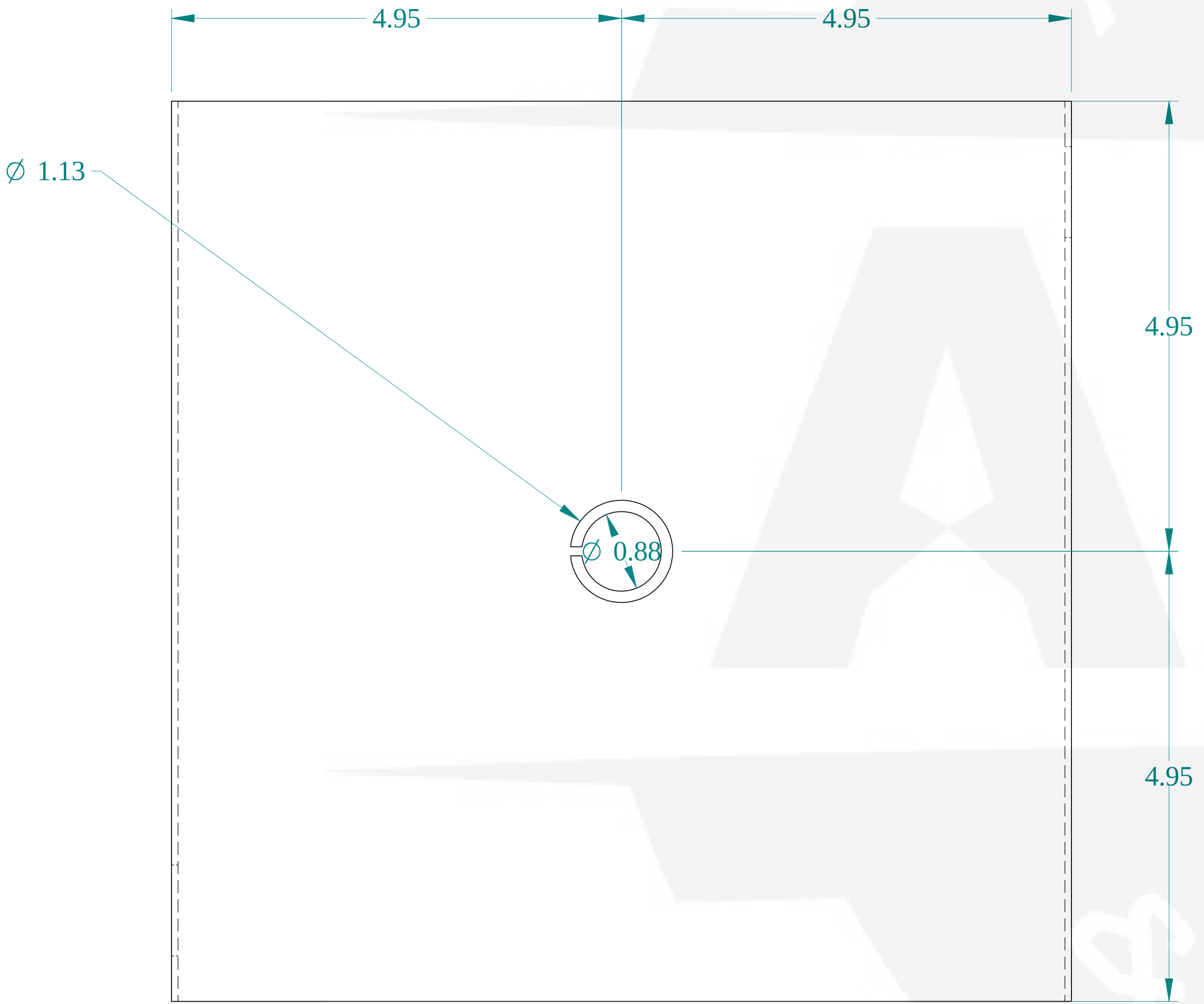
FRONT VIEW
