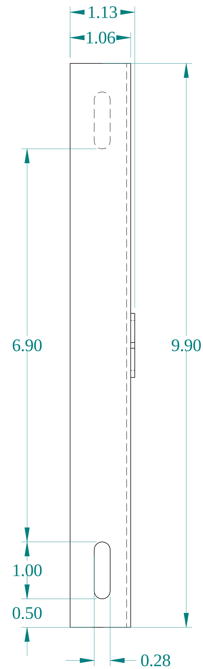
SIDE VIEW
