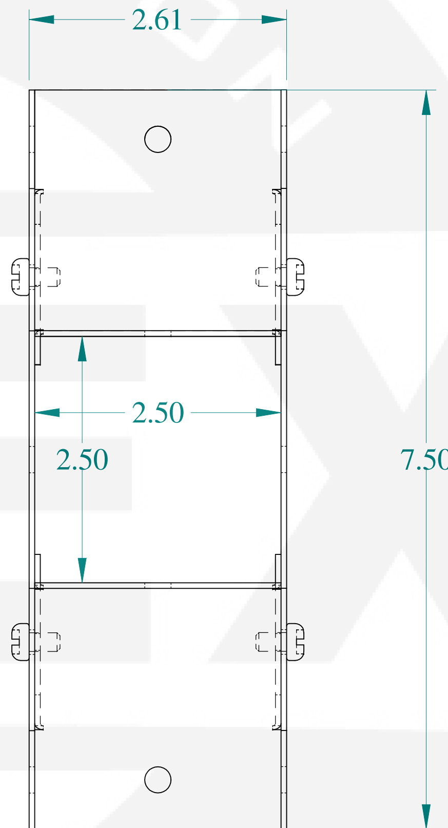
SIDE VIEW
