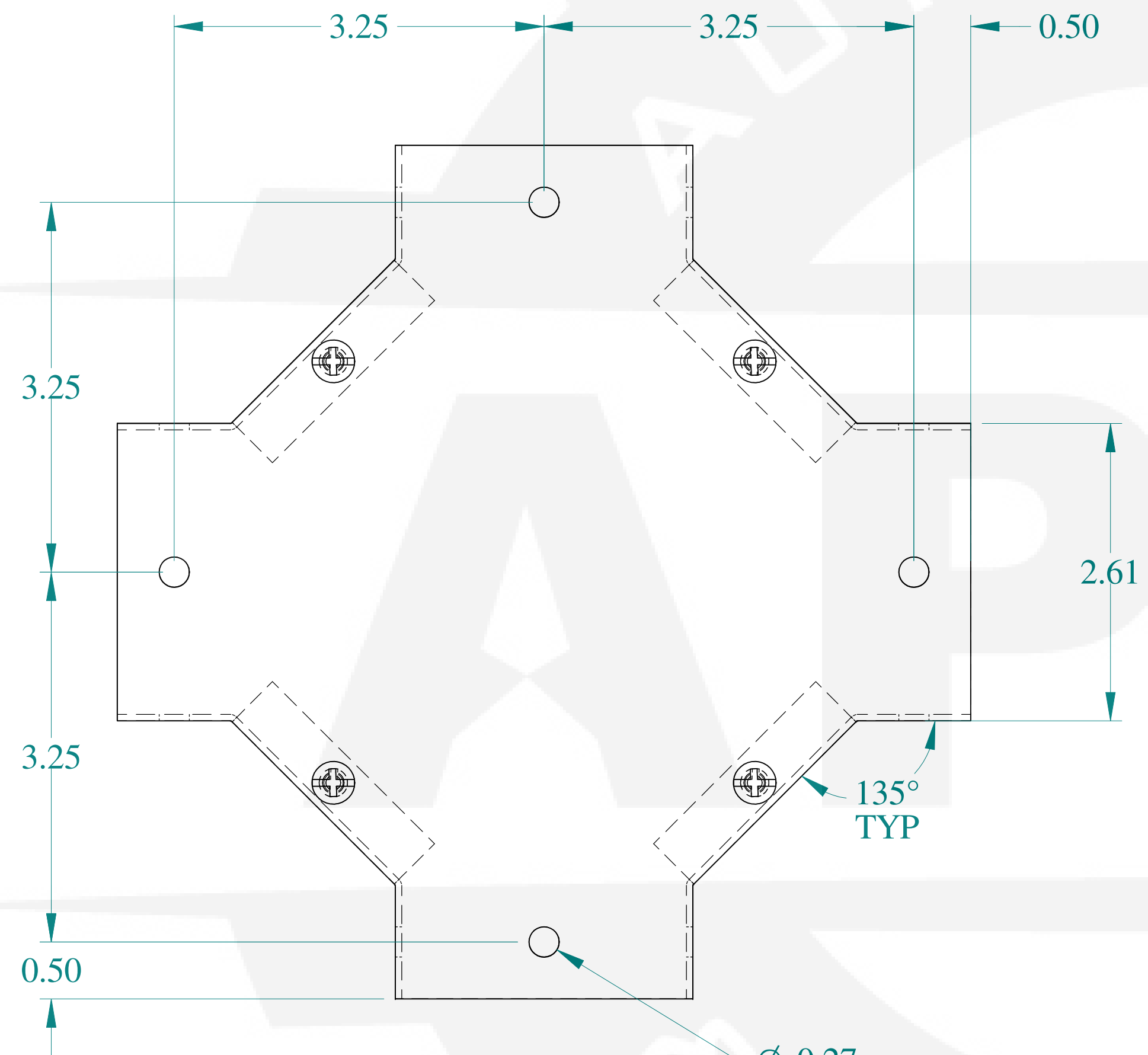
TOP VIEW
