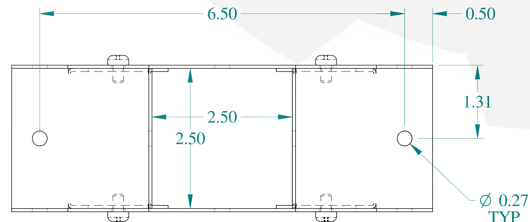
BOTTOM VIEW
