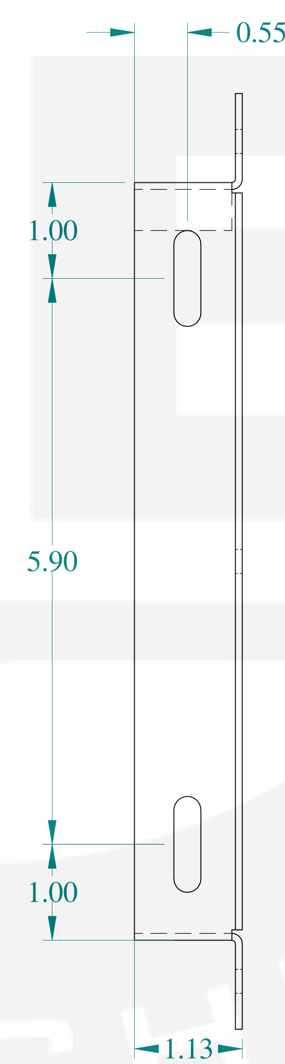
SIDE VIEW
