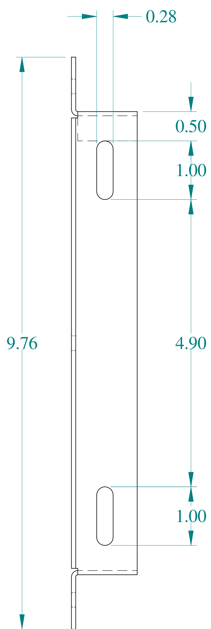
SIDE VIEW
