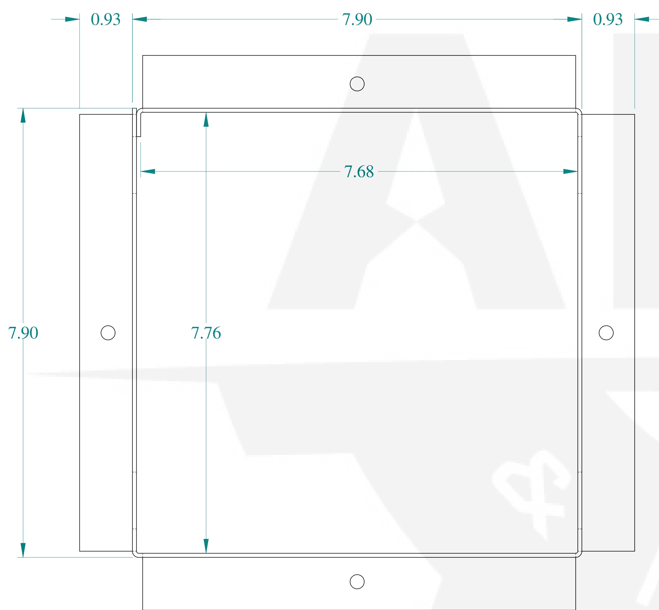
FRONT VIEW
