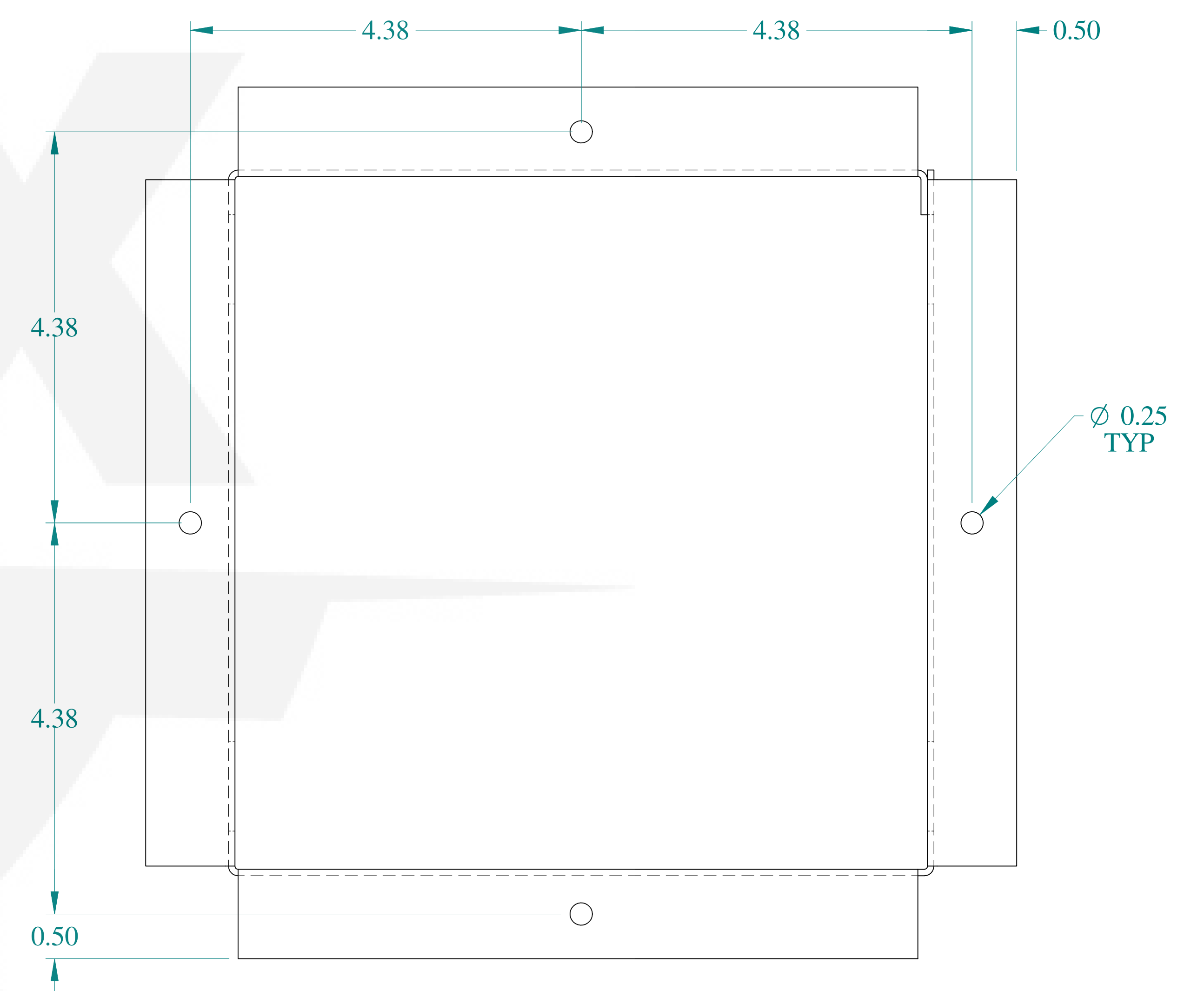
BACK VIEW
