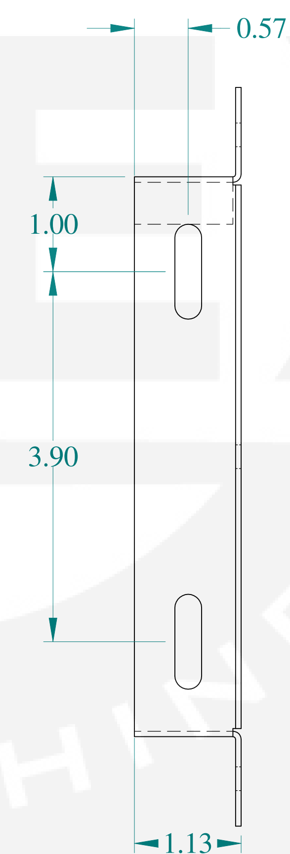
SIDE VIEW
