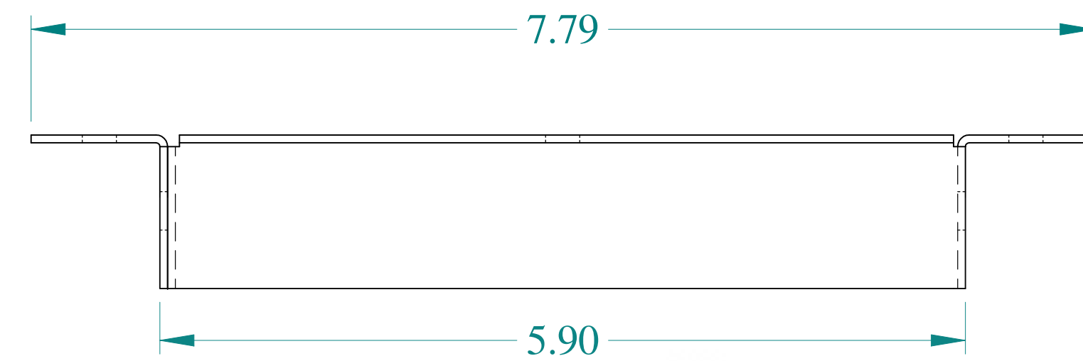
TOP VIEW
