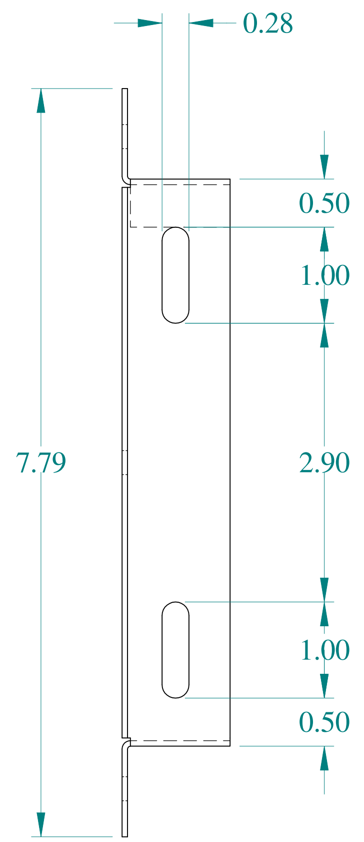
SIDE VIEW
