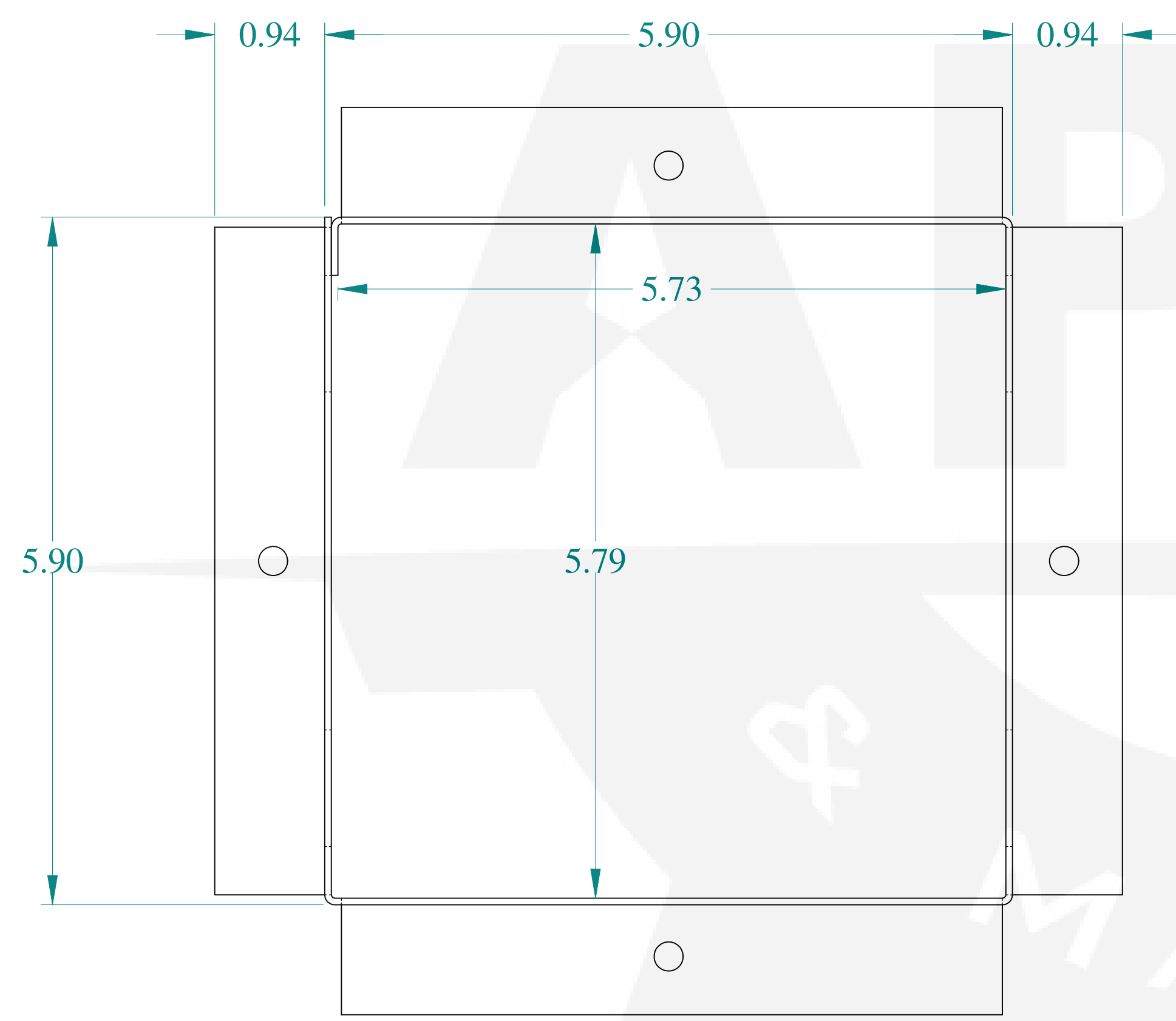
FRONT VIEW
