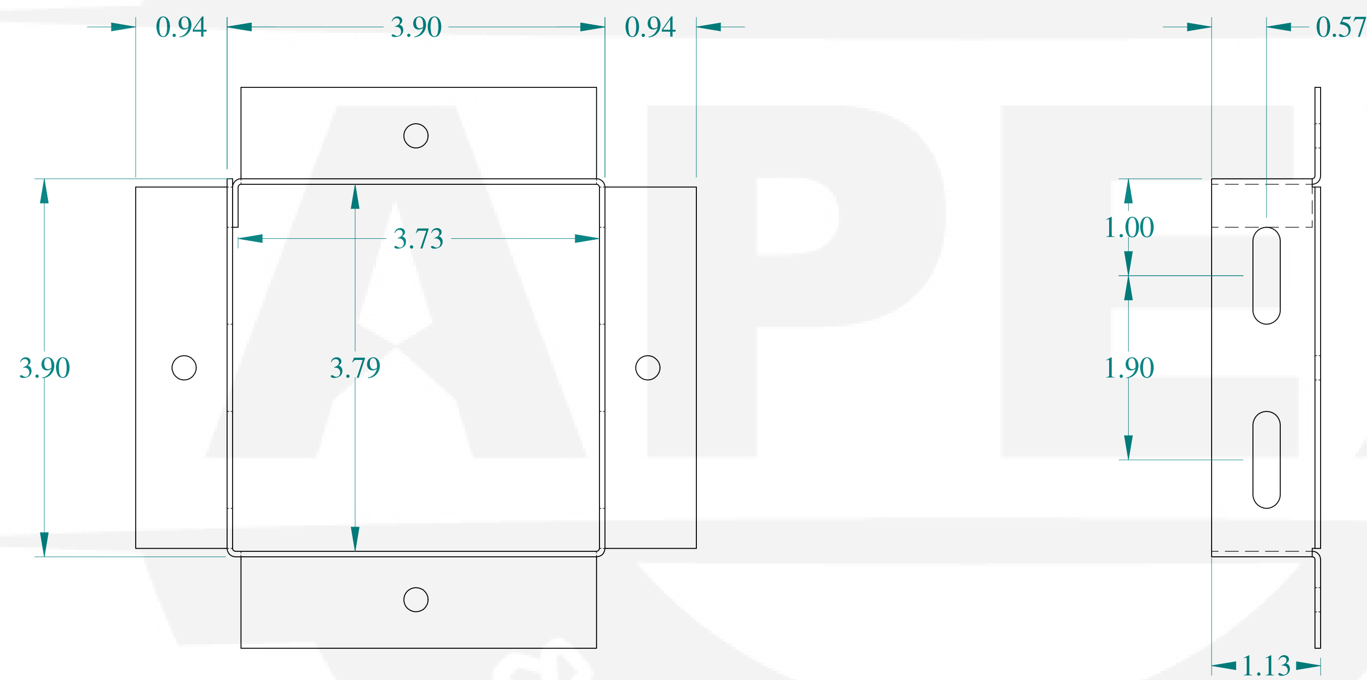
SIDE VIEW
