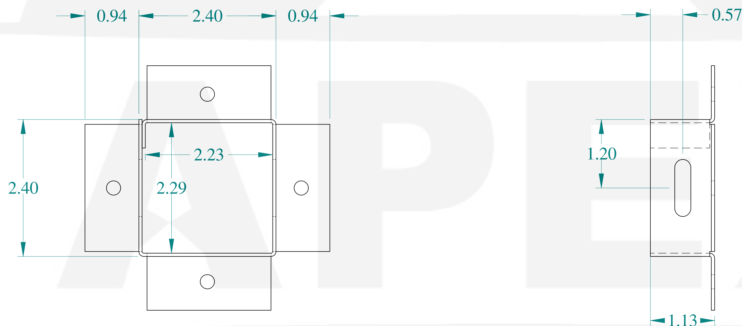
SIDE VIEW
