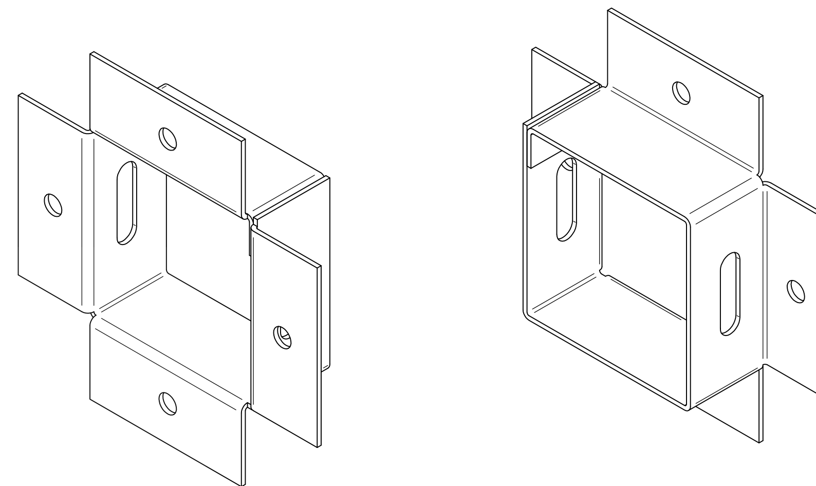
ISOMETRIC VIEWS
