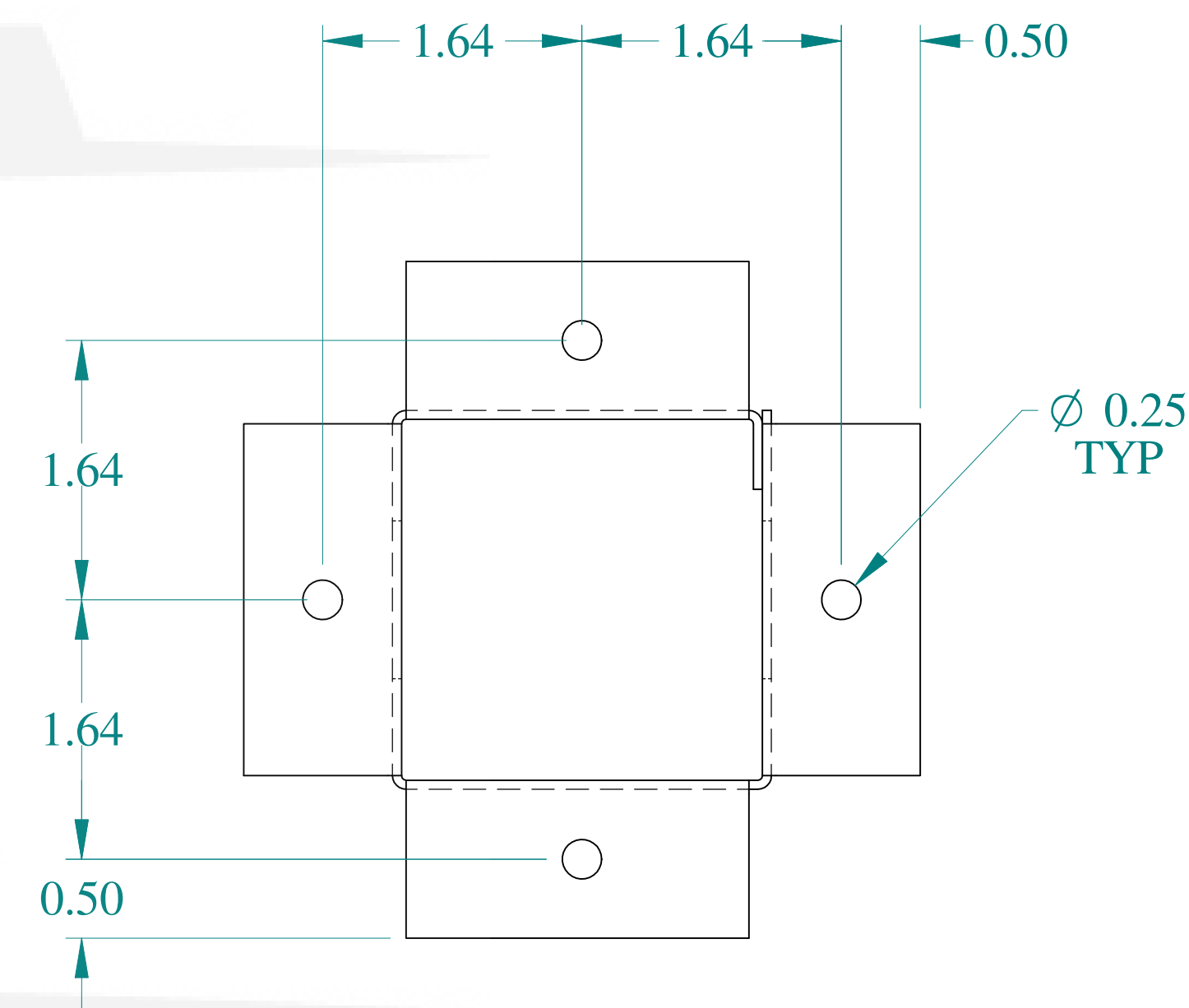
BACK VIEW
