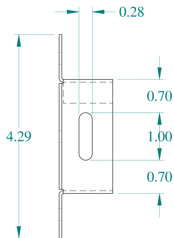
SIDE VIEW
