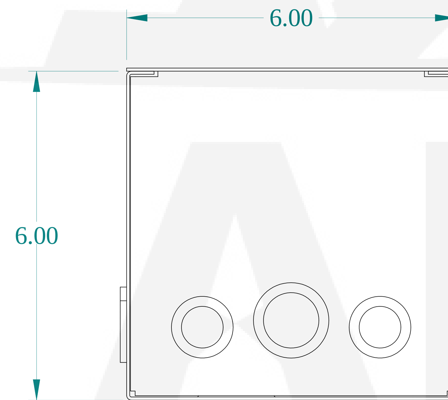
FRONT VIEW
