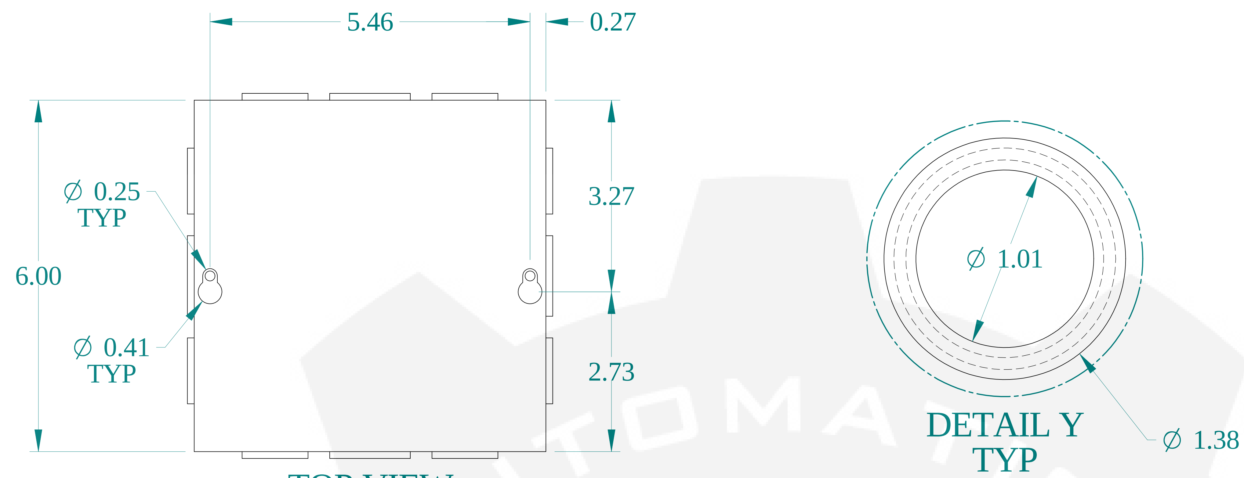
TOP VIEW
