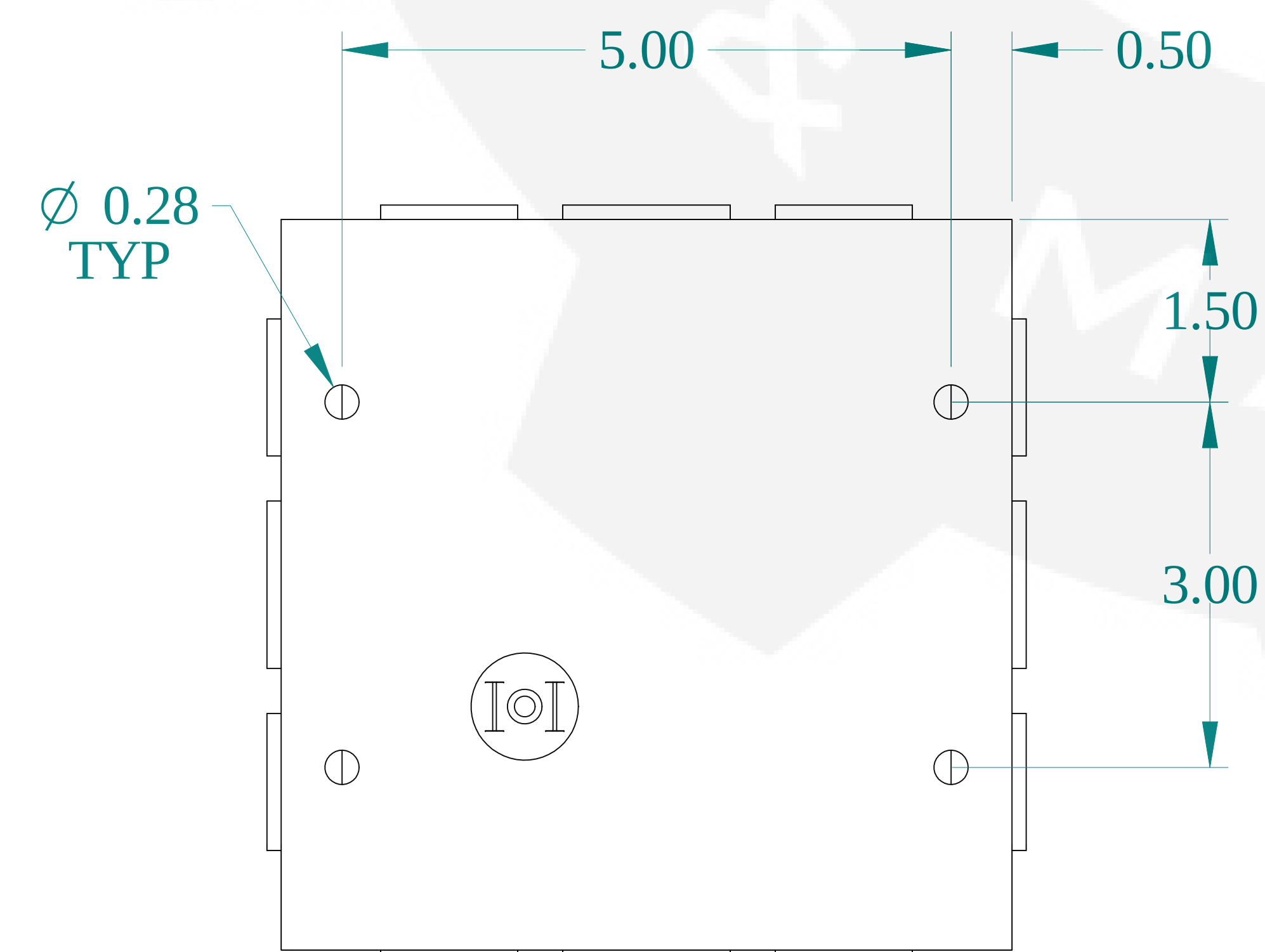
BOTTOM VIEW
