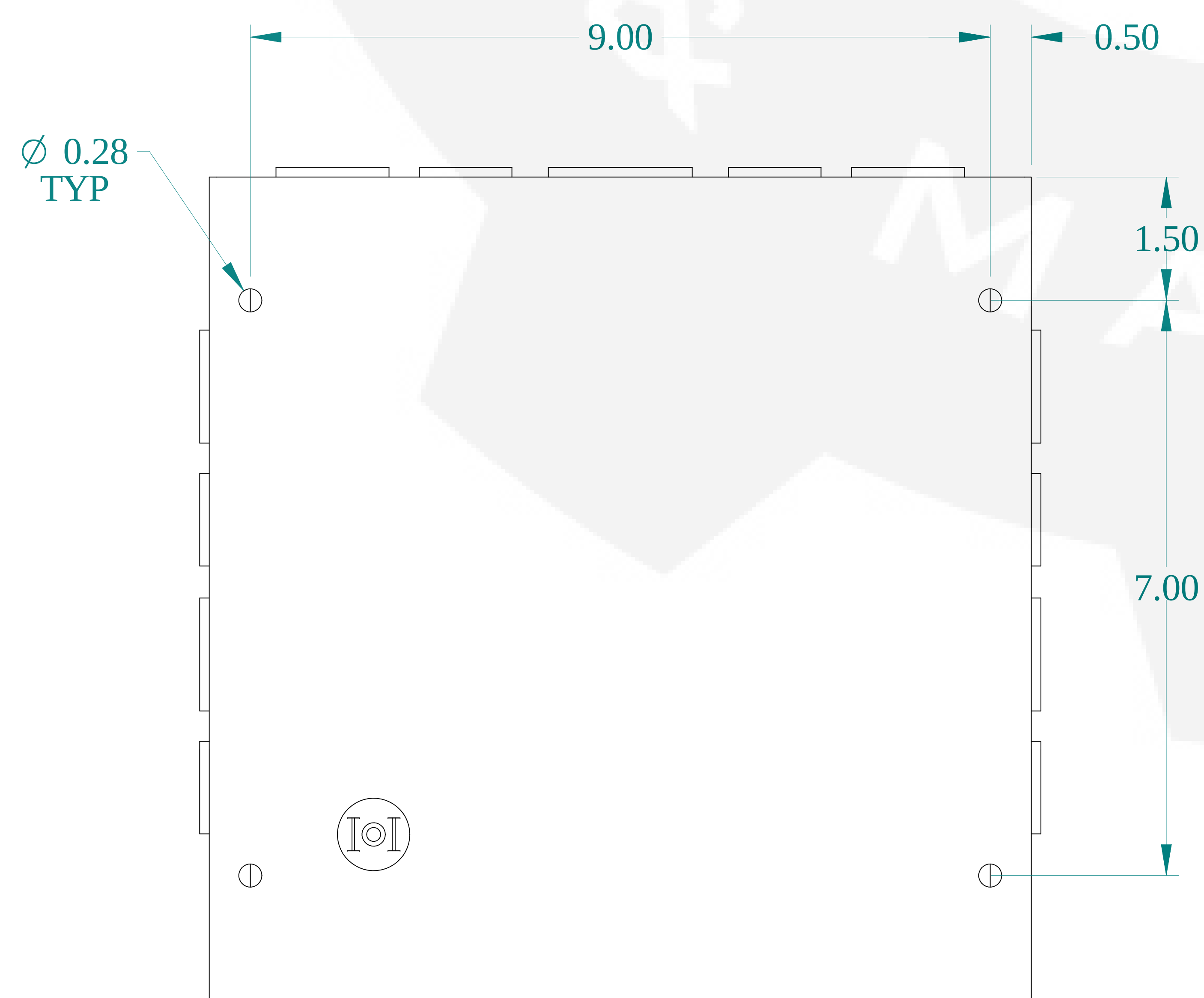
BOTTOM VIEW
