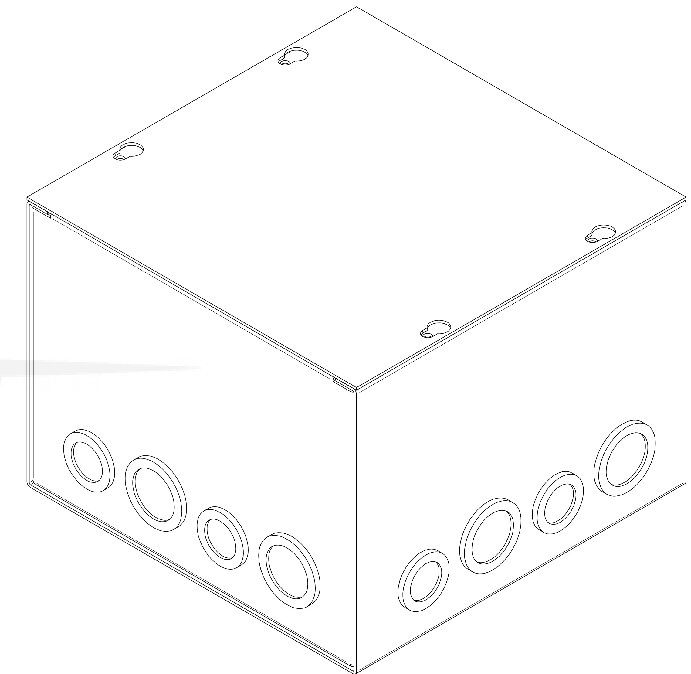
ISOMETRIC VIEWS
