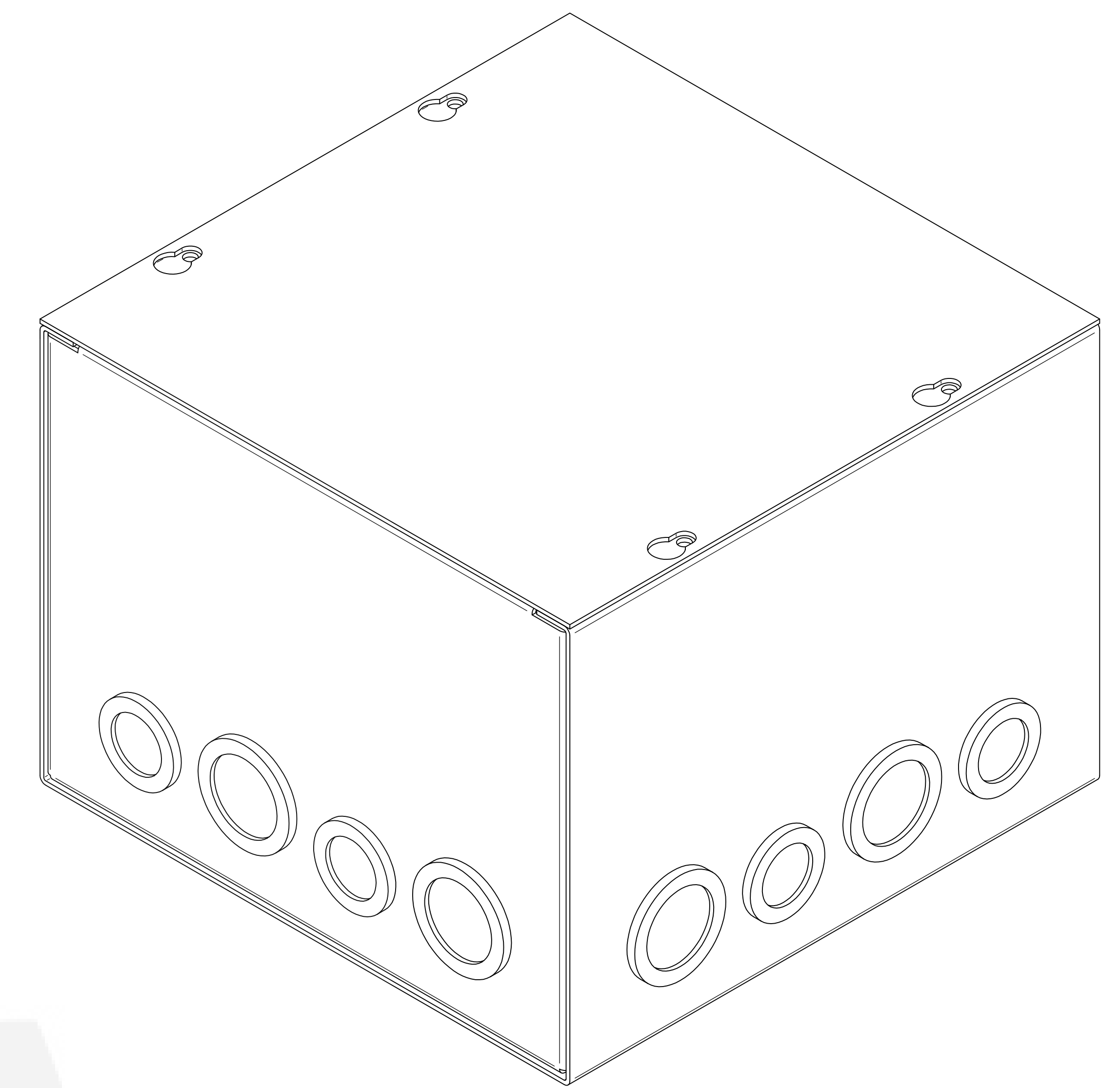
ISOMETRIC VIEWS
