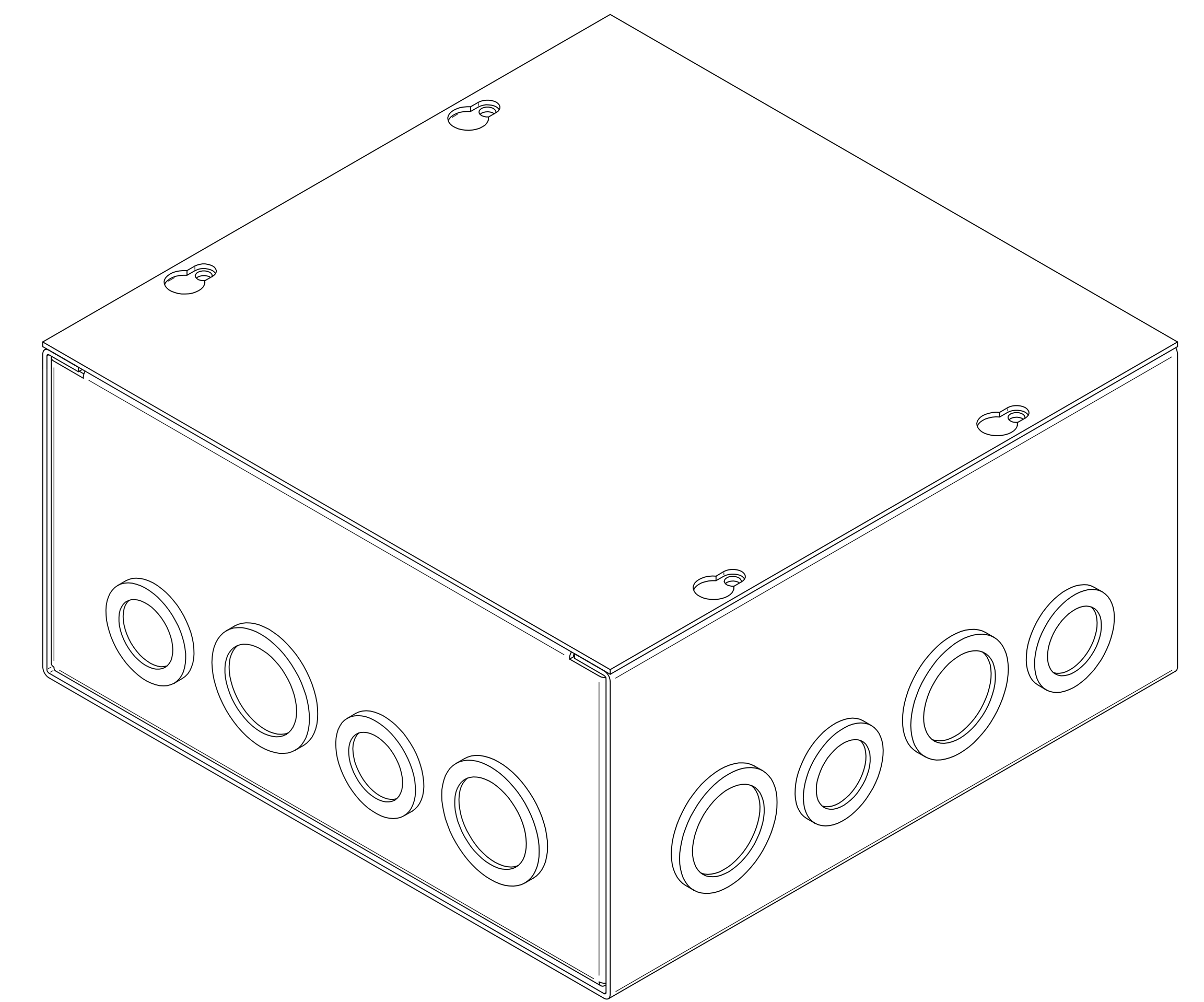
ISOMETRIC VIEWS
