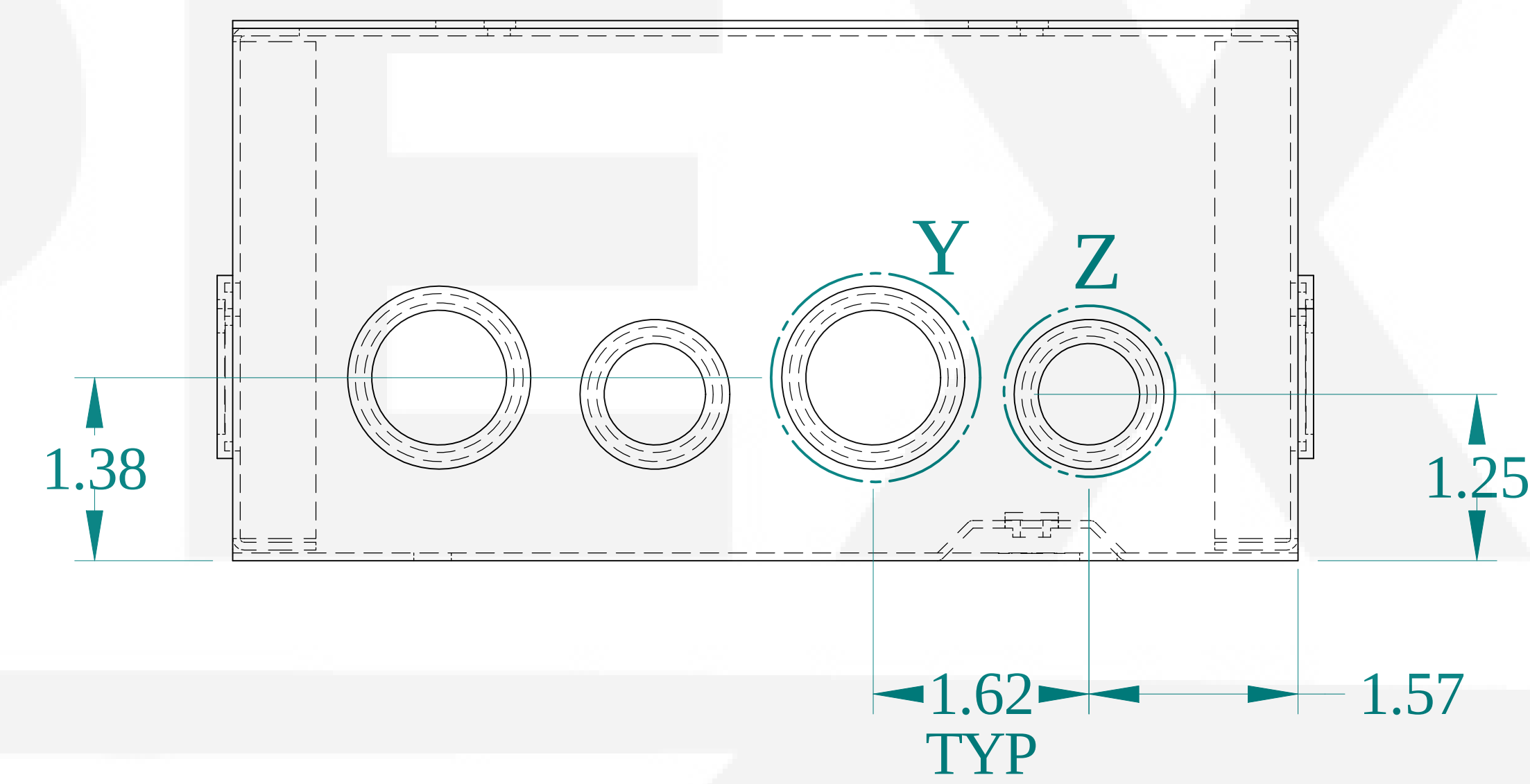
SIDE VIEW
