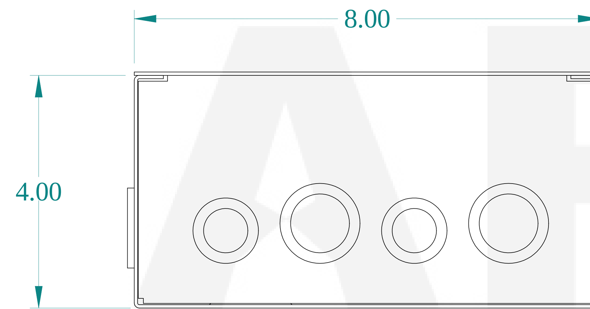
FRONT VIEW
