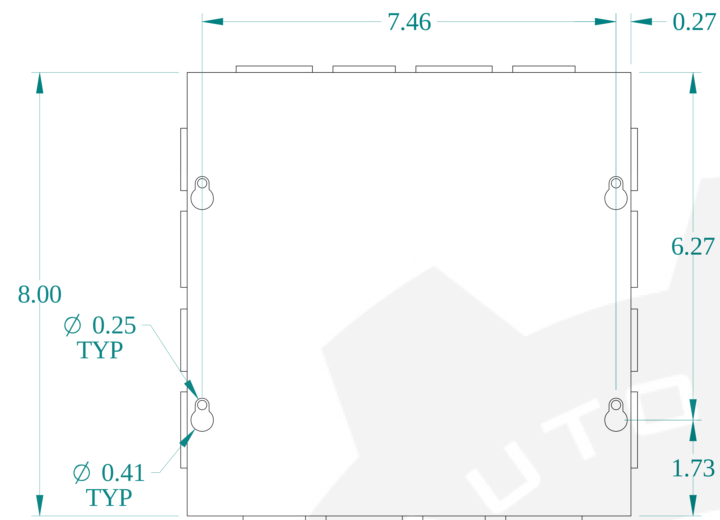
TOP VIEW
