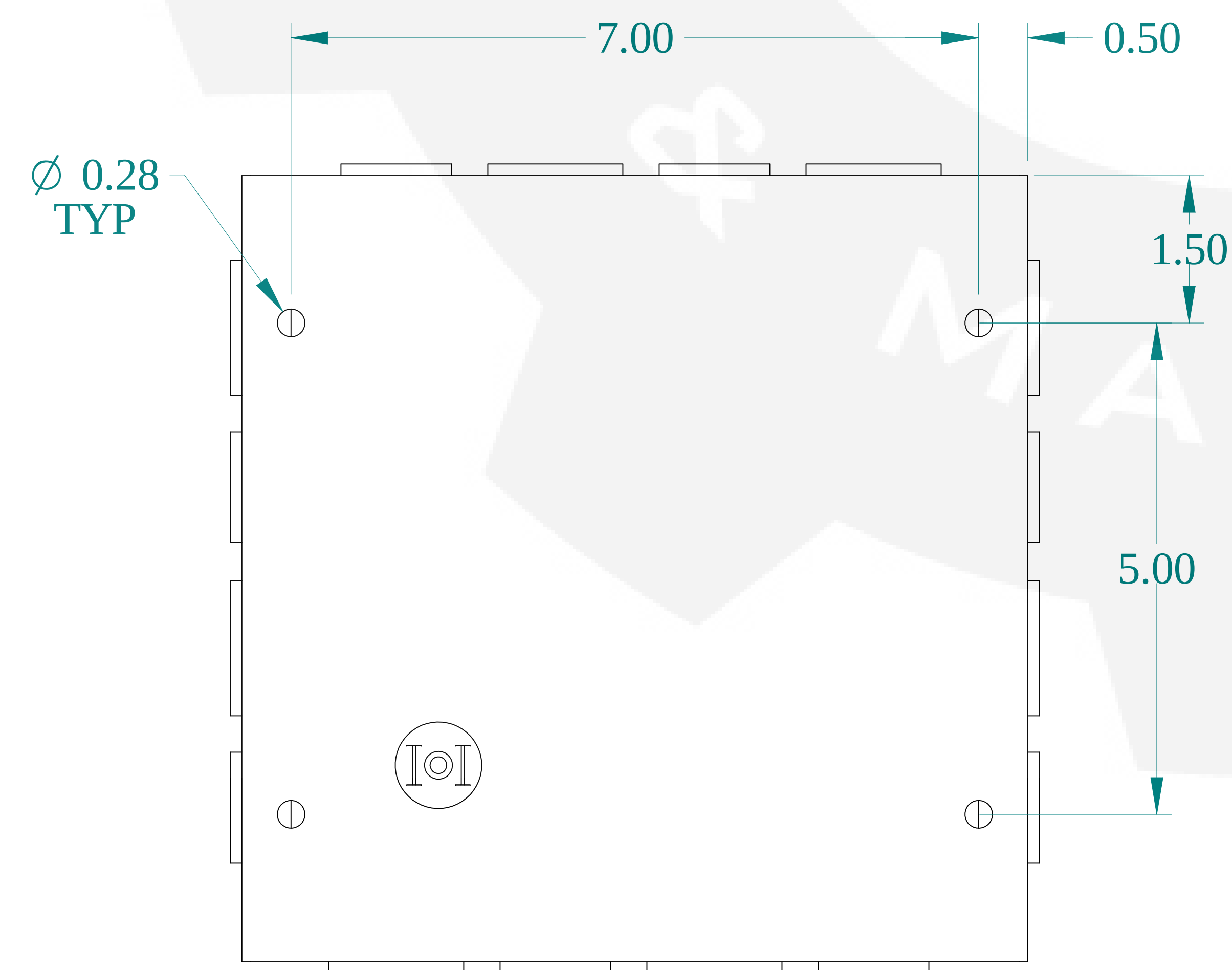
BOTTOM VIEW
