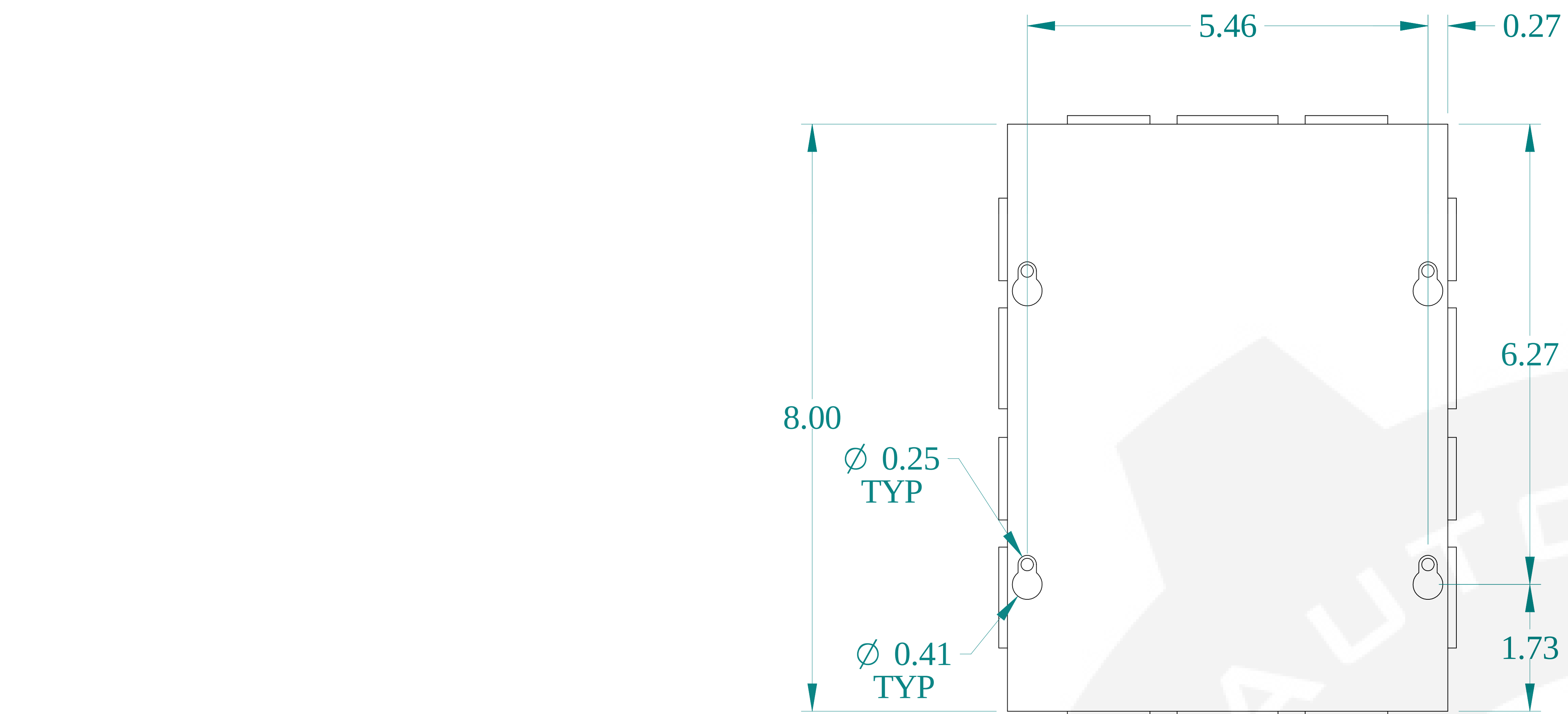
TOP VIEW
