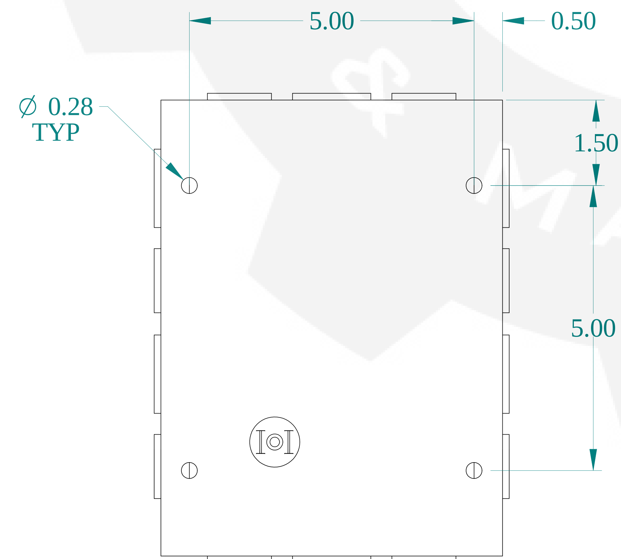
BOTTOM VIEW
