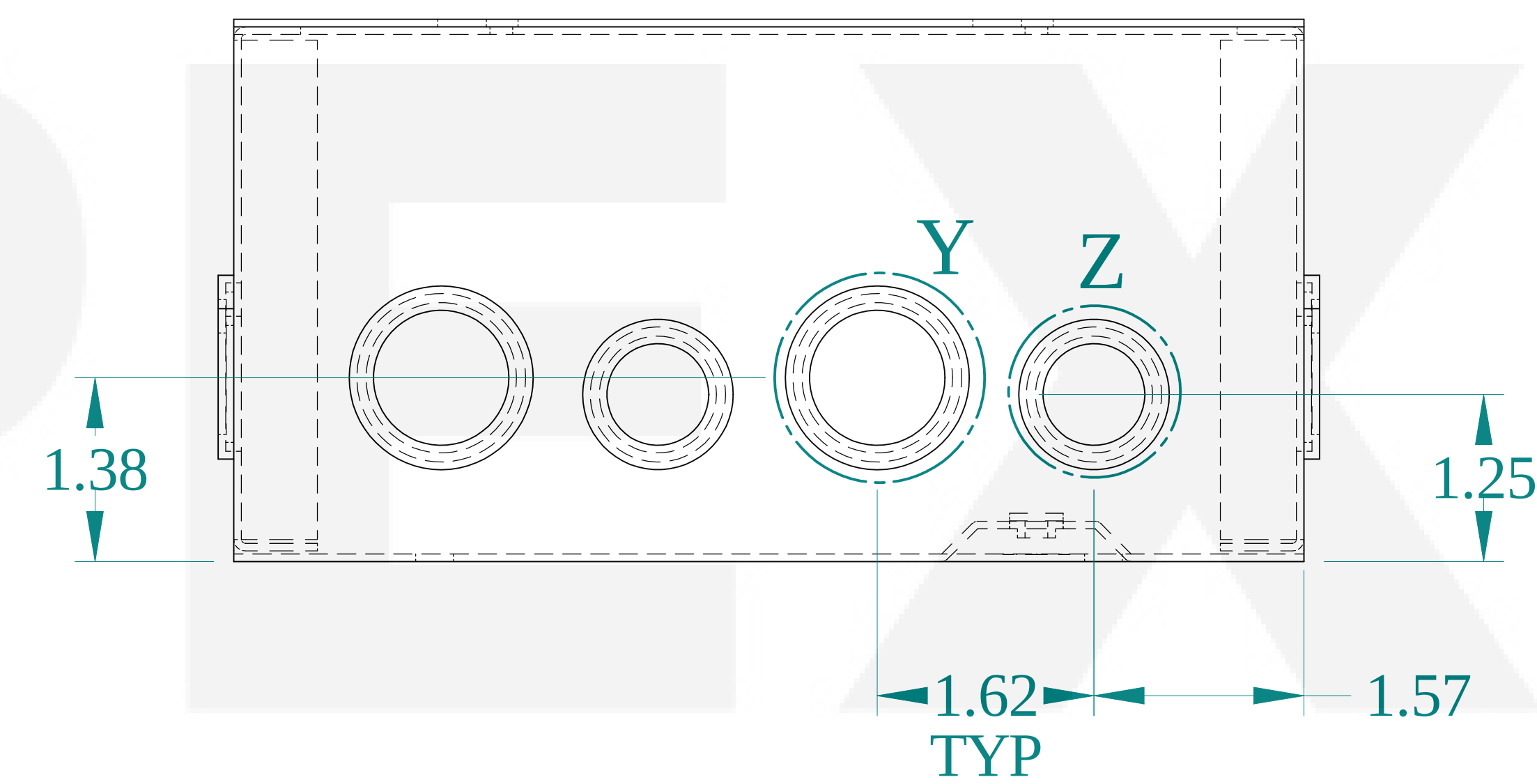
SIDE VIEW
