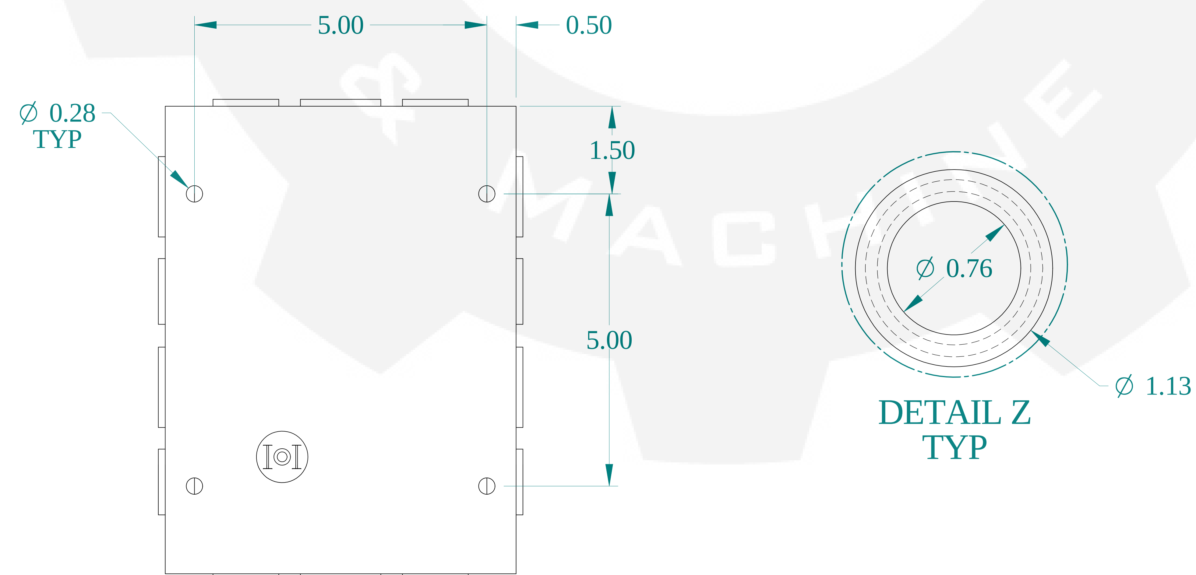
BOTTOM VIEW
