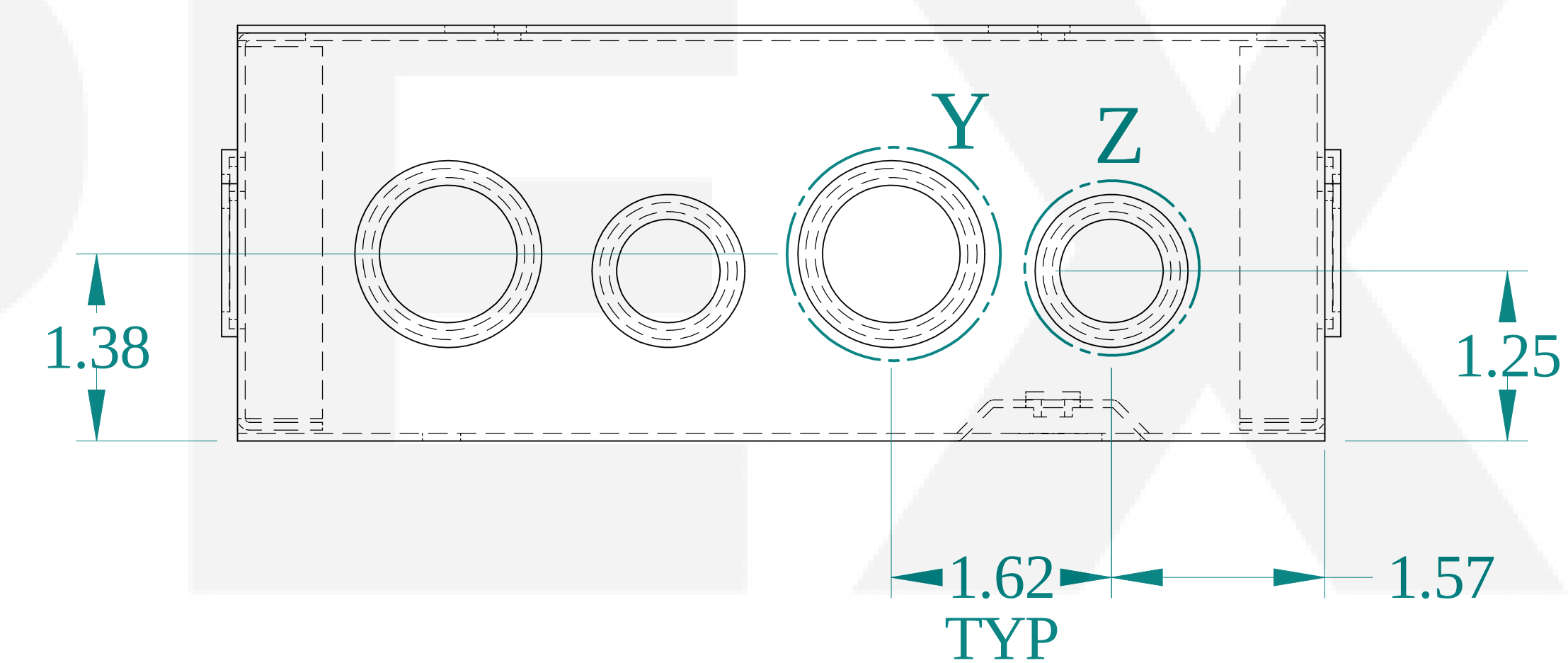
SIDE VIEW
