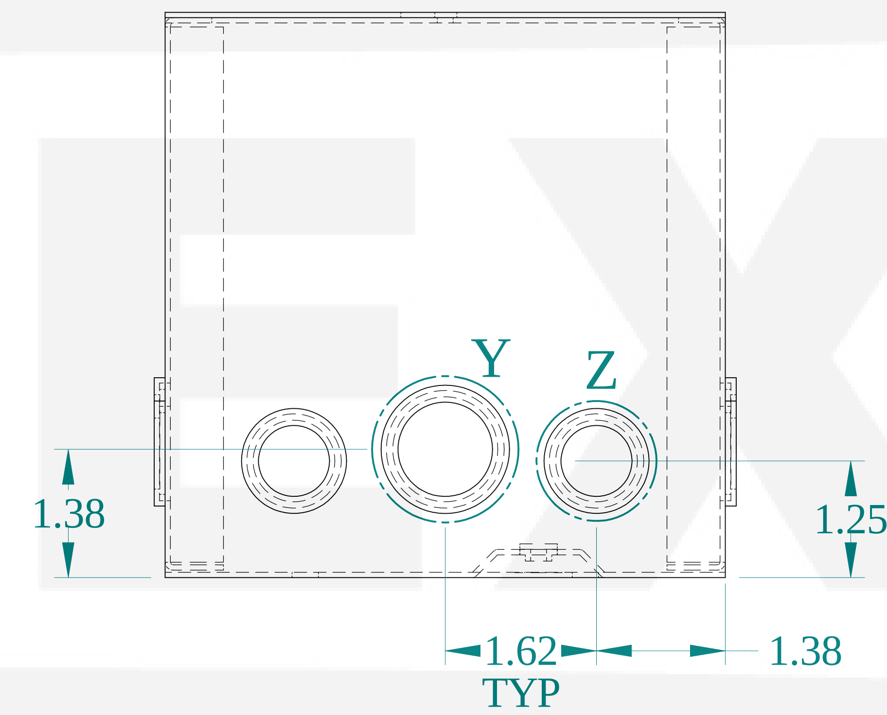
SIDE VIEW
