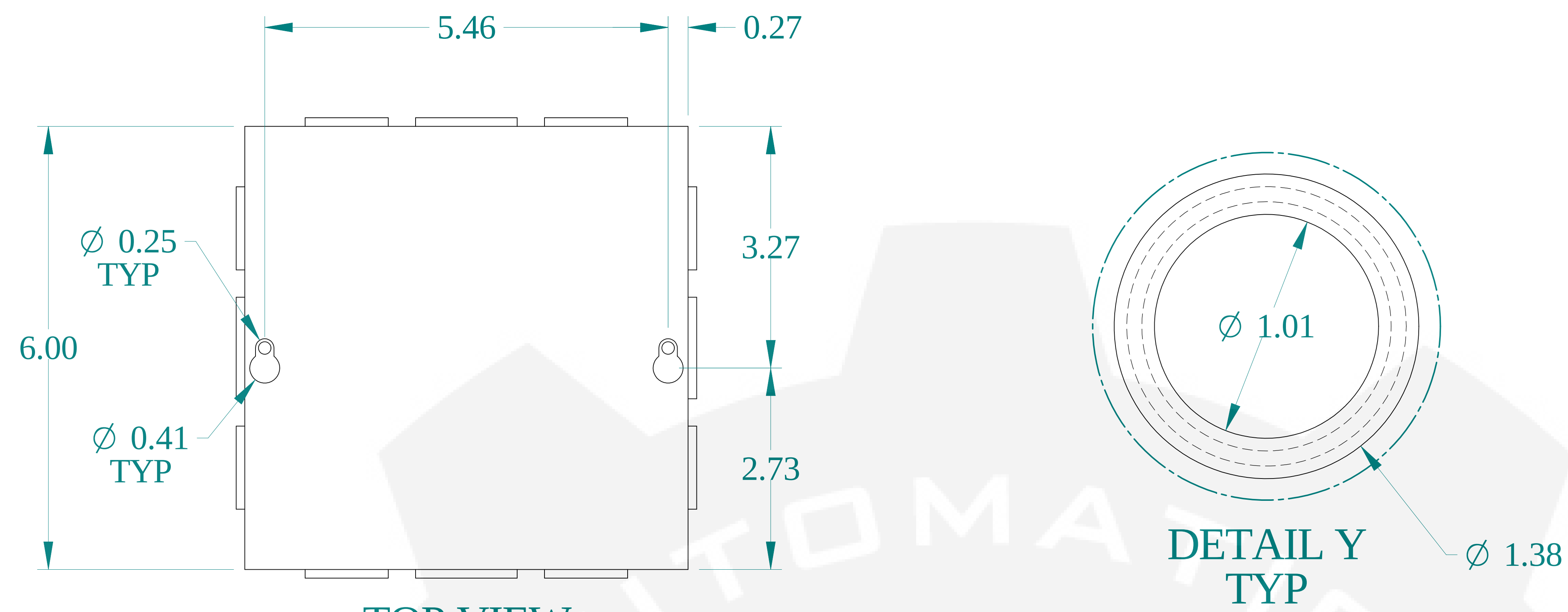
TOP VIEW
