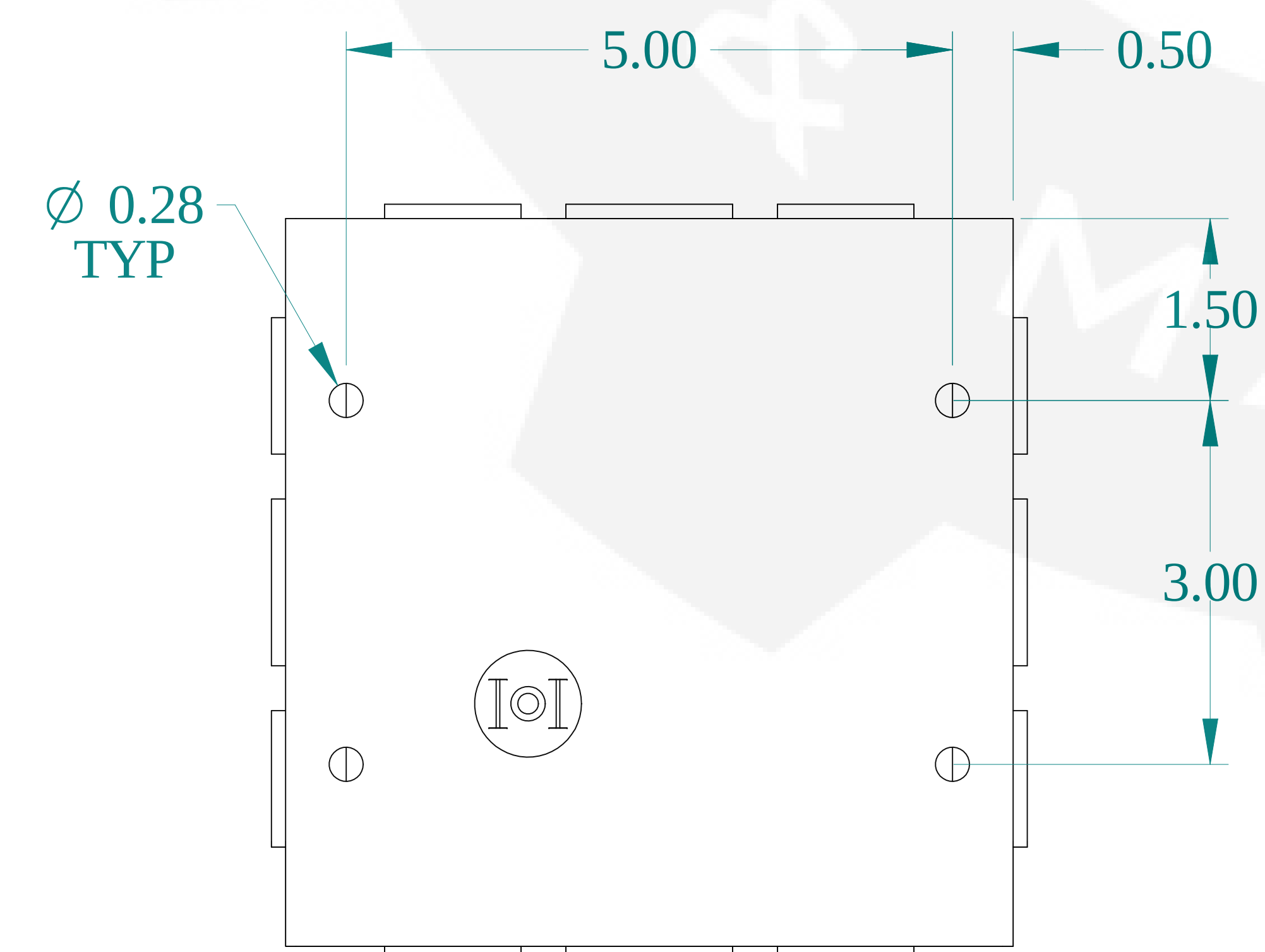
BOTTOM VIEW
