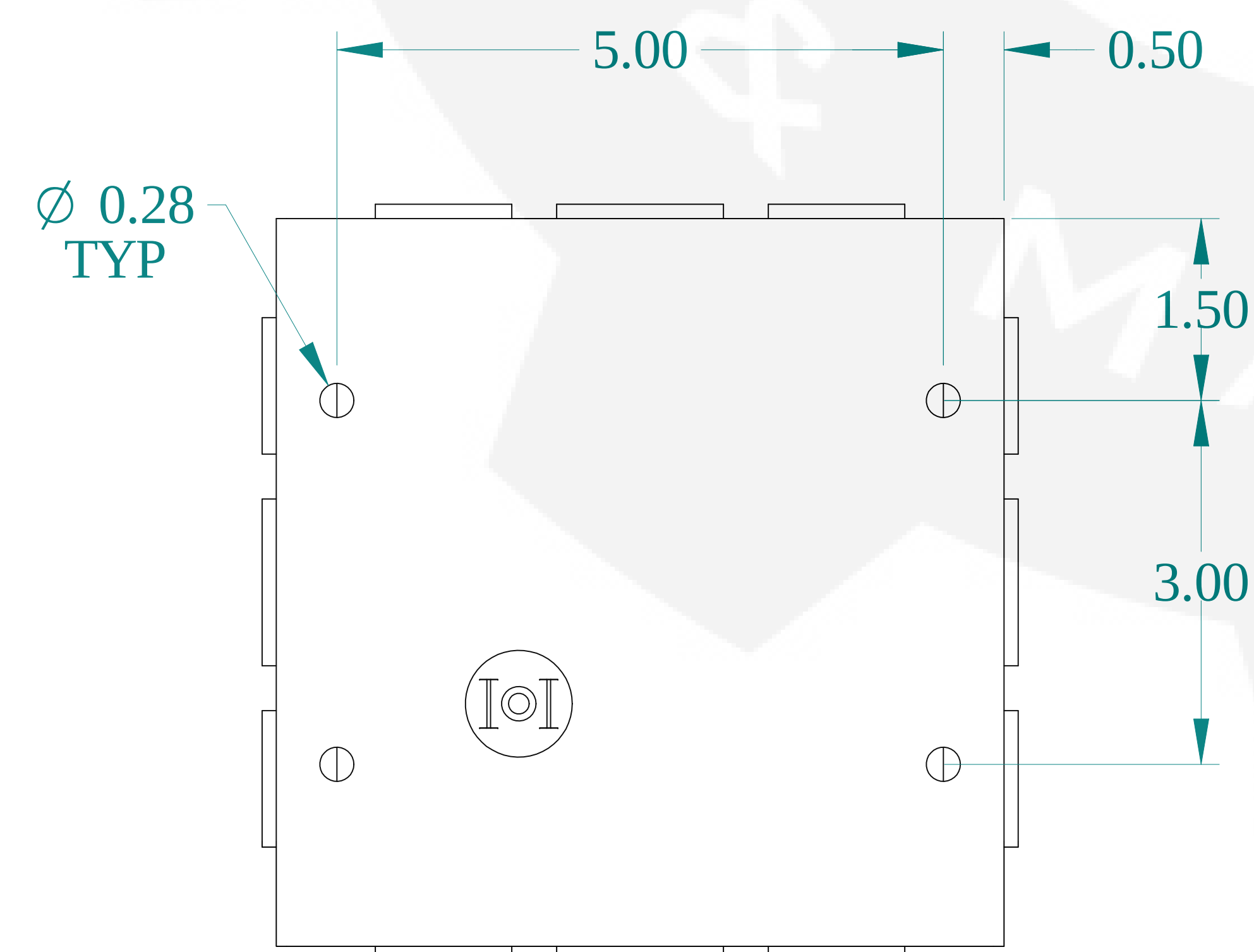
BOTTOM VIEW
