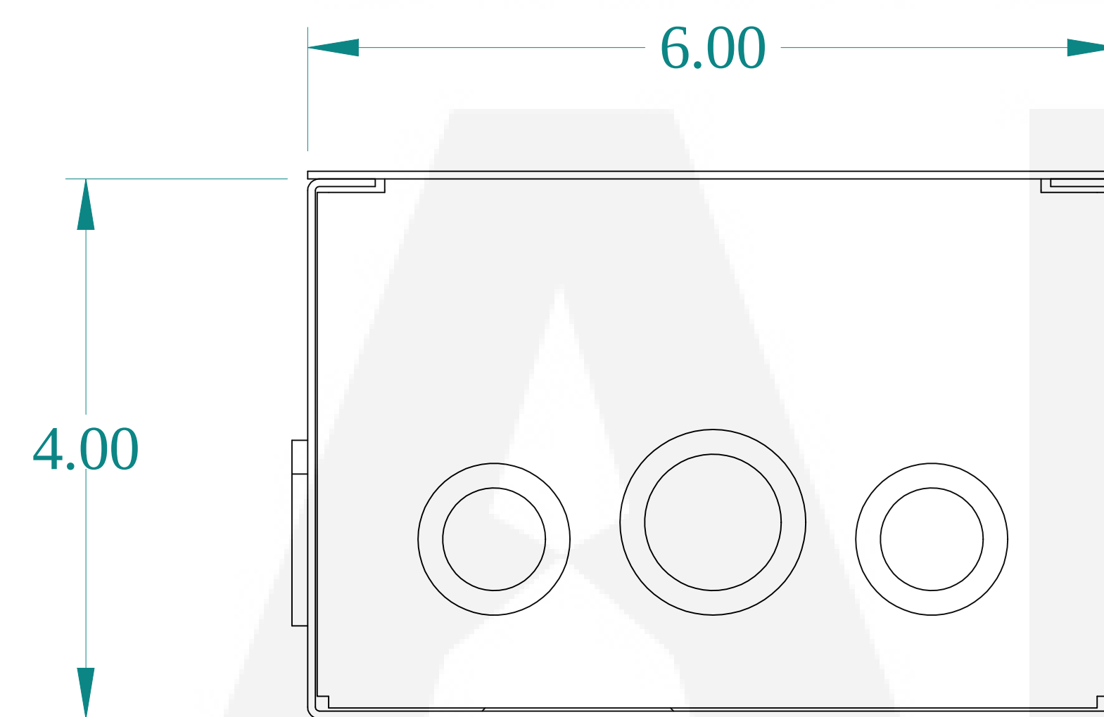
FRONT VIEW
