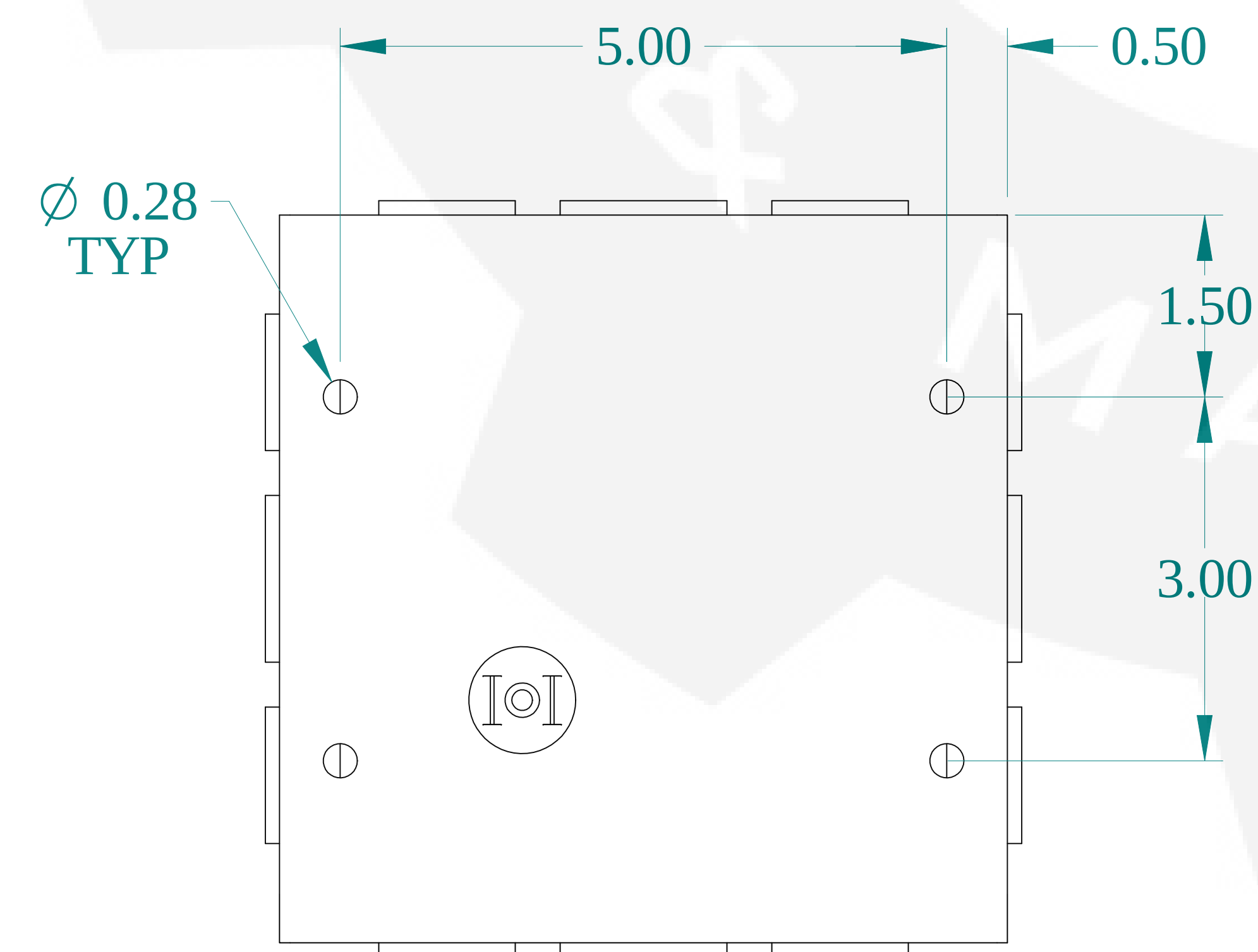
BOTTOM VIEW
