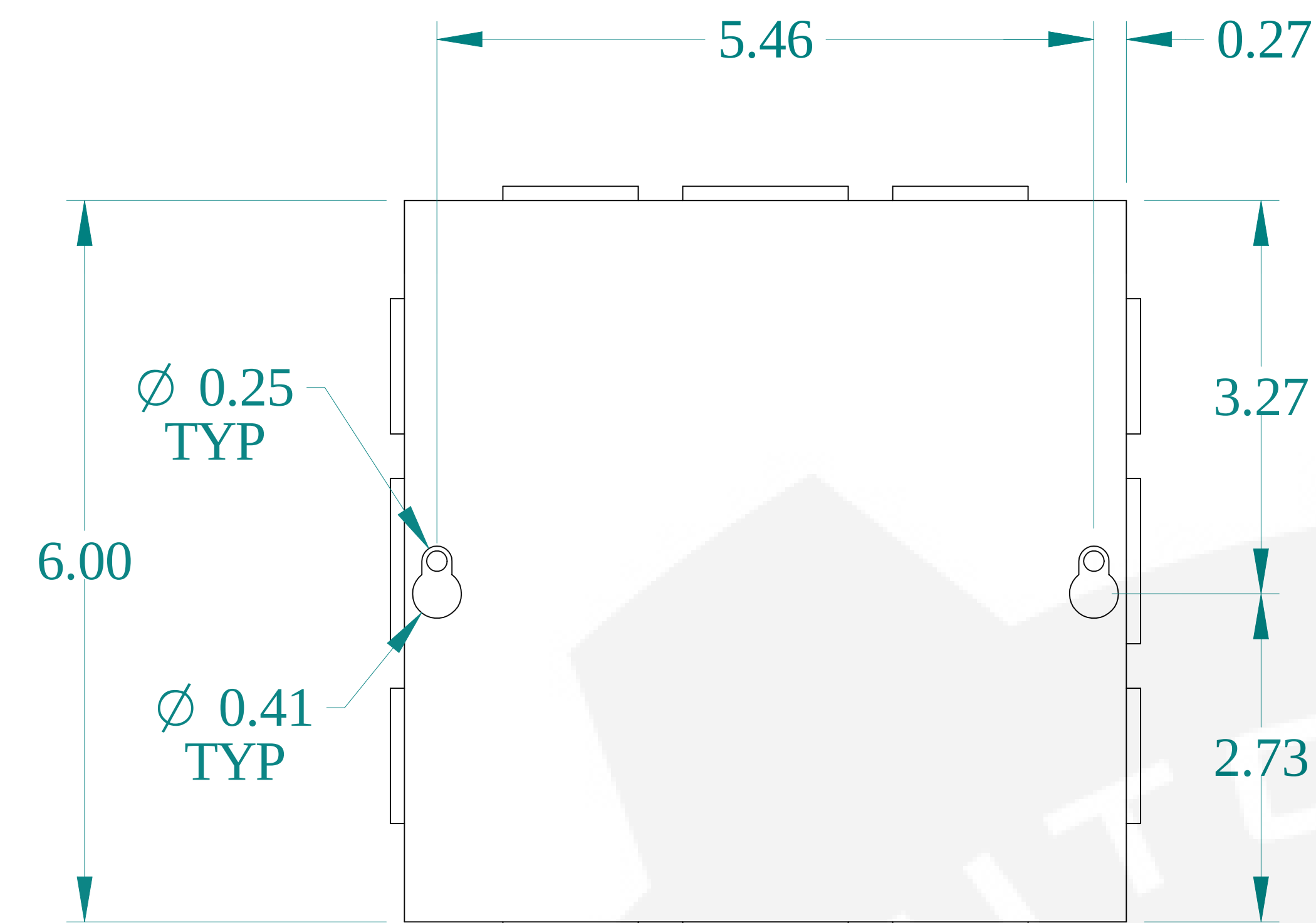
TOP VIEW
