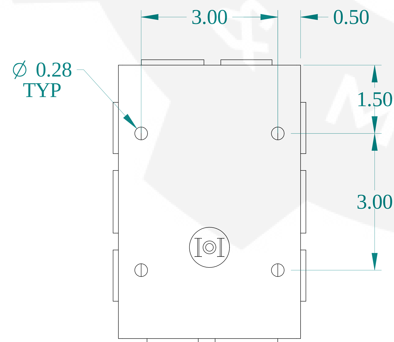
BOTTOM VIEW
