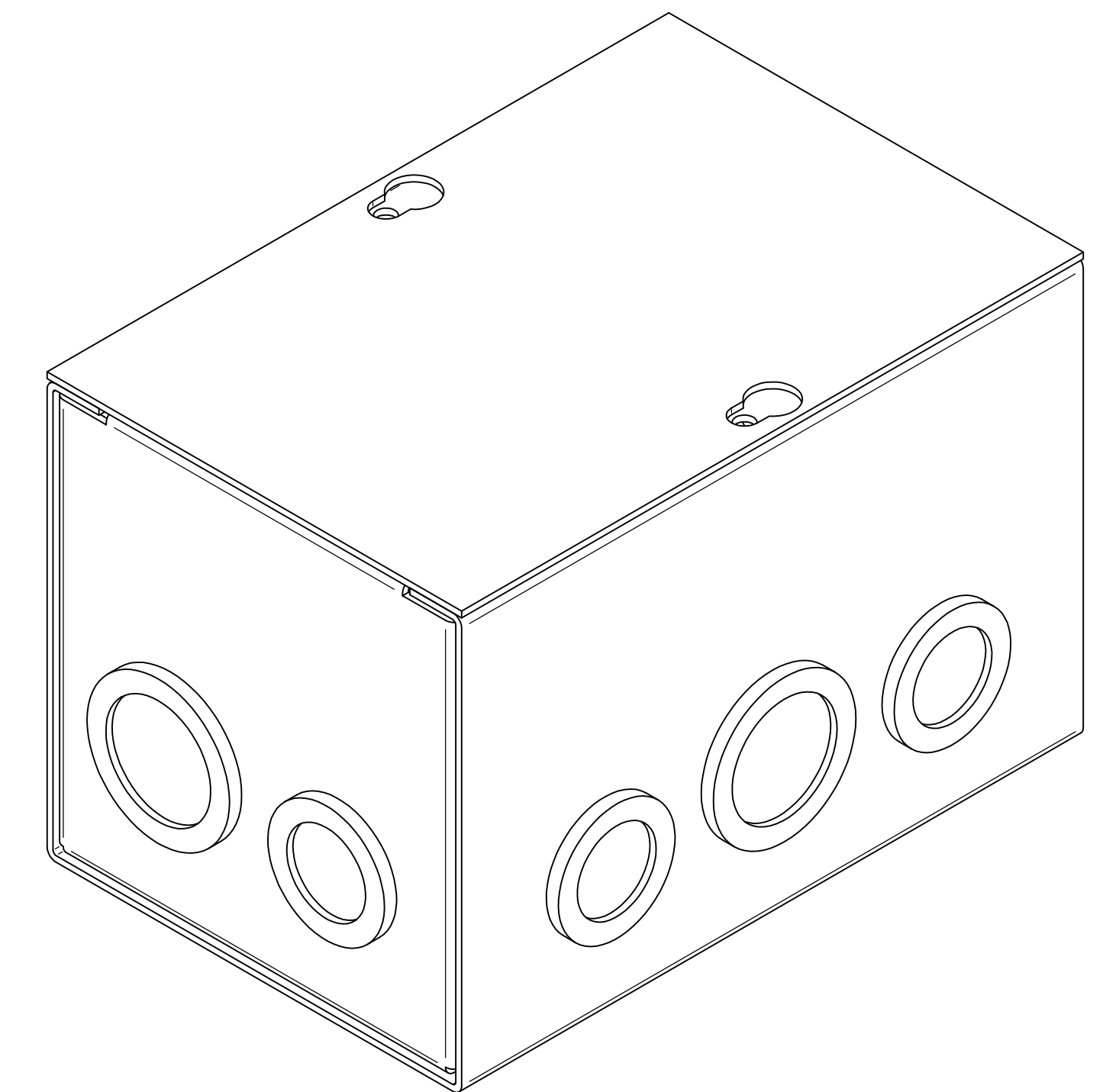
ISOMETRIC VIEWS
