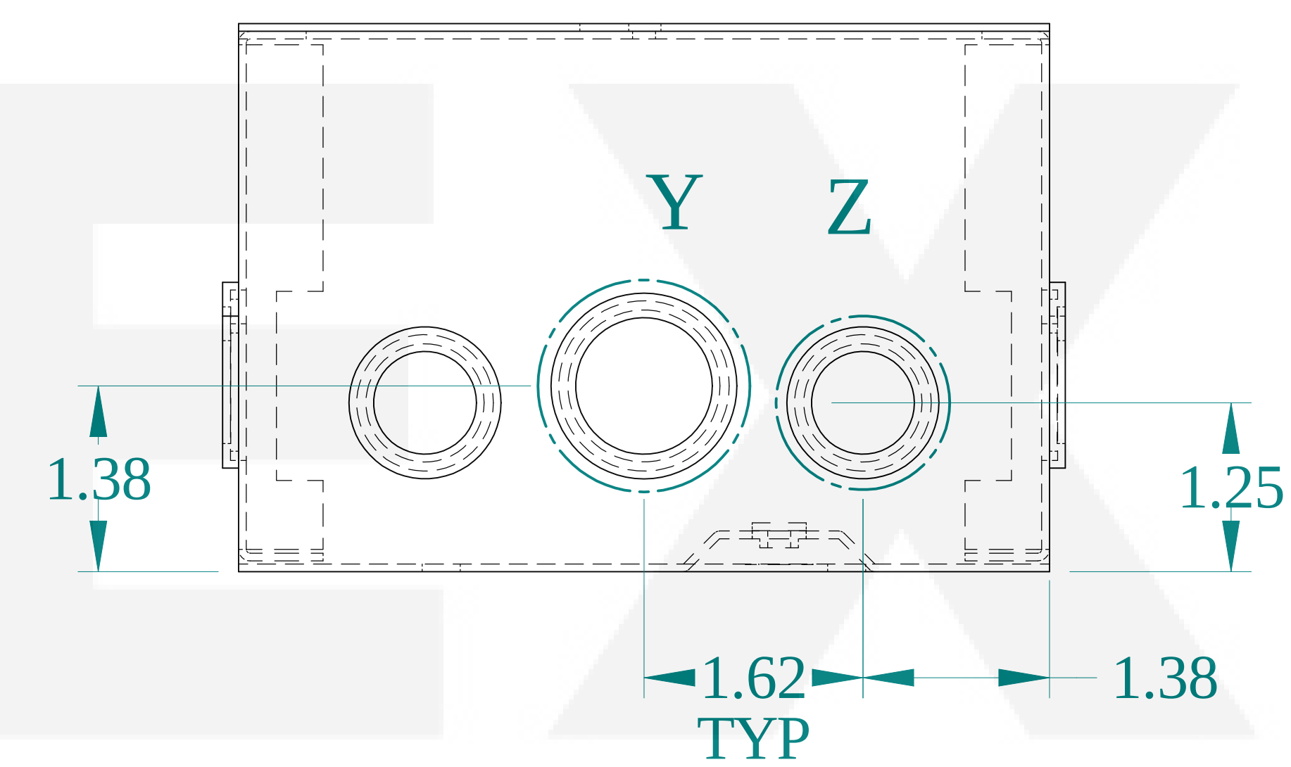
SIDE VIEW
