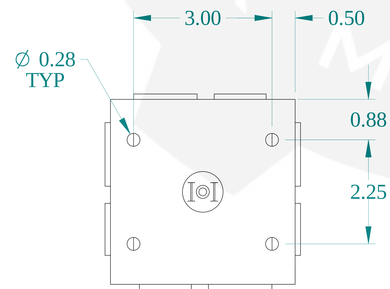
BOTTOM VIEW
