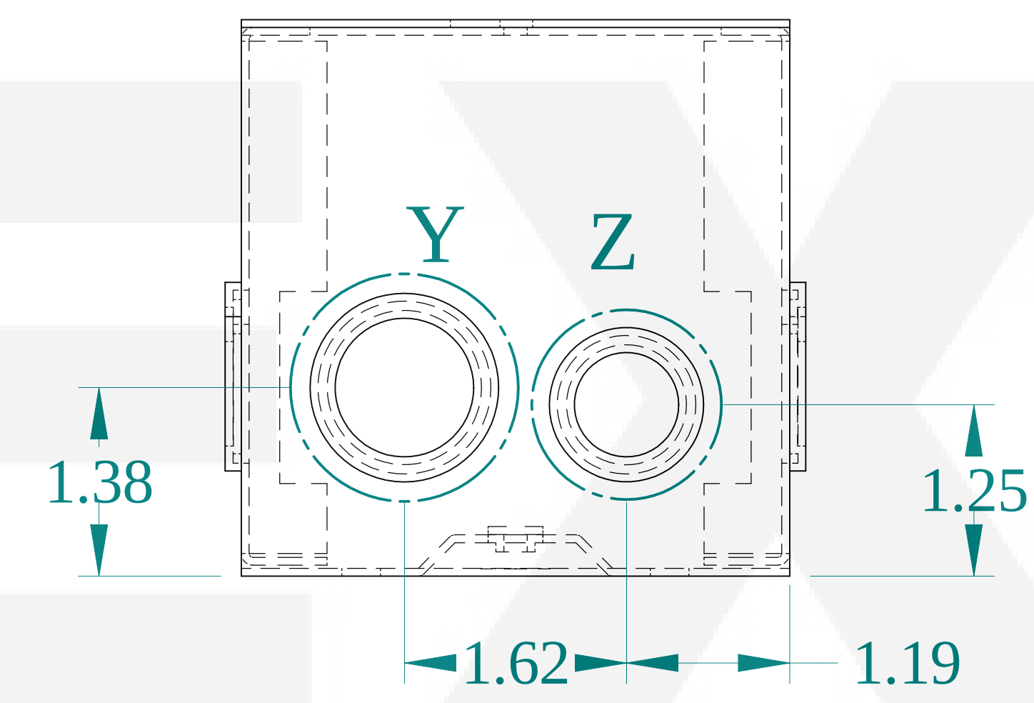
SIDE VIEW
