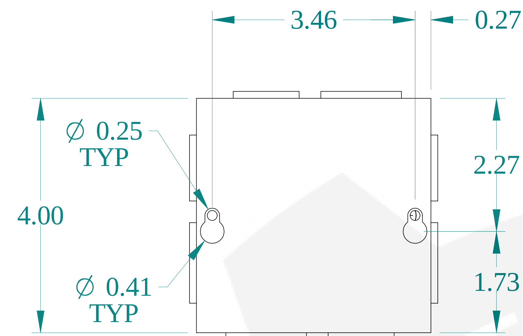
TOP VIEW
