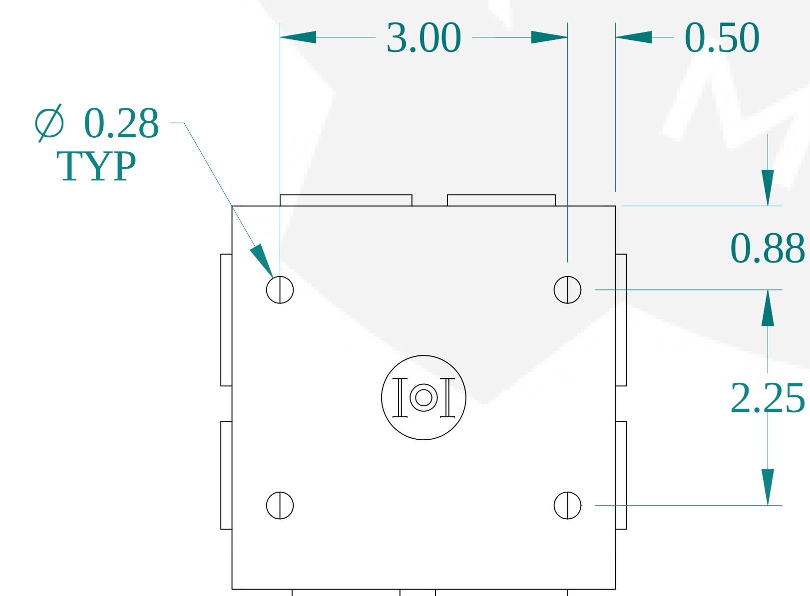
BOTTOM VIEW
