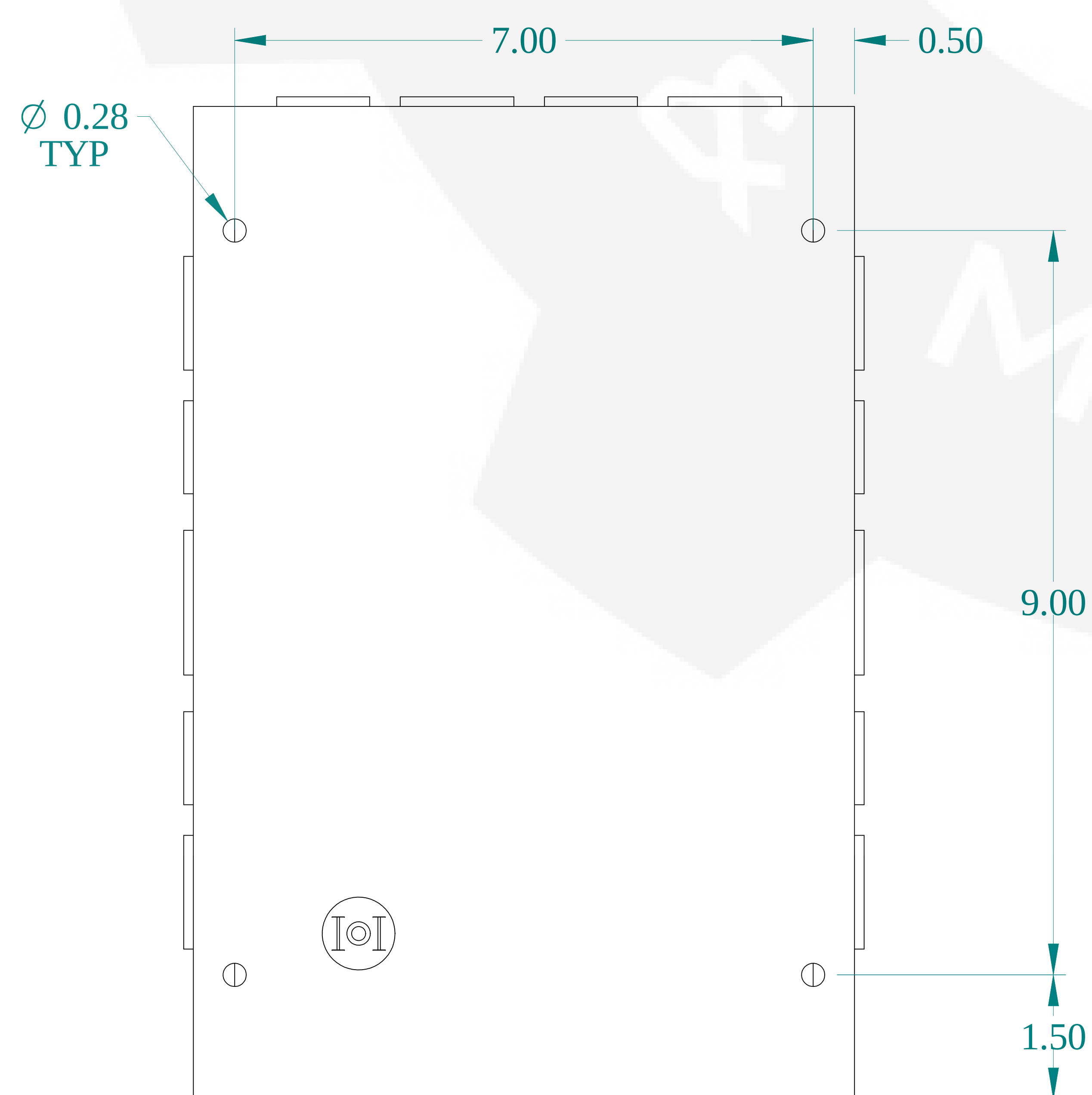
BOTTOM VIEW
