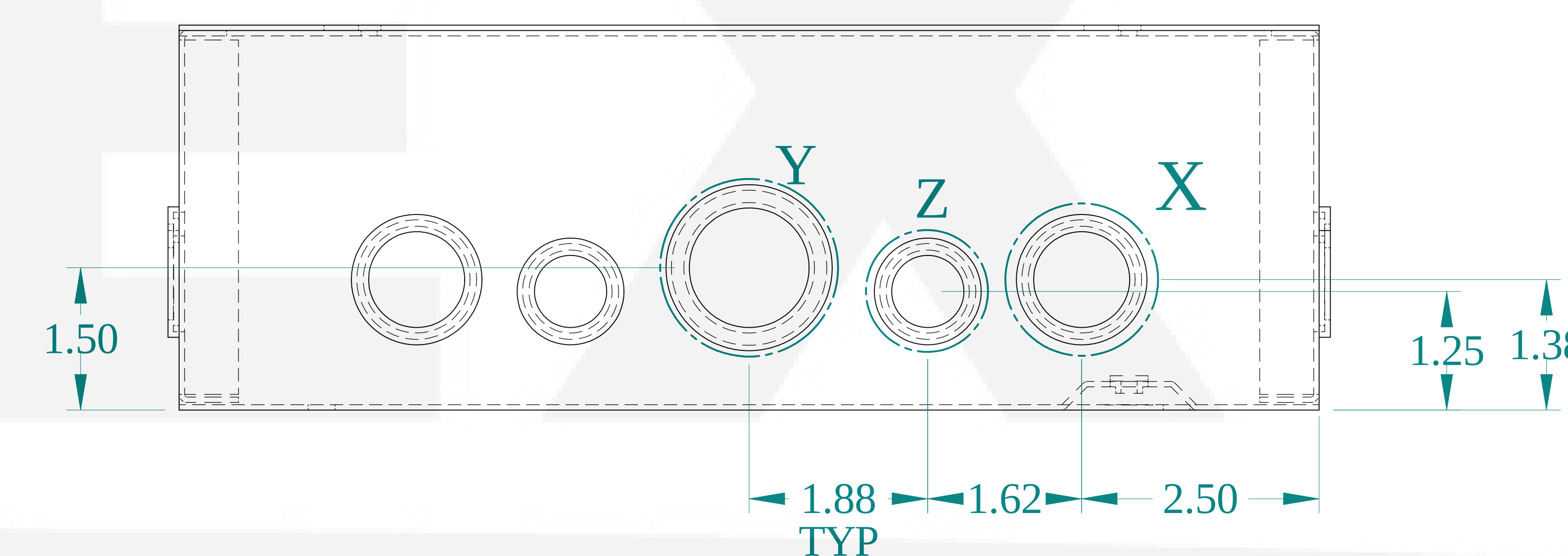
SIDE VIEW
