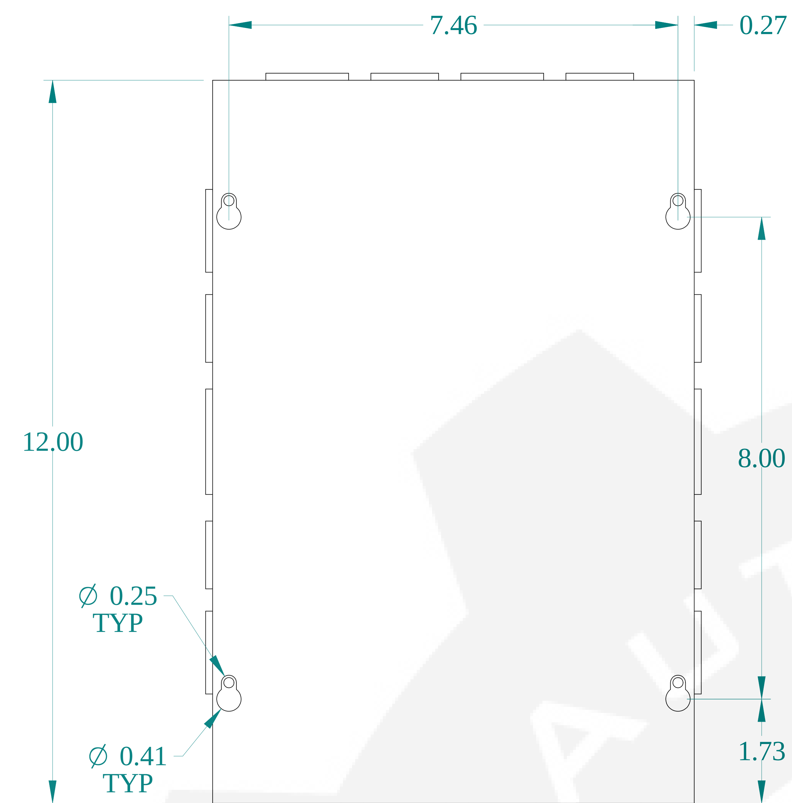
TOP VIEW
