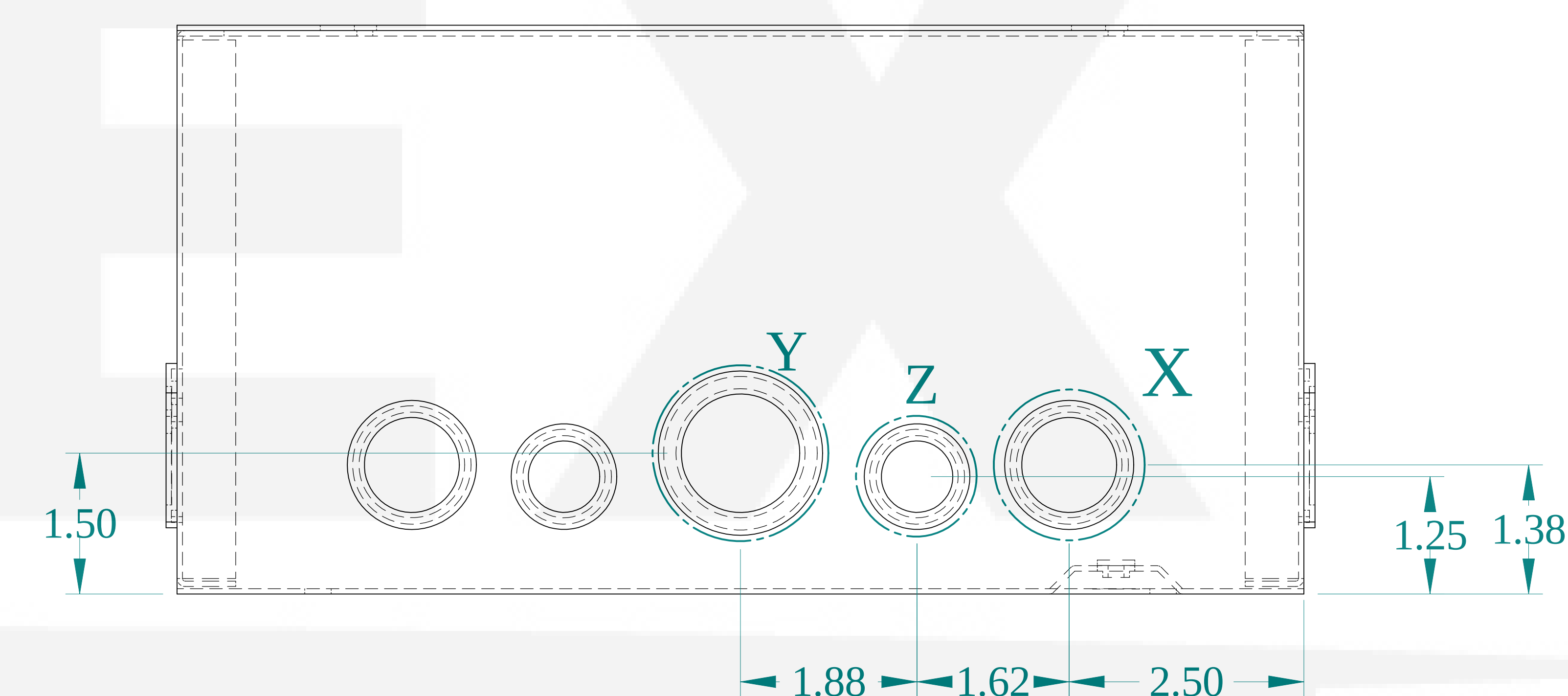
SIDE VIEW
