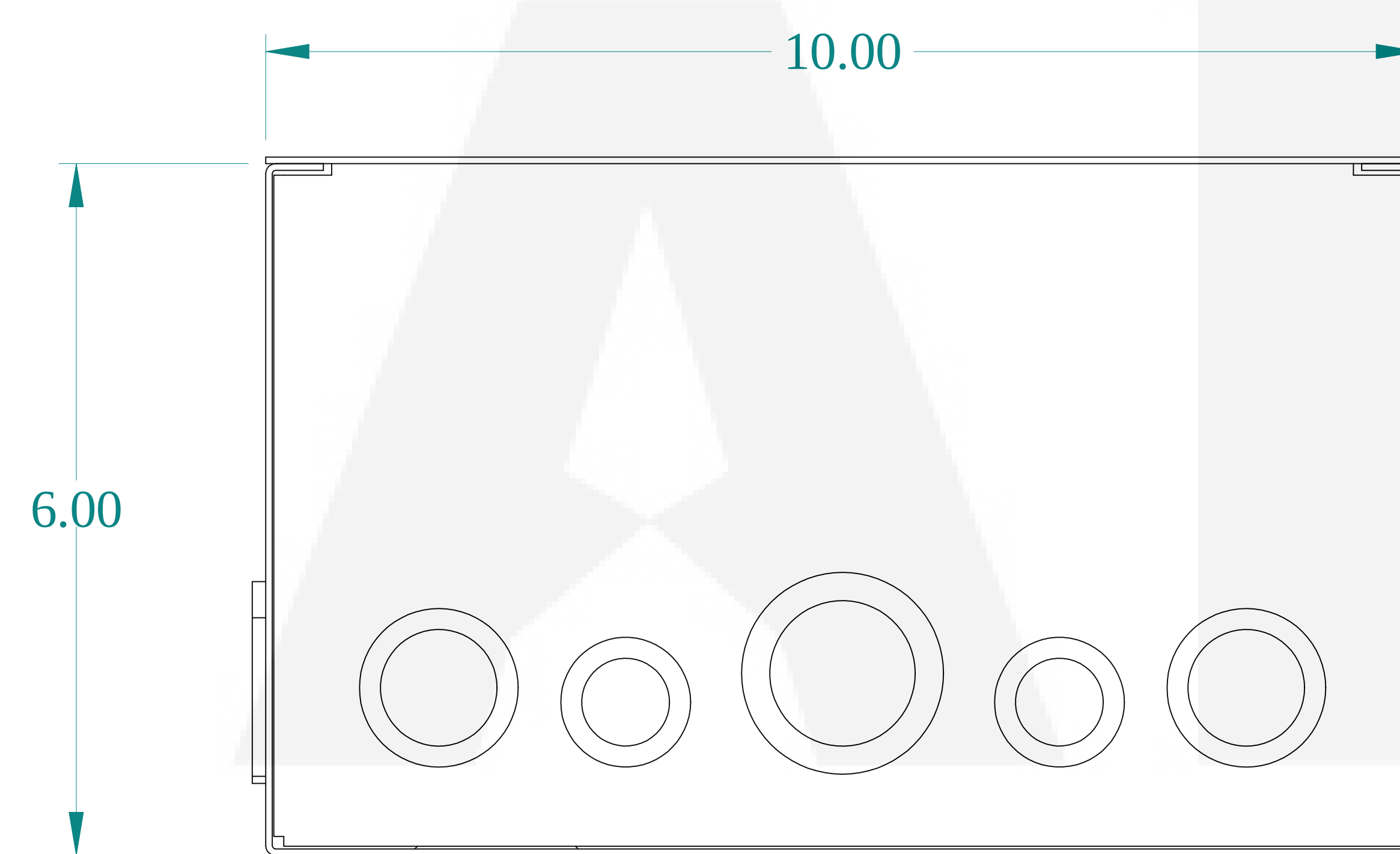
FRONT VIEW
