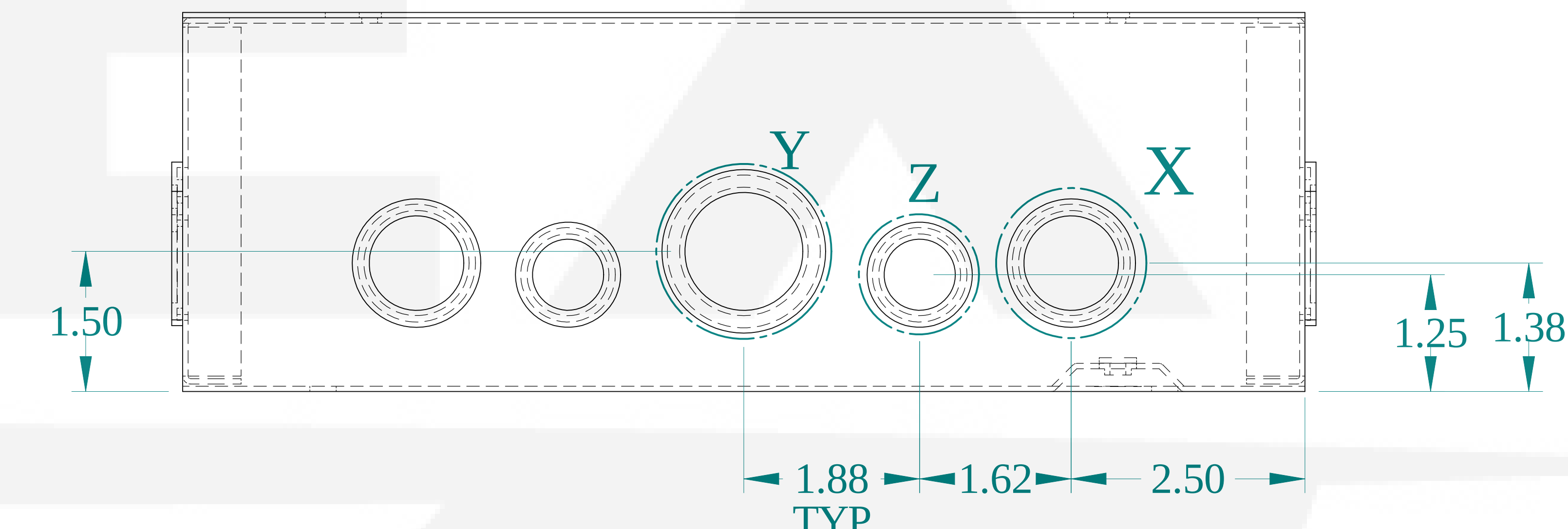
SIDE VIEW
