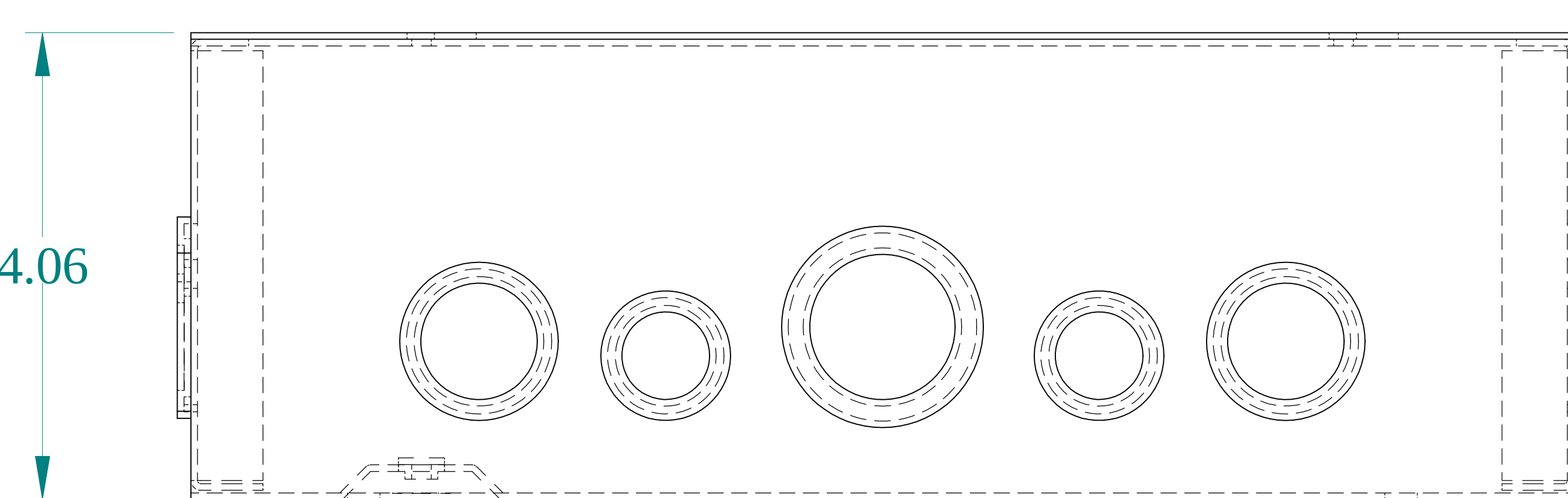
SIDE VIEW
