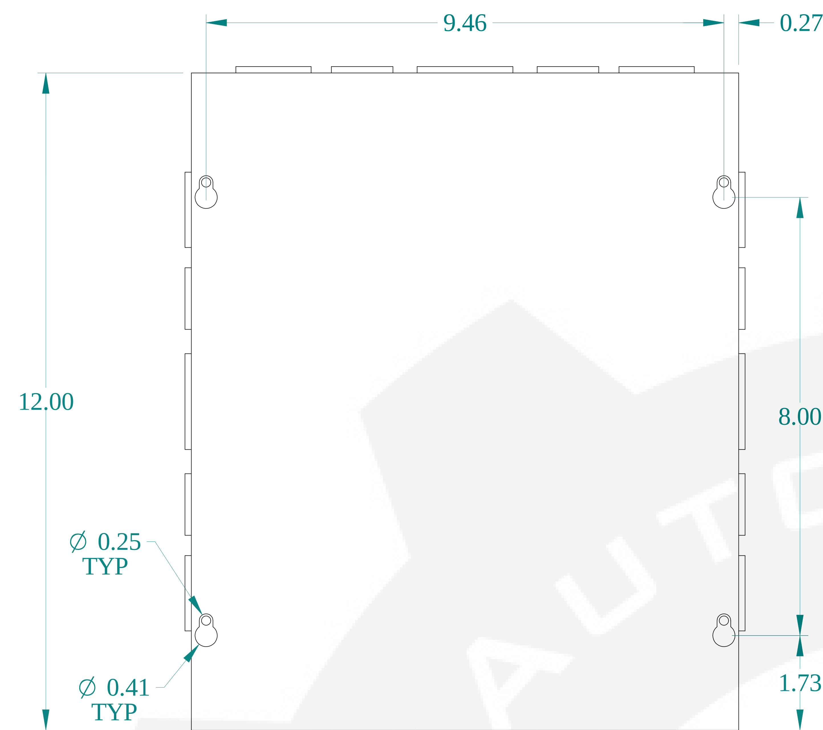
TOP VIEW
