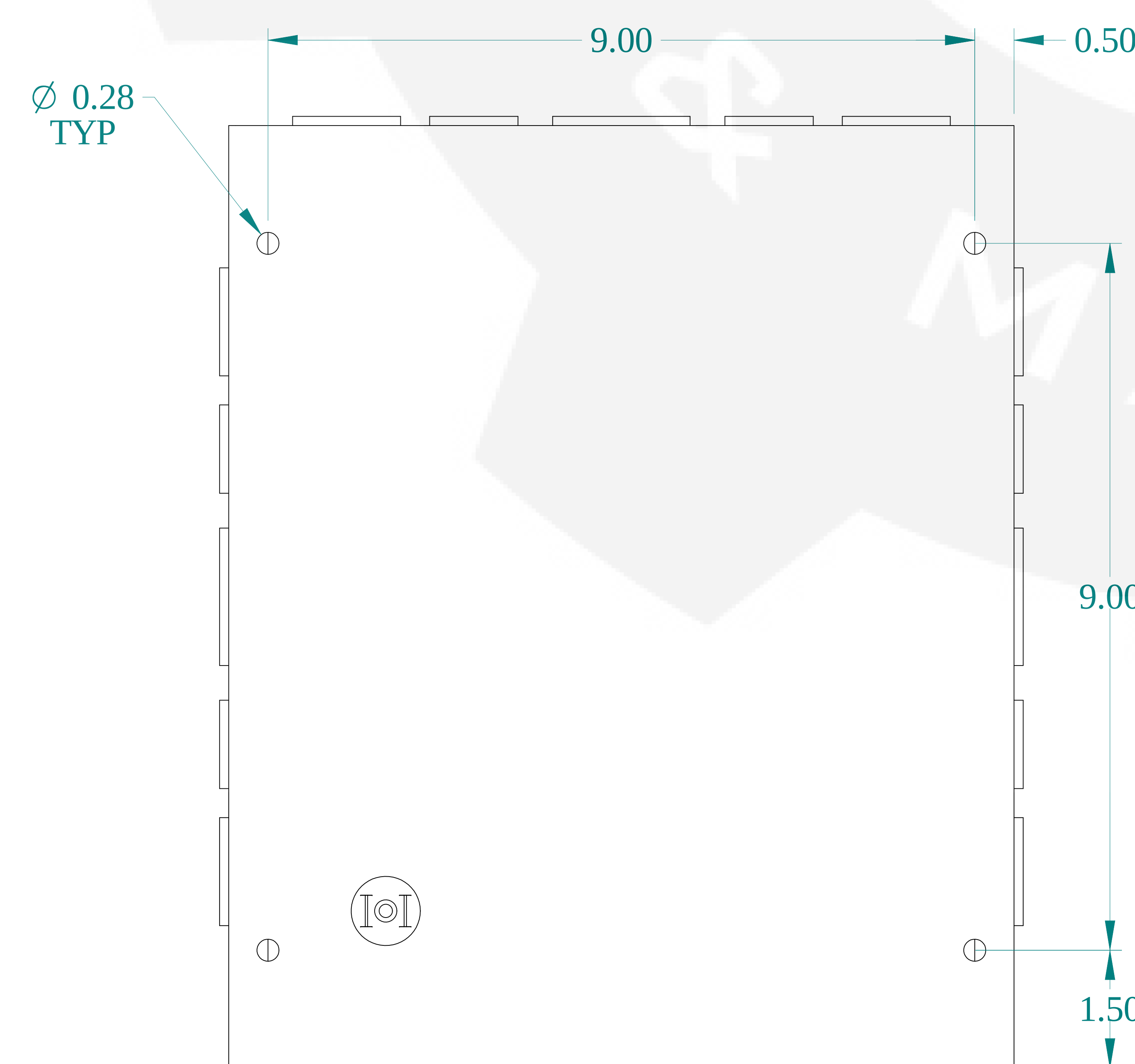
BOTTOM VIEW
