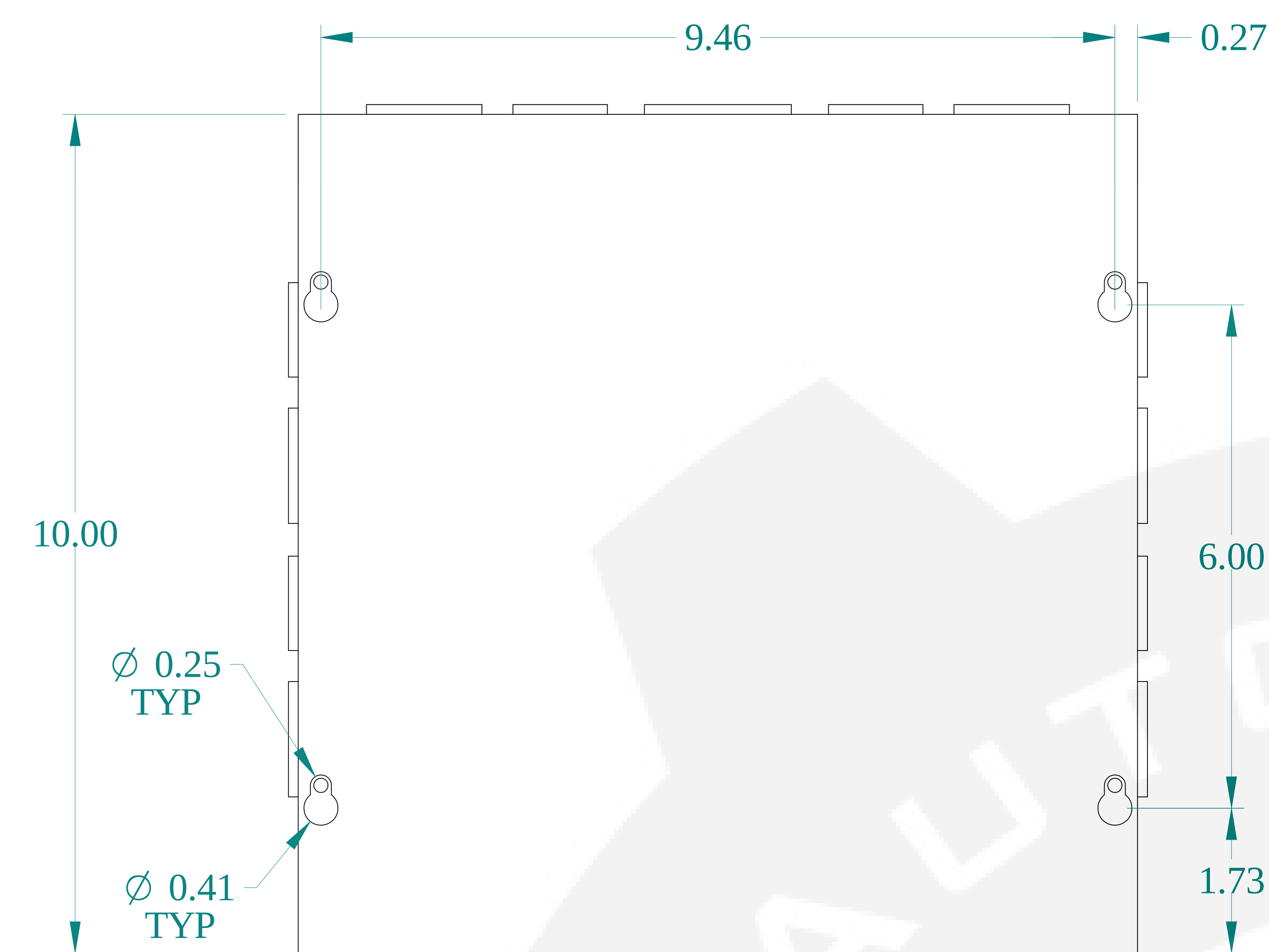
TOP VIEW
