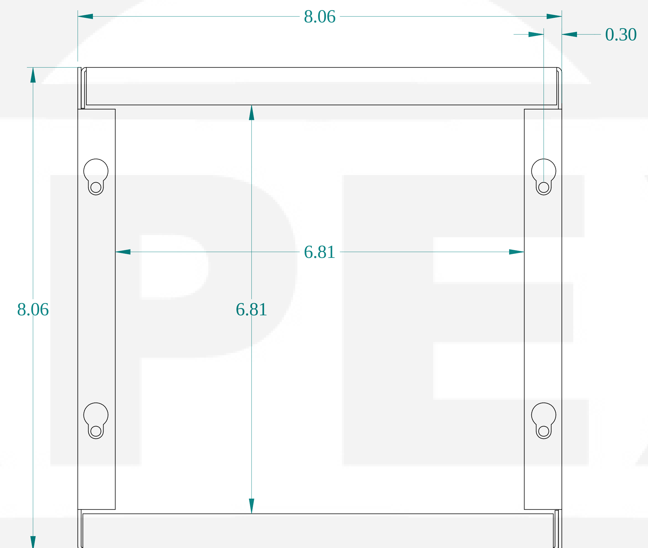
FRONT VIEW
