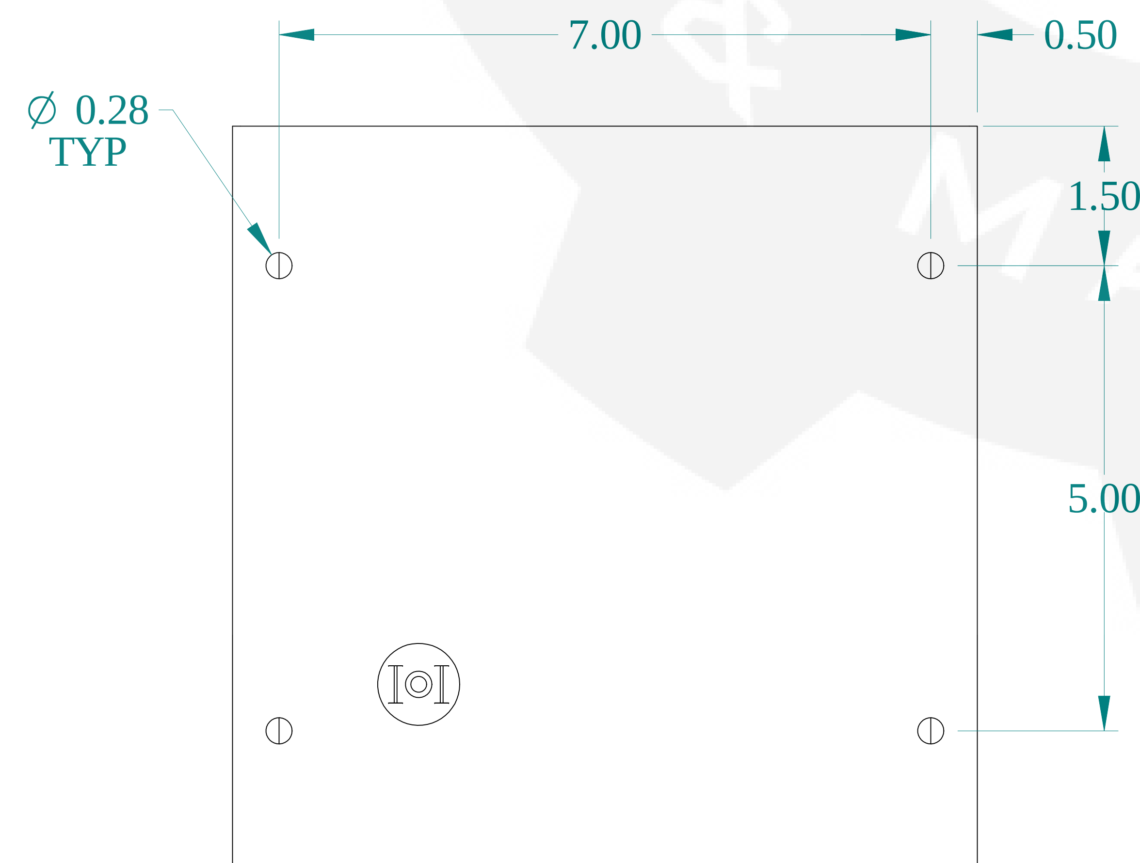
FRONT VIEW
