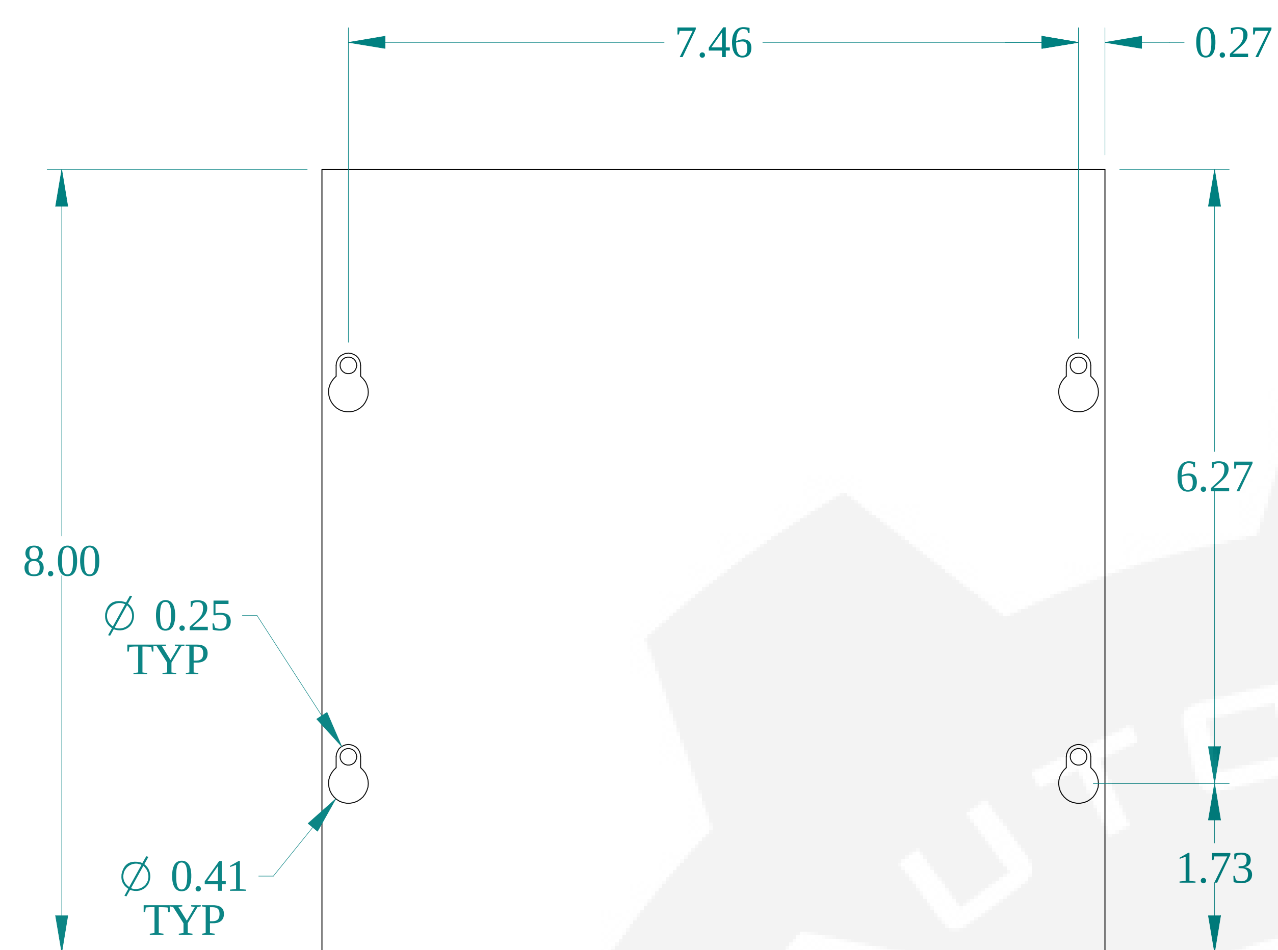
TOP VIEW
