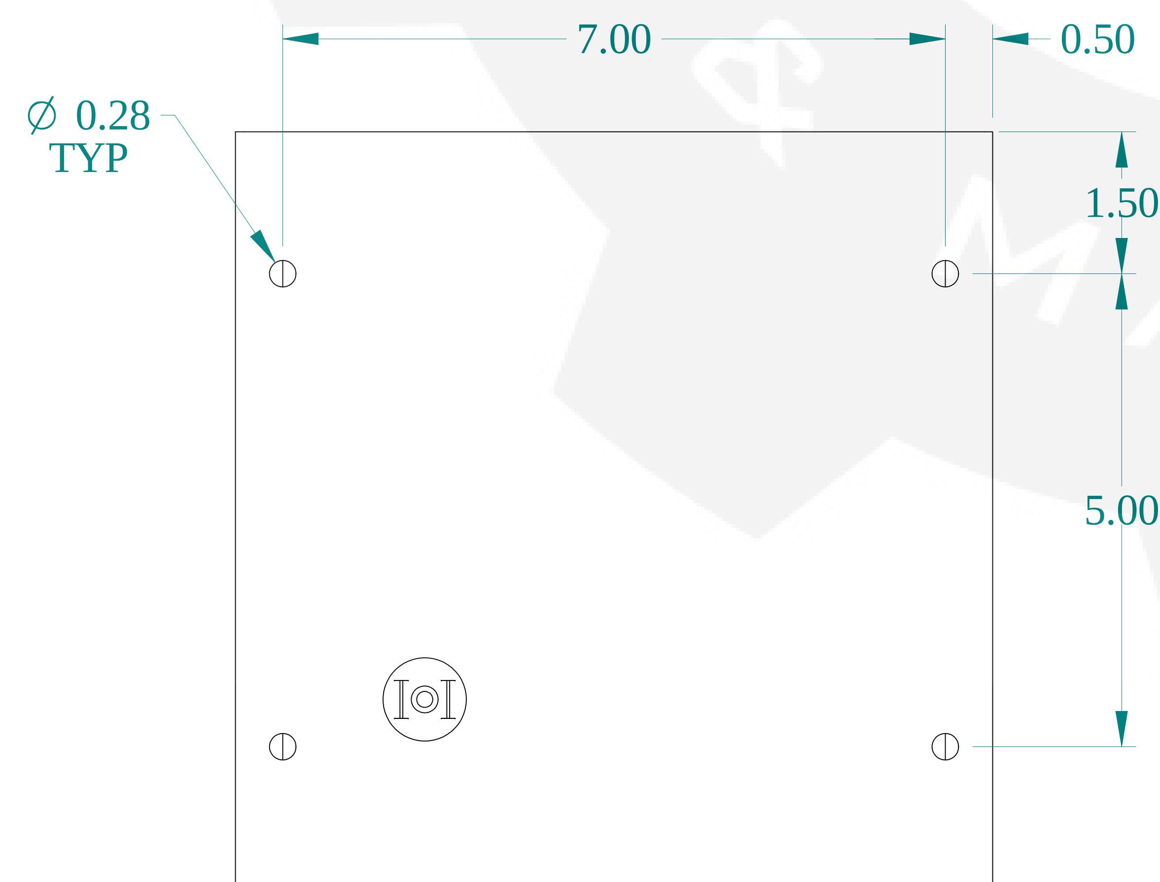
BOTTOM VIEW
