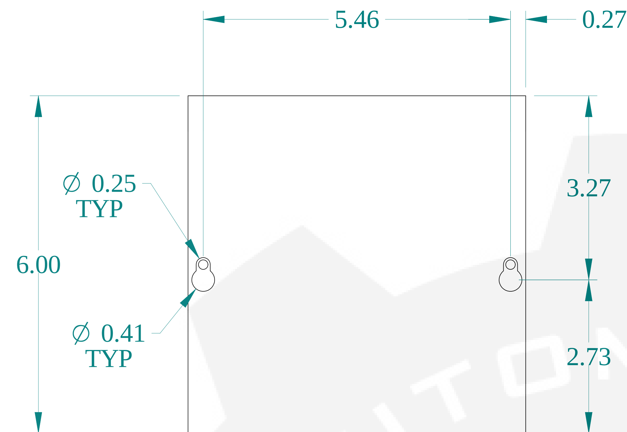
TOP VIEW
