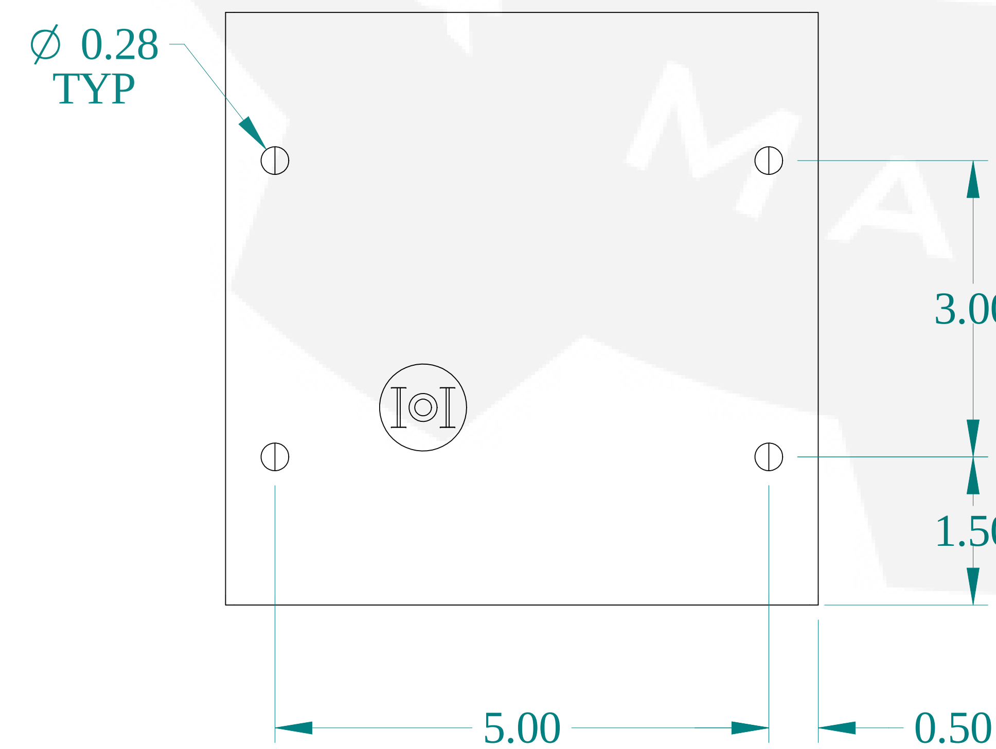
BOTTOM VIEW
