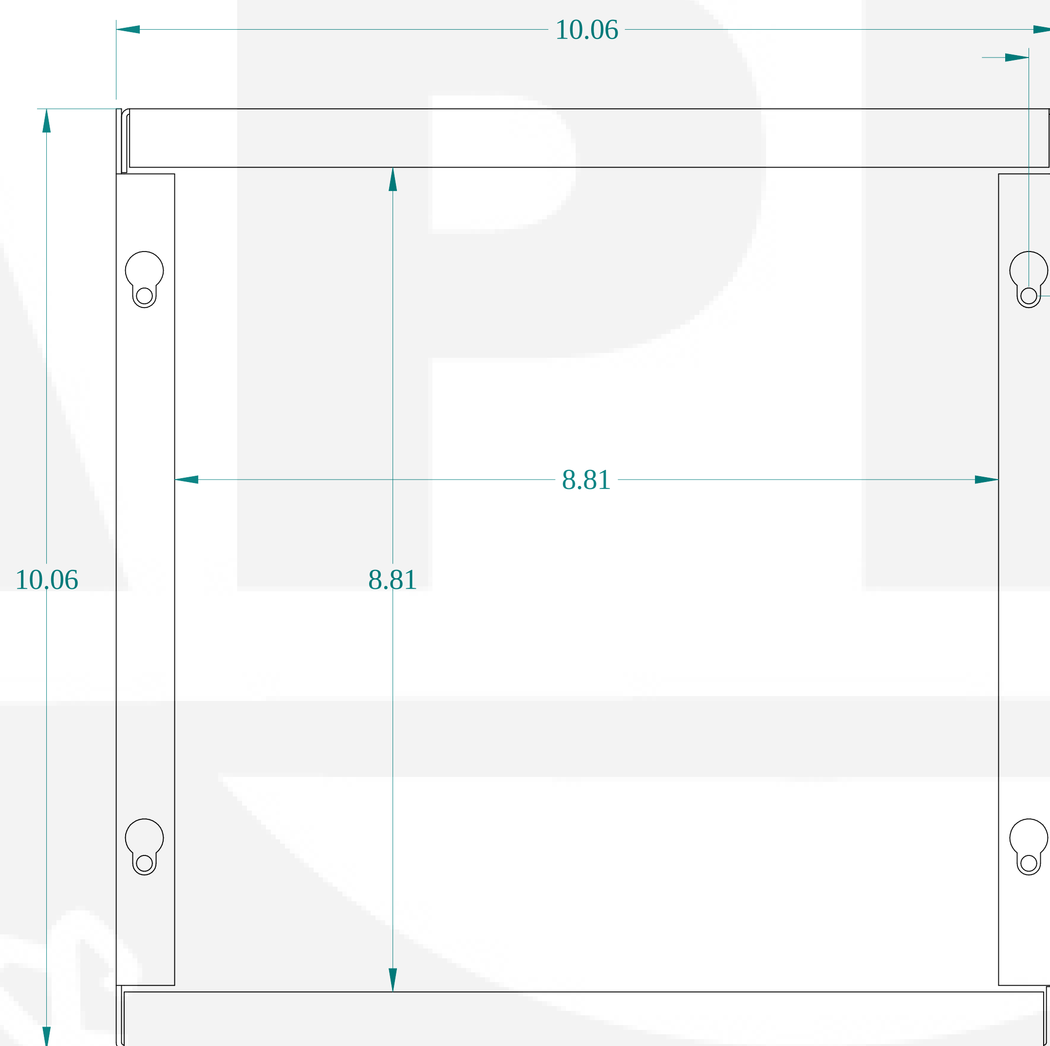
FRONT VIEW
