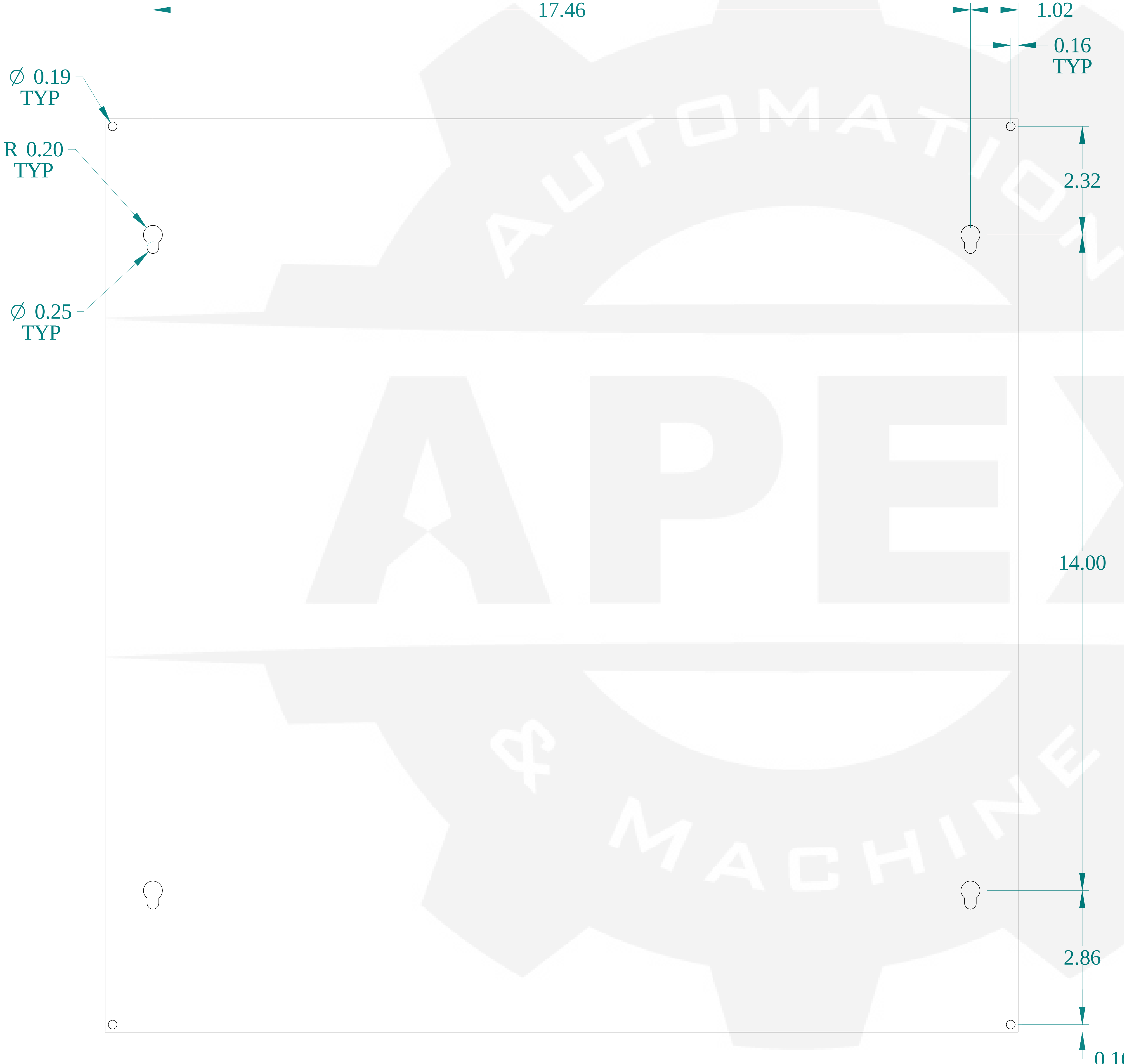
FRONT VIEW
