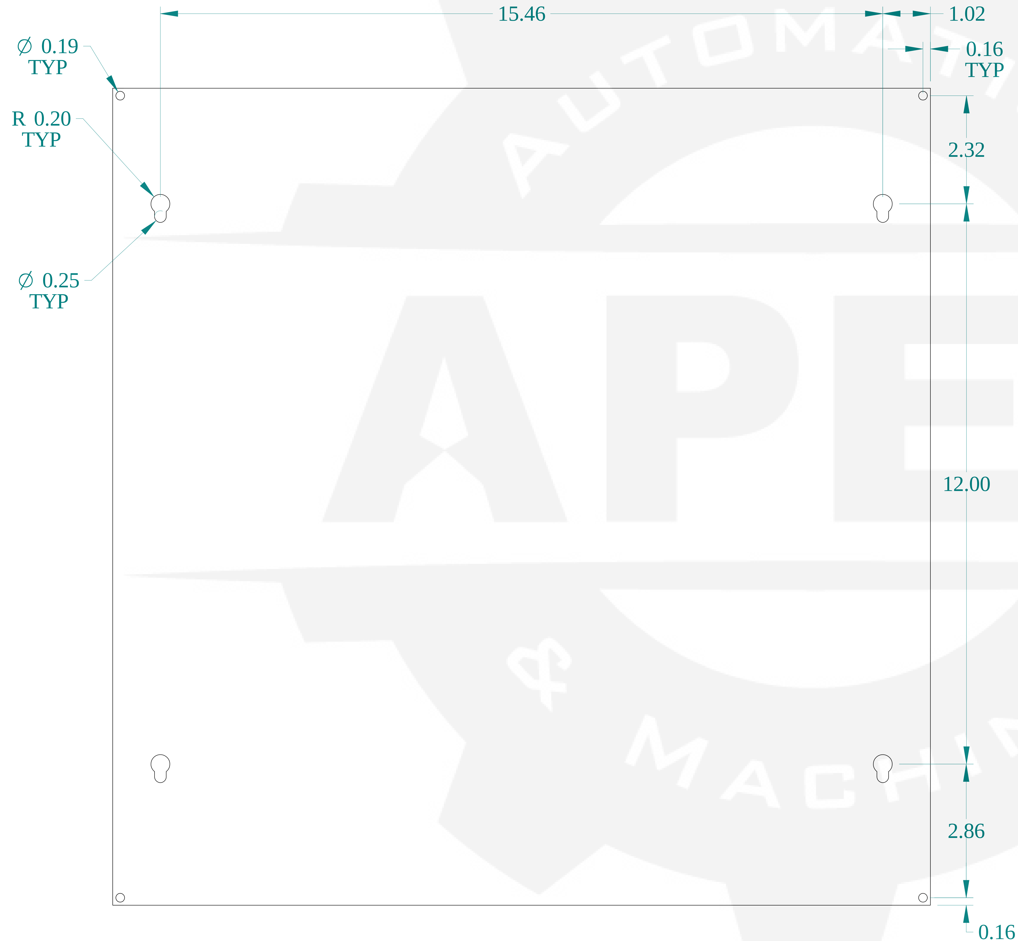
FRONT VIEW
