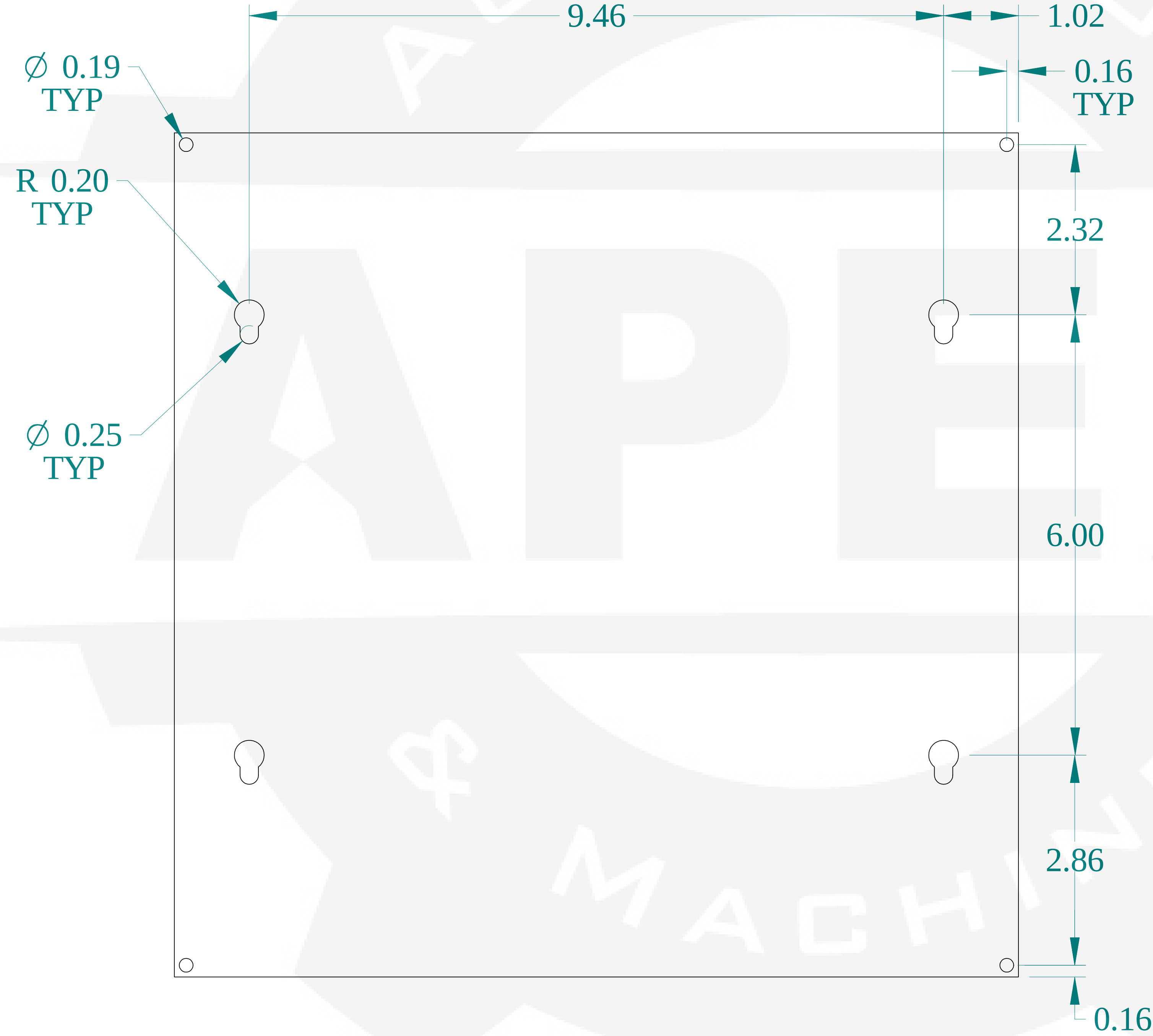
FRONT VIEW
