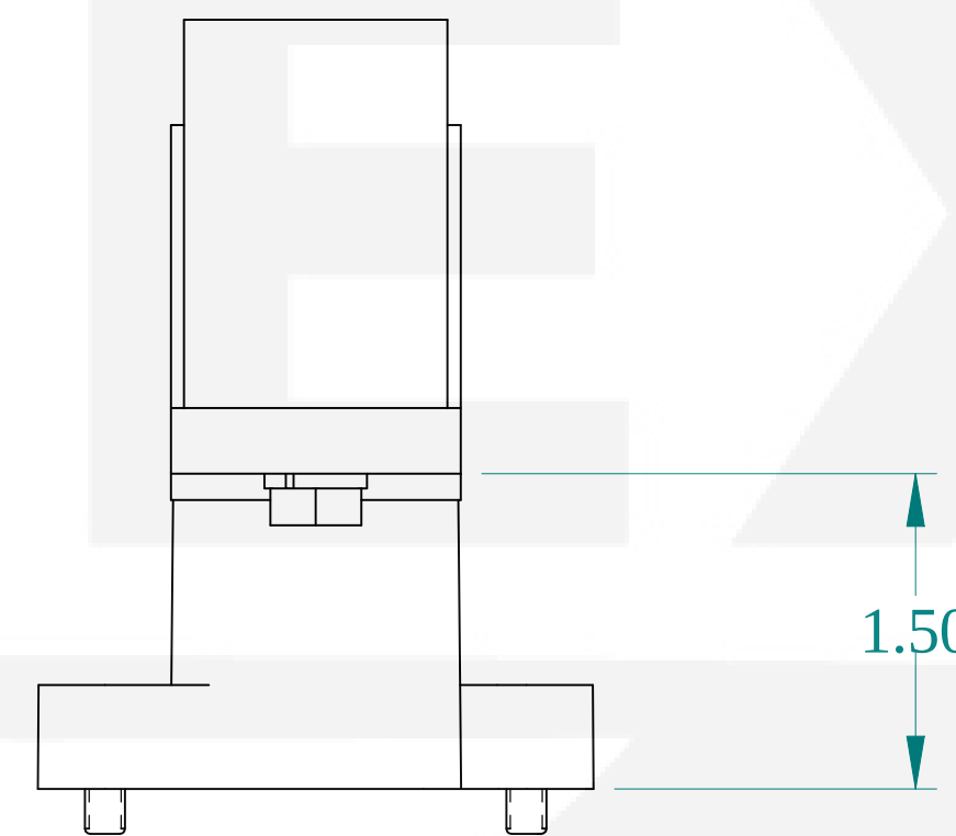
SIDE VIEW
