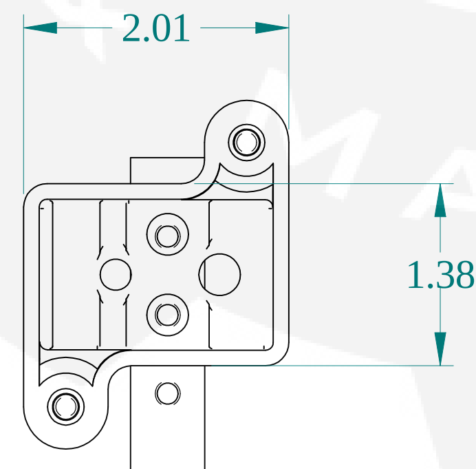
BOTTOM VIEW
