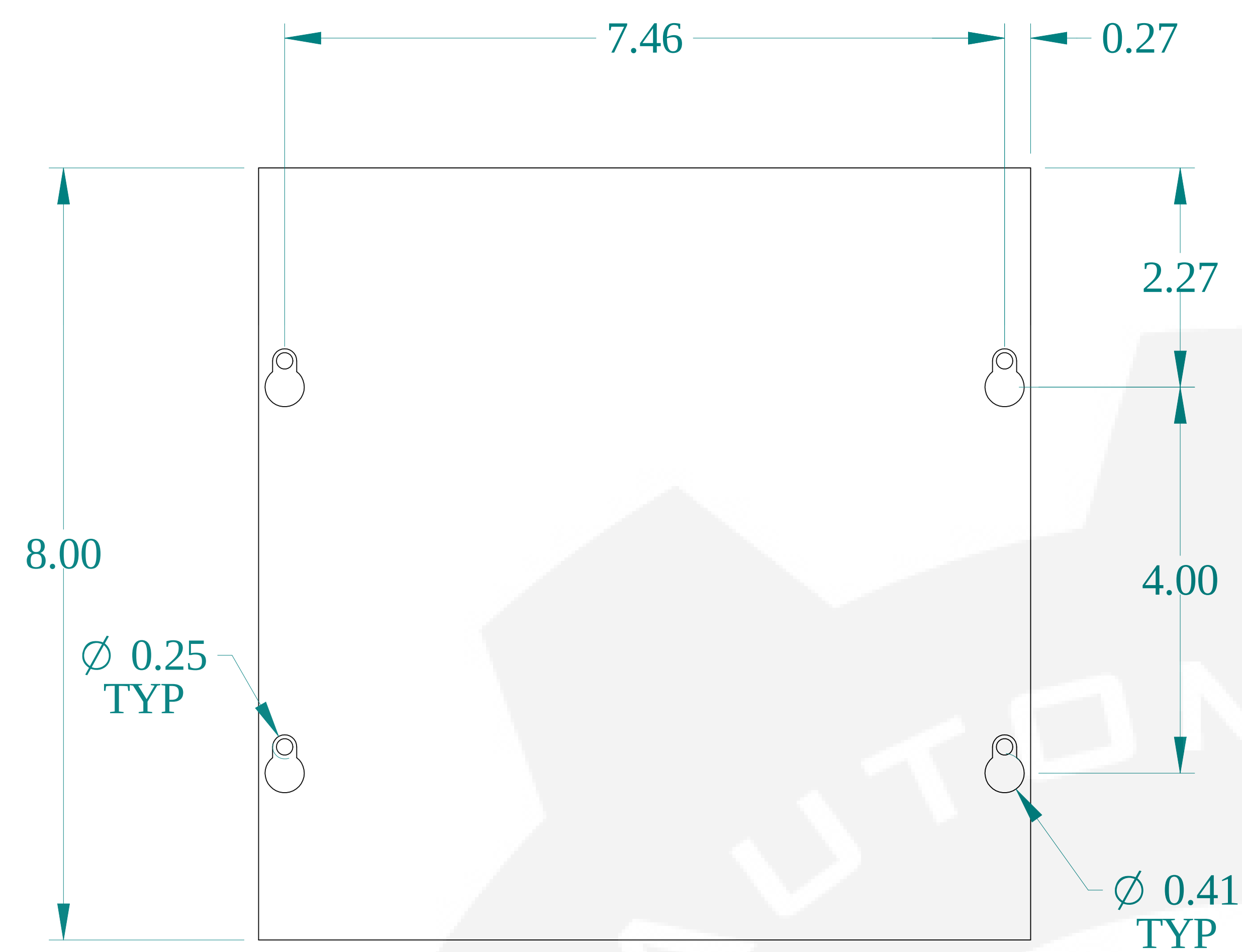
TOP VIEW
