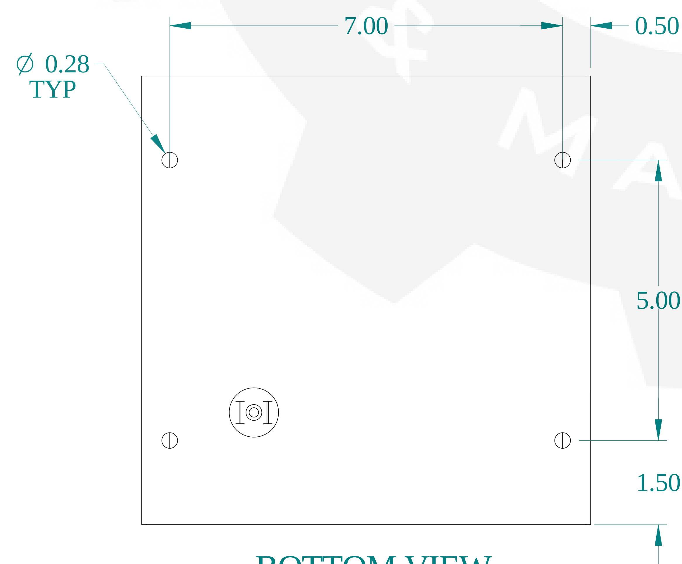
BOTTOM VIEW
