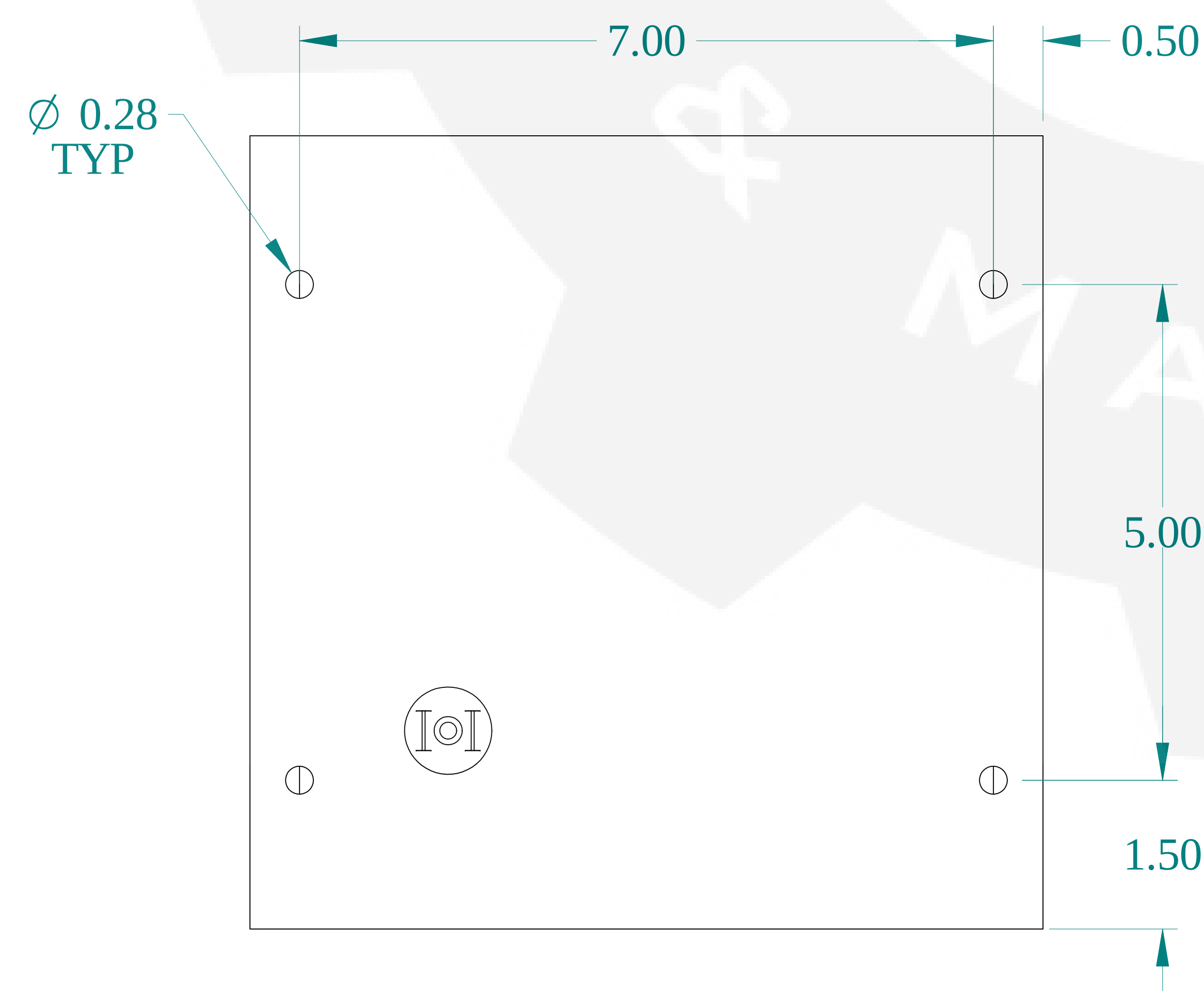
BOTTOM VIEW
