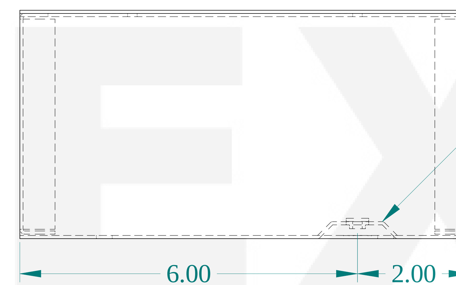
SIDE VIEW
