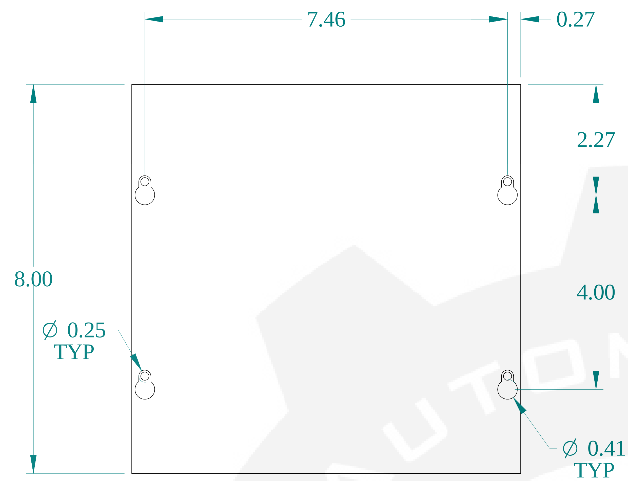
TOP VIEW
