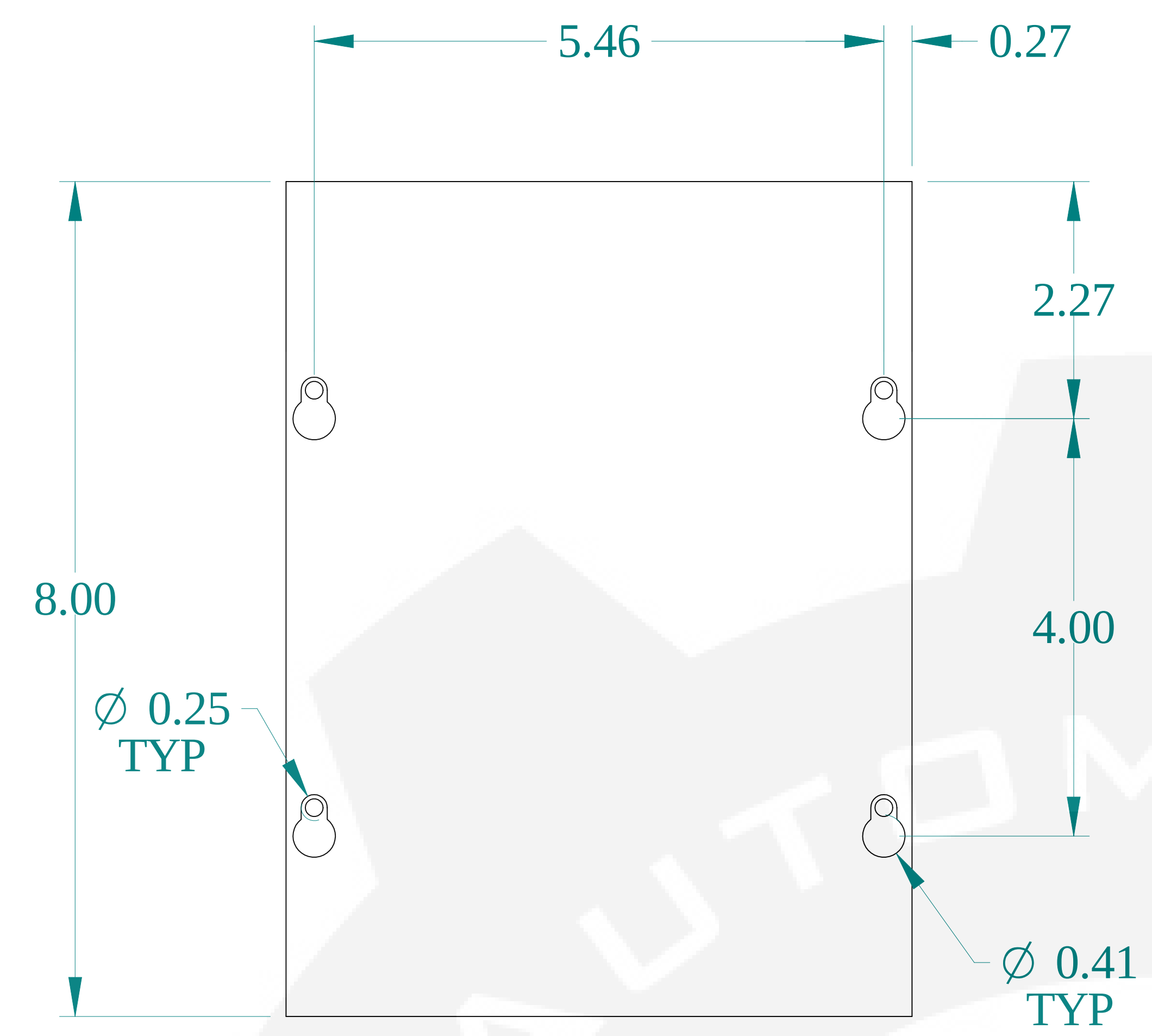
TOP VIEW
