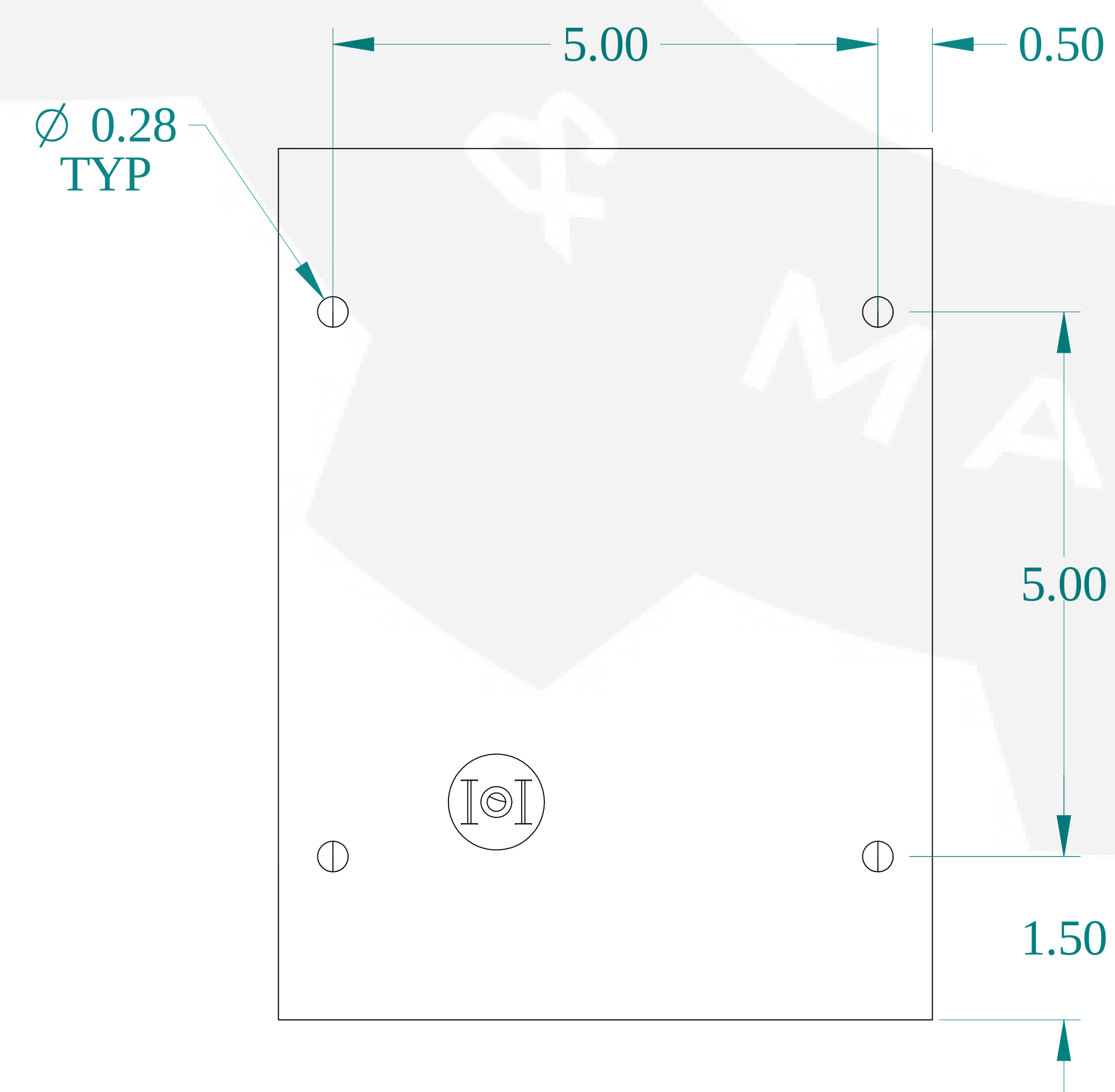
BOTTOM VIEW
