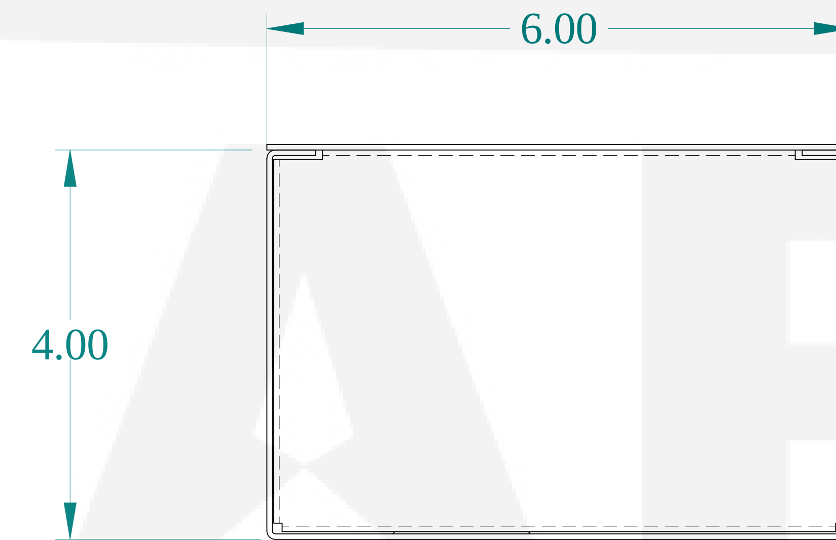
TOP VIEW
