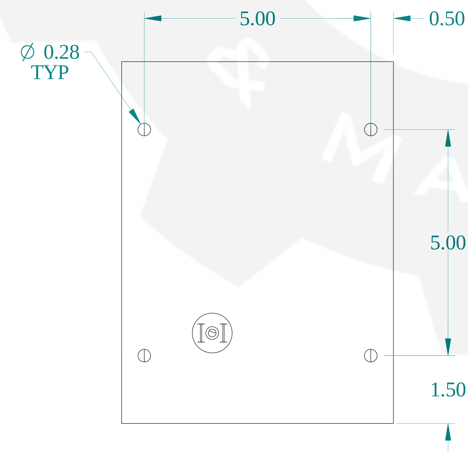
BOTTOM VIEW
