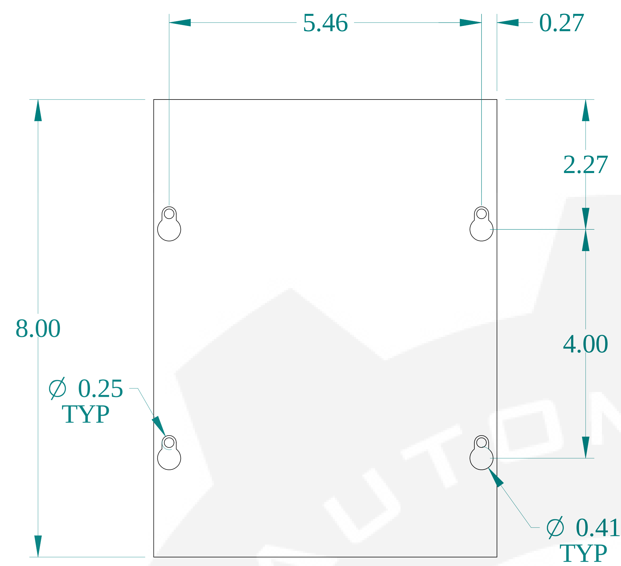
TOP VIEW
