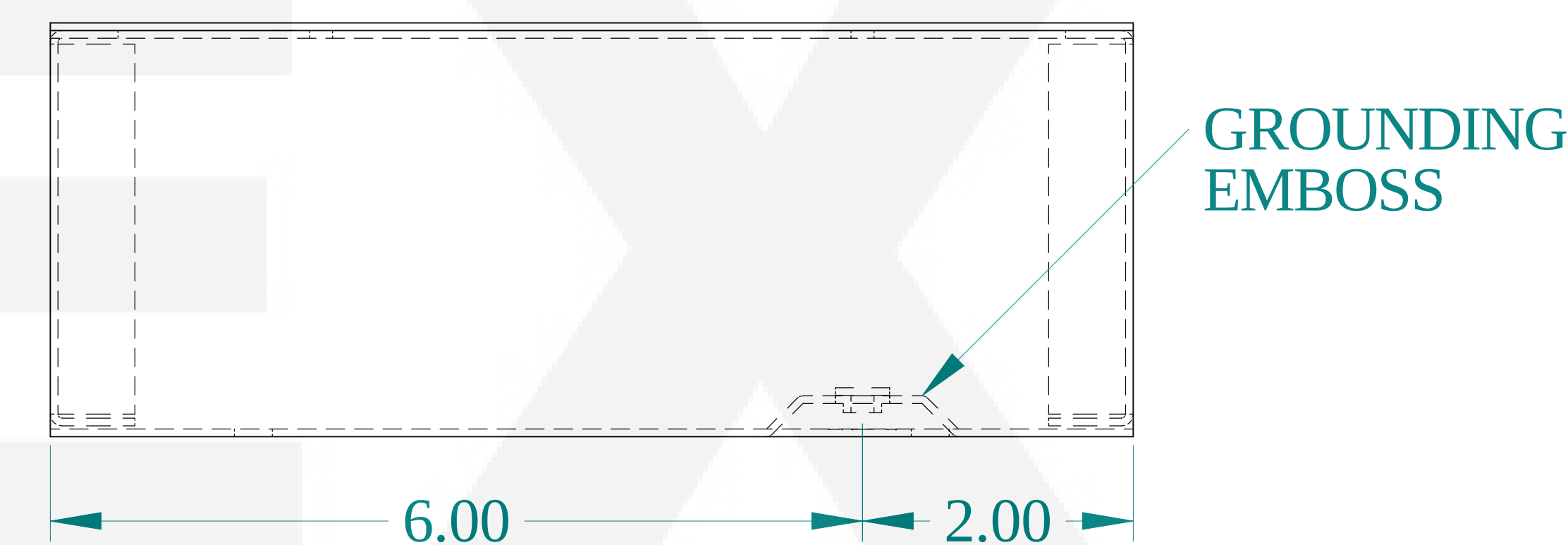
SIDE VIEW
