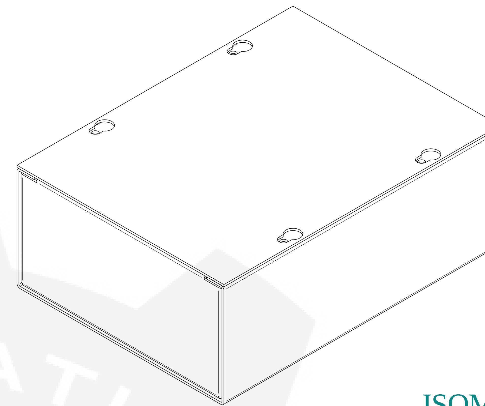
ISOMETRIC VIEWS
