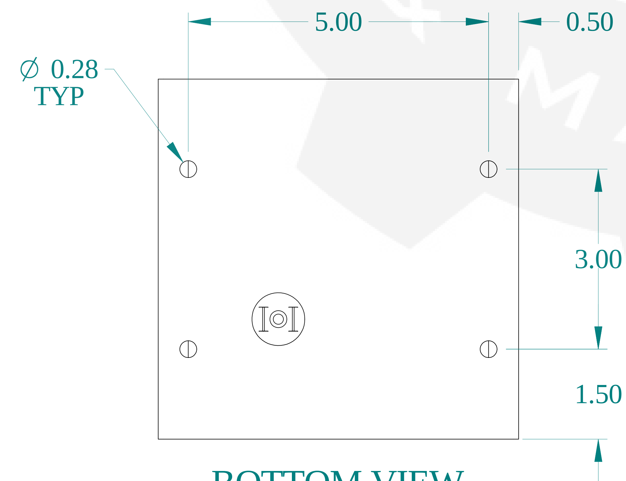
BOTTOM VIEW
