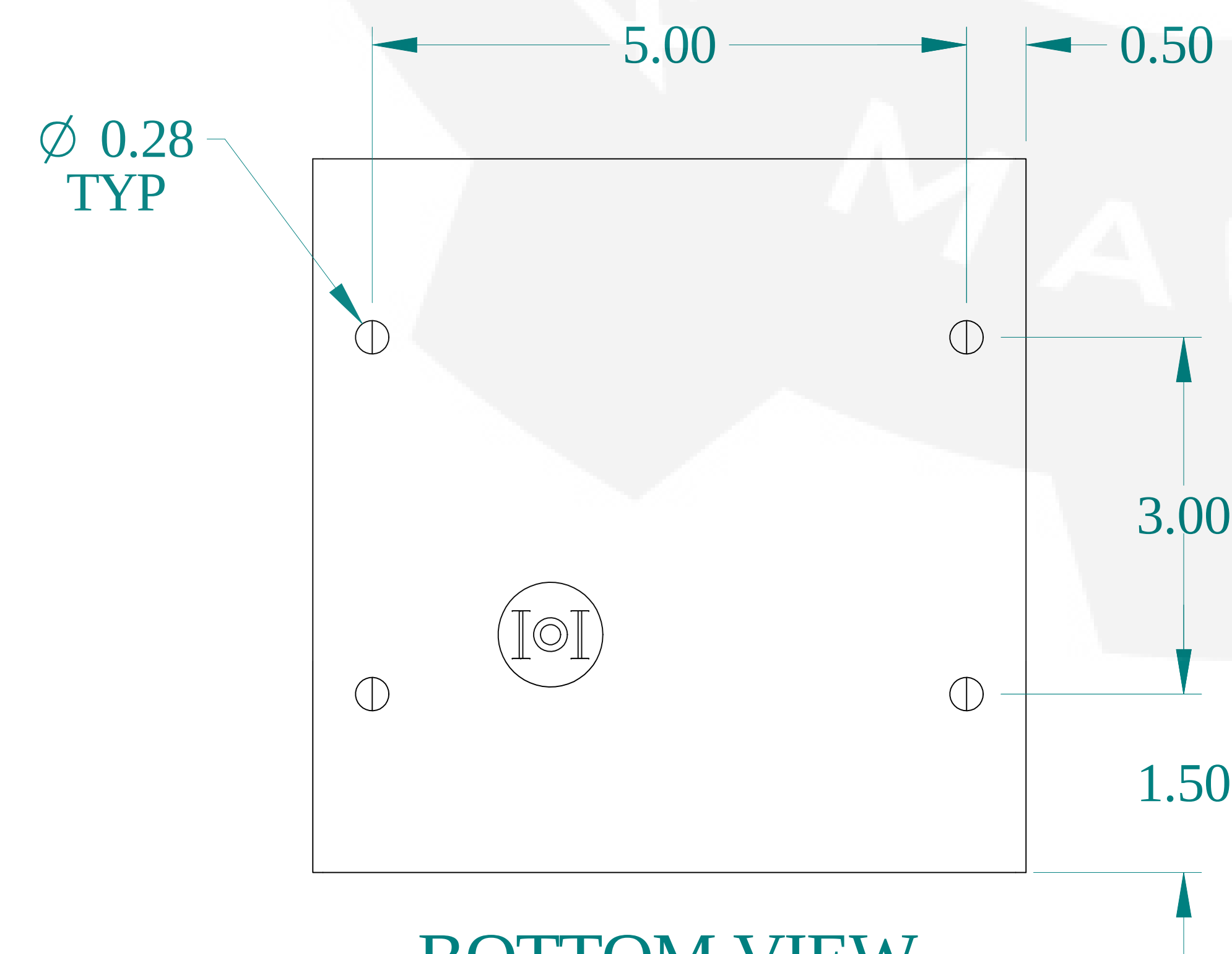
BOTTOM VIEW
