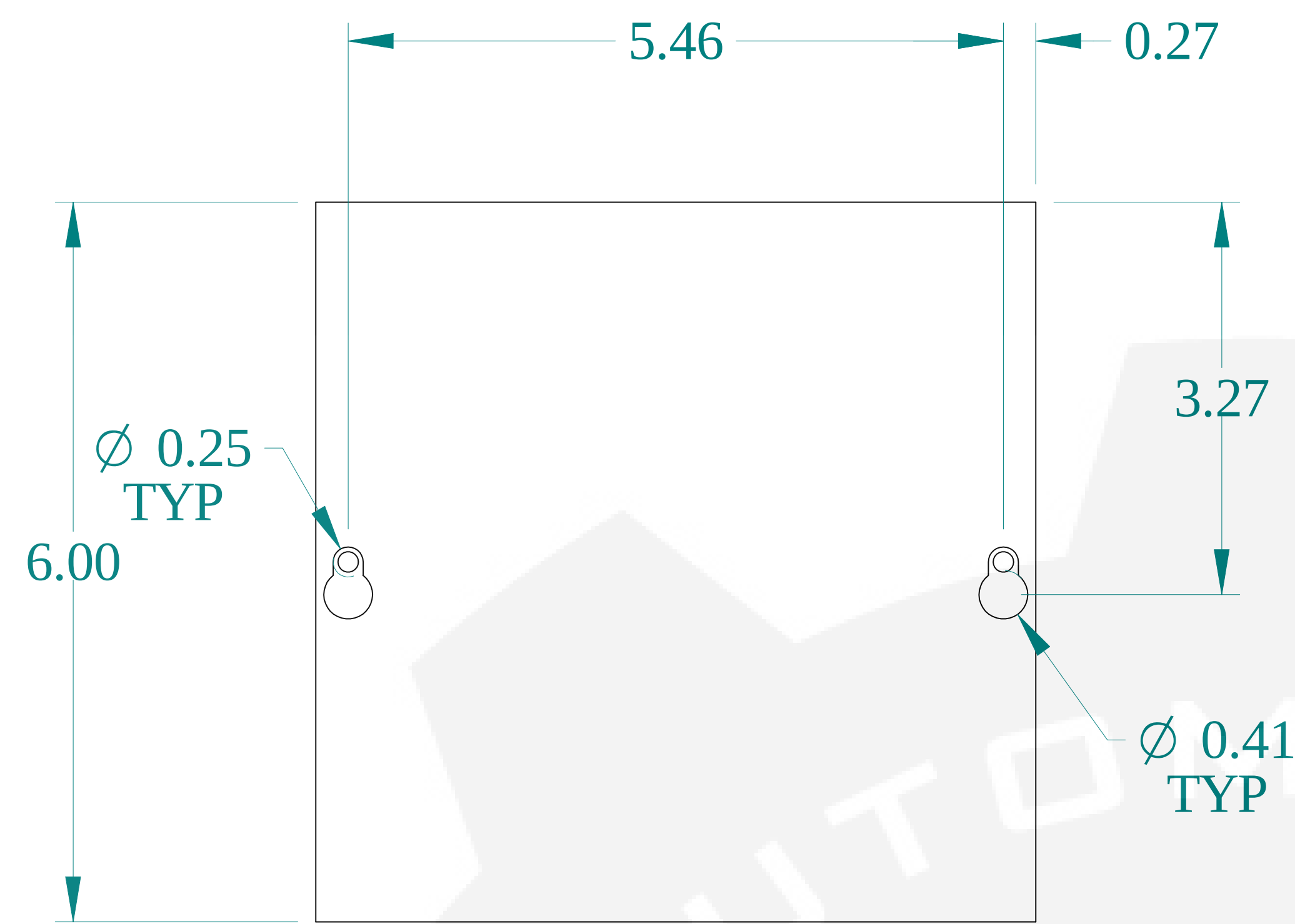
TOP VIEW
