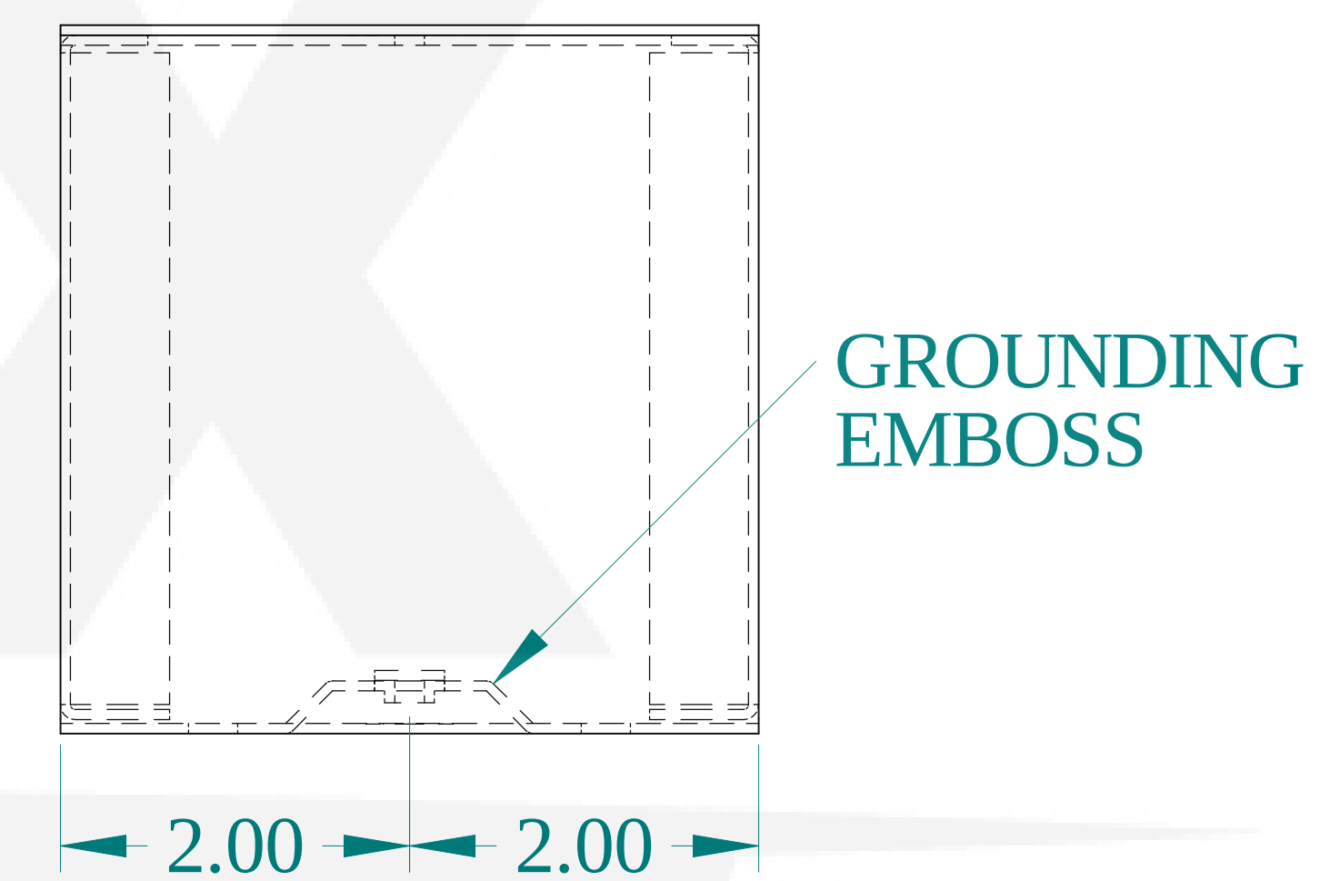
SIDE VIEW
