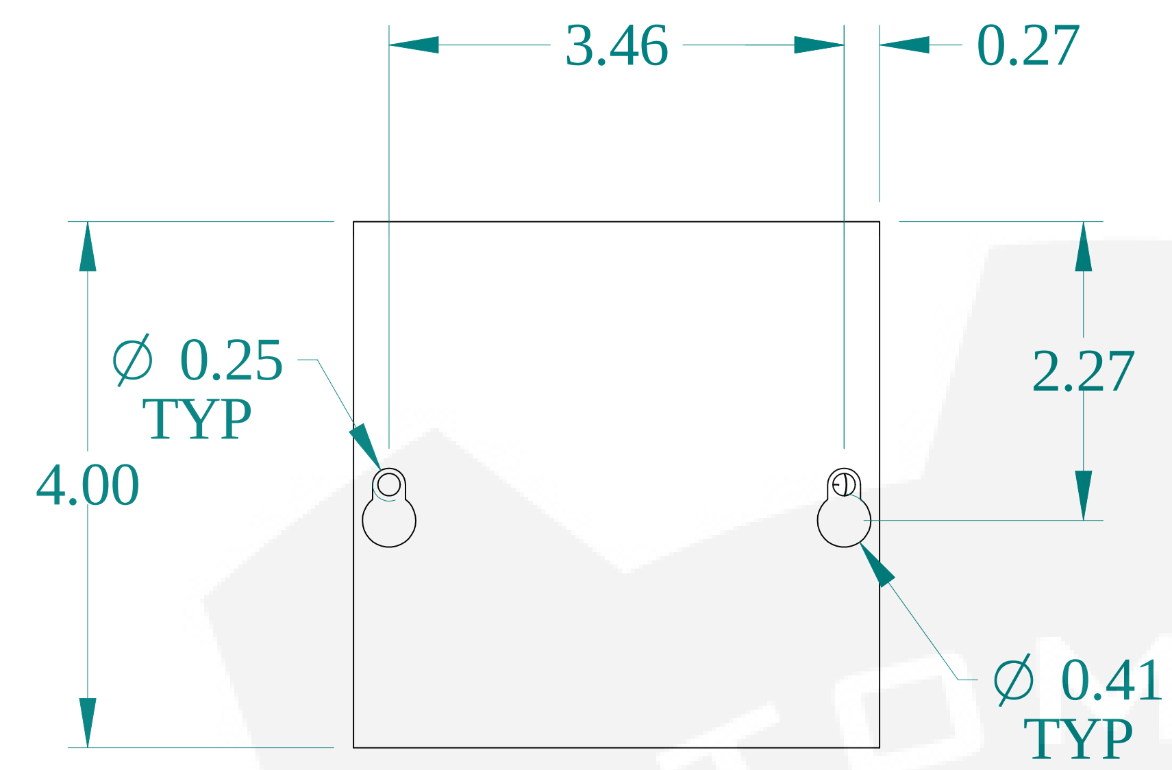
TOP VIEW
