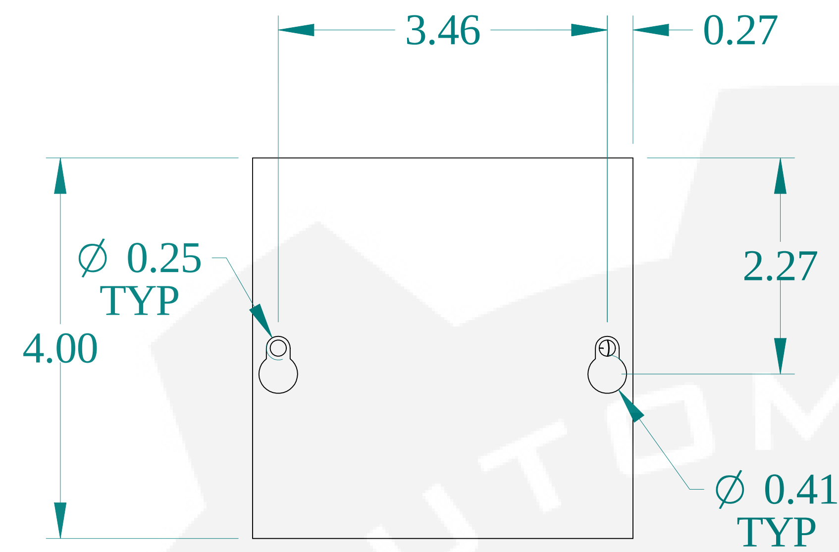
TOP VIEW
