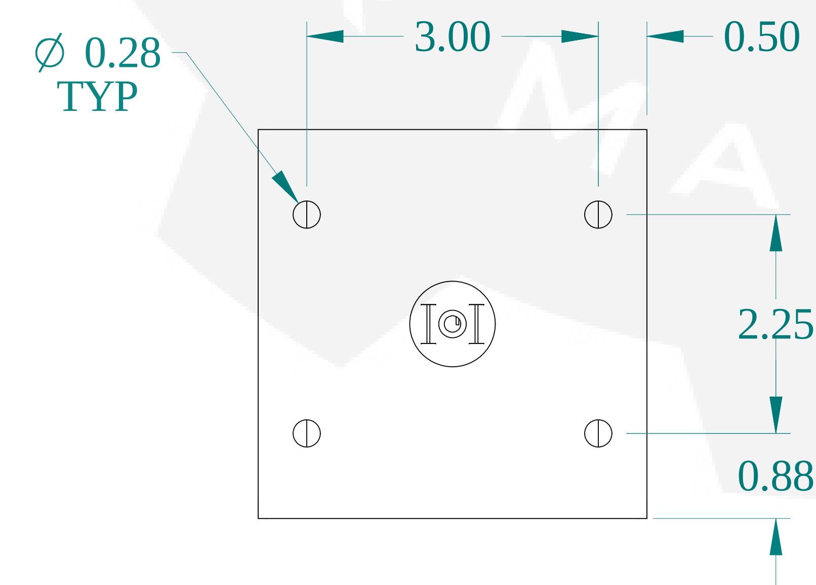
BOTTOM VIEW
