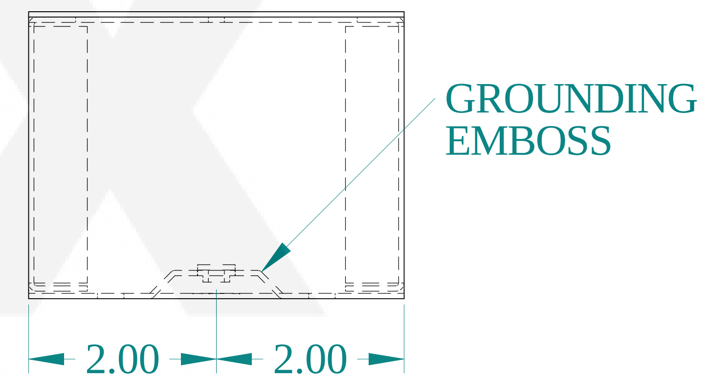
SIDE VIEW
