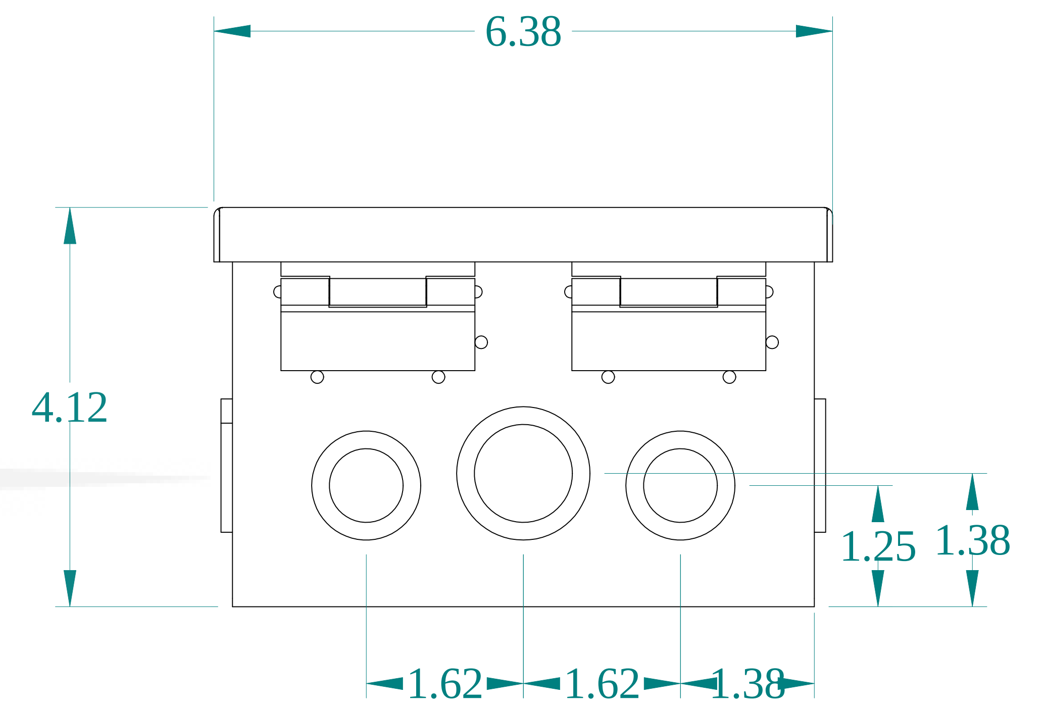
BACK VIEW
