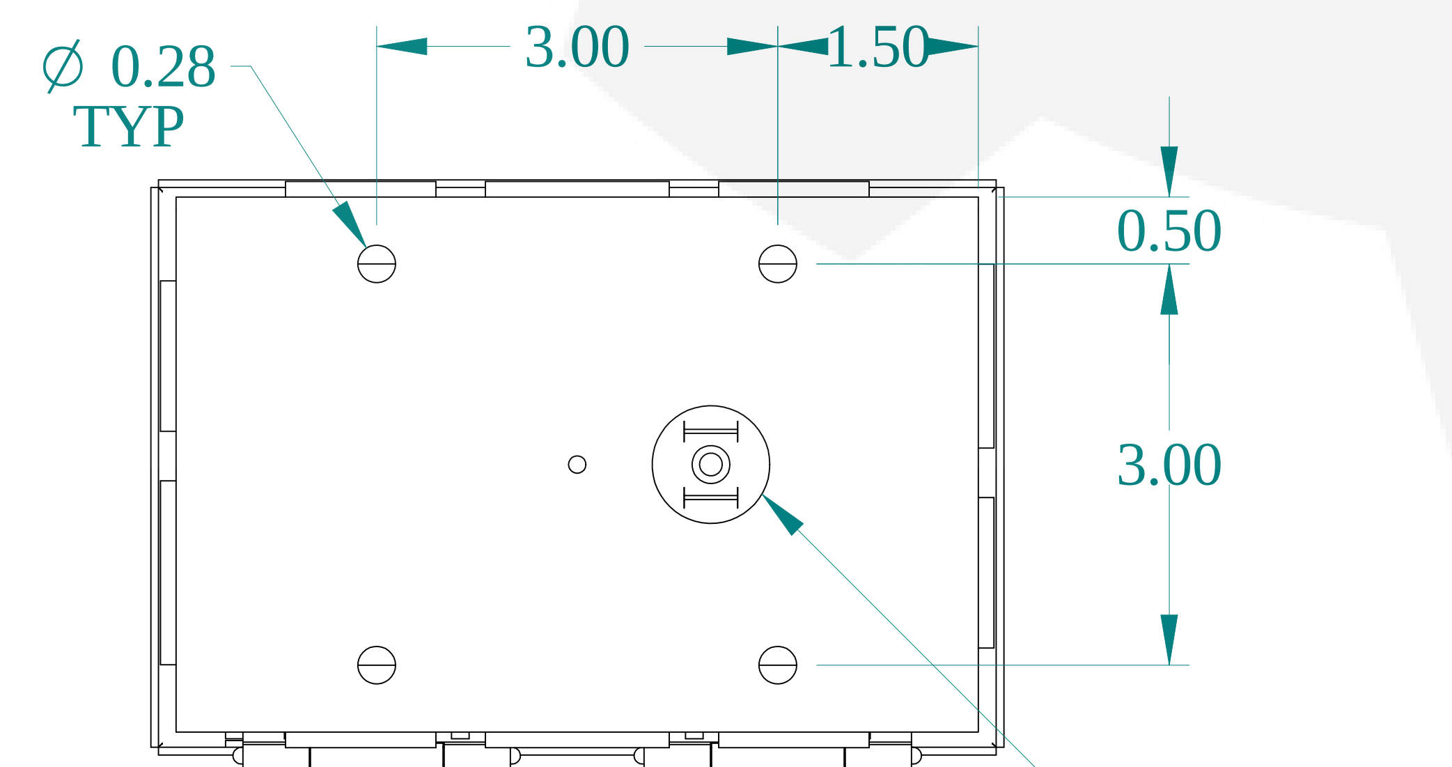
BOTTOM VIEW
