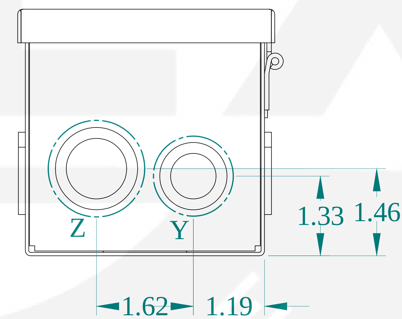
SIDE VIEW
