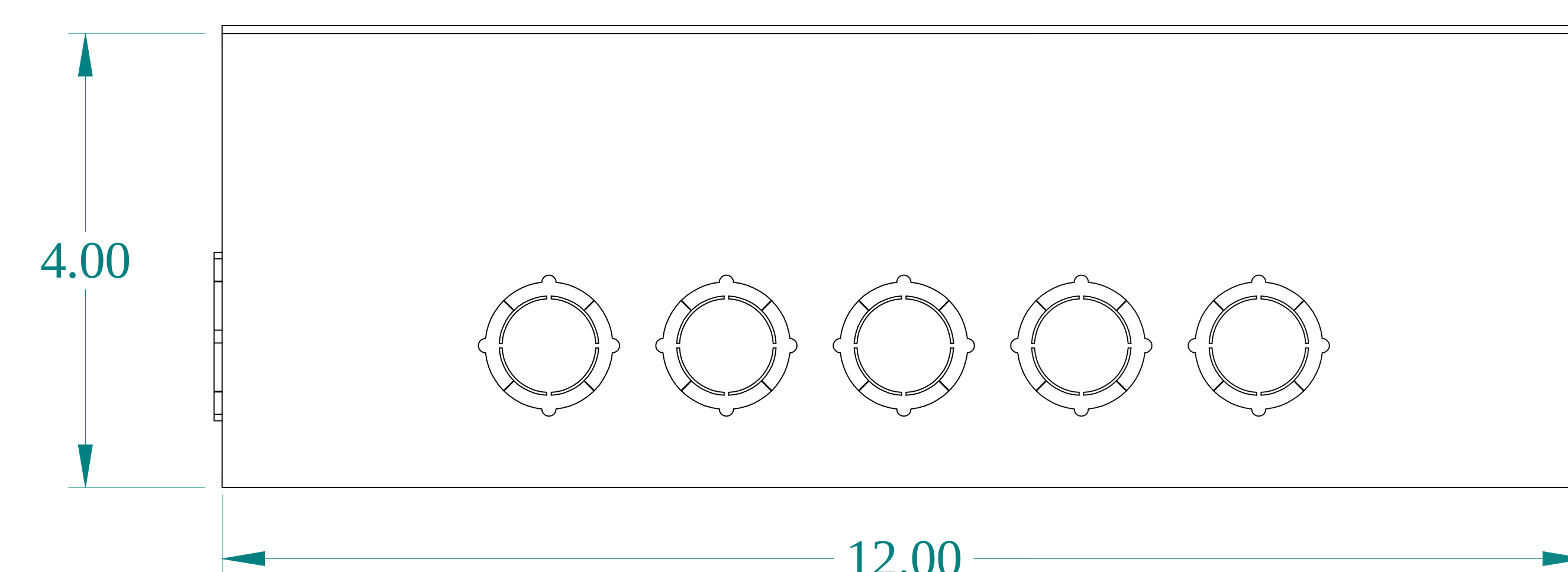
SIDE VIEW
