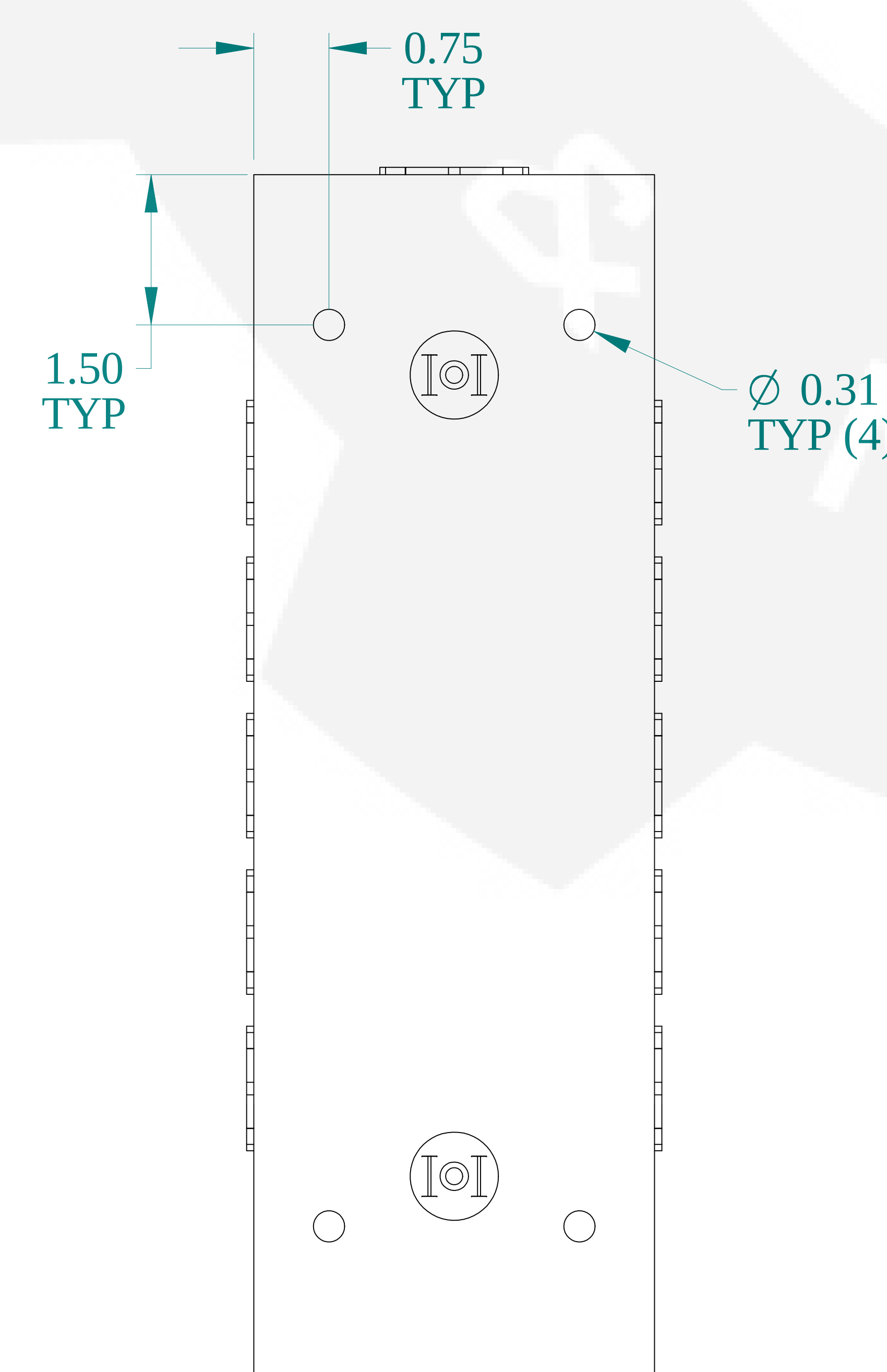
BOTTOM VIEW
