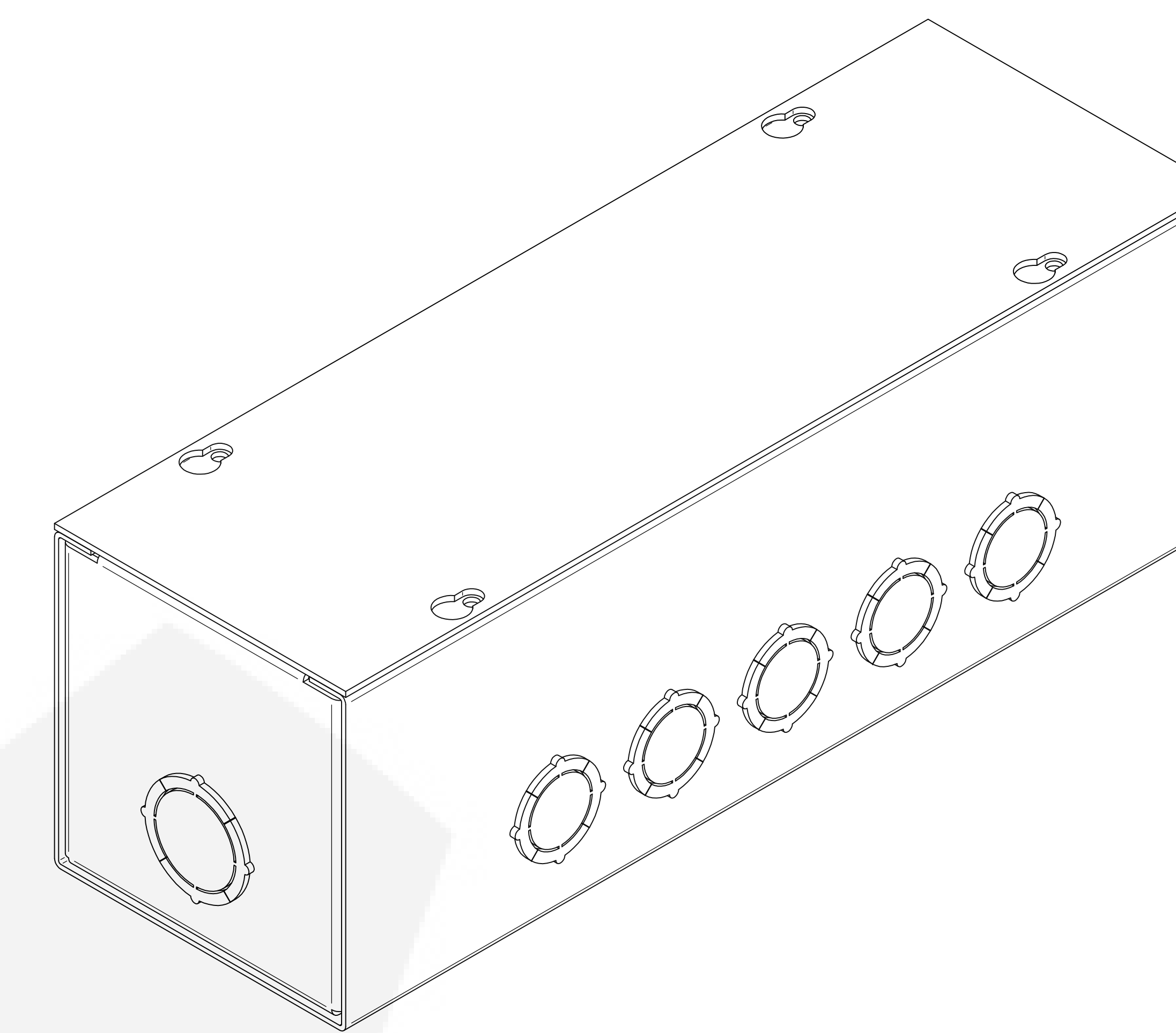
ISOMETRIC VIEWS
