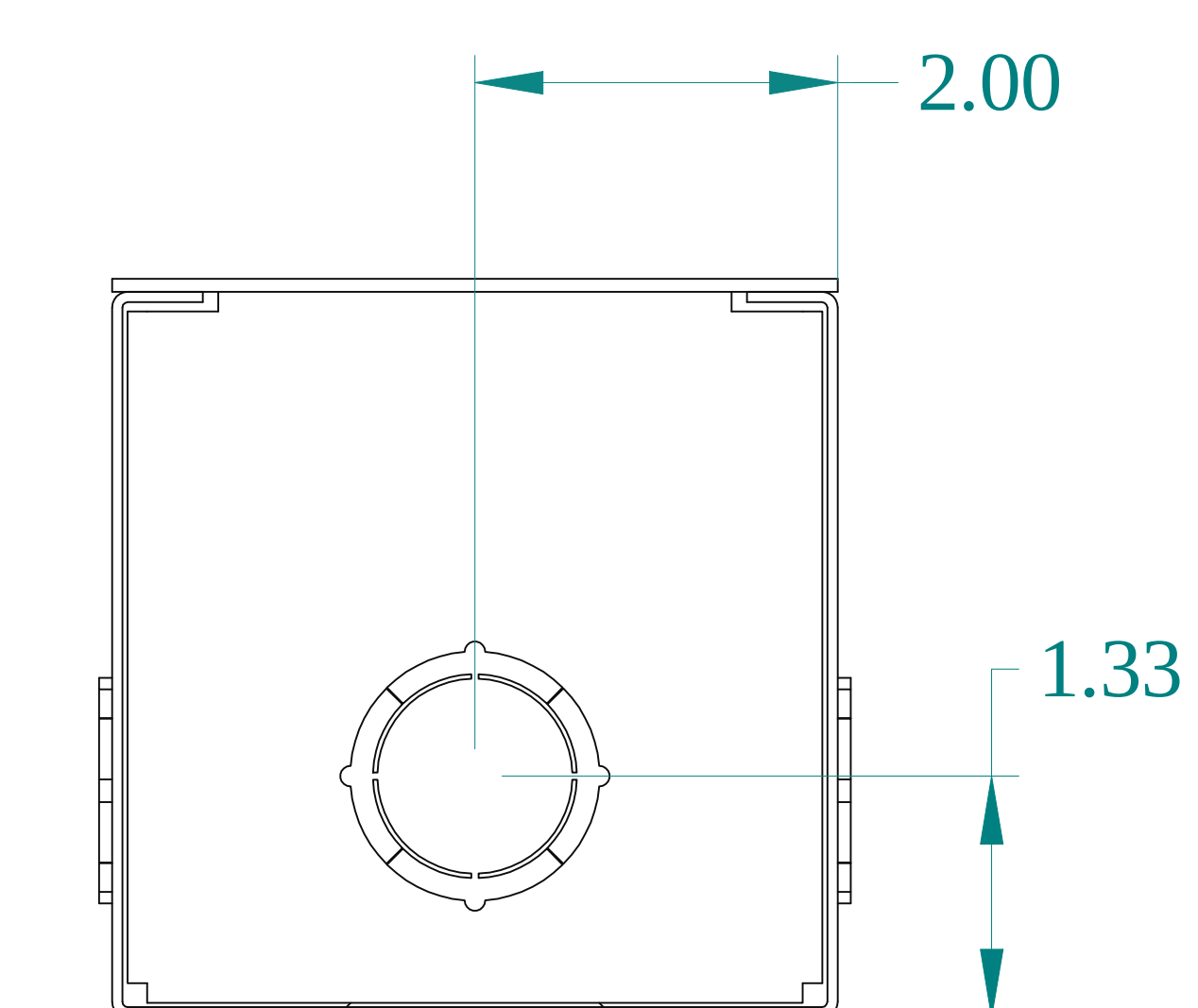
BACK VIEW
