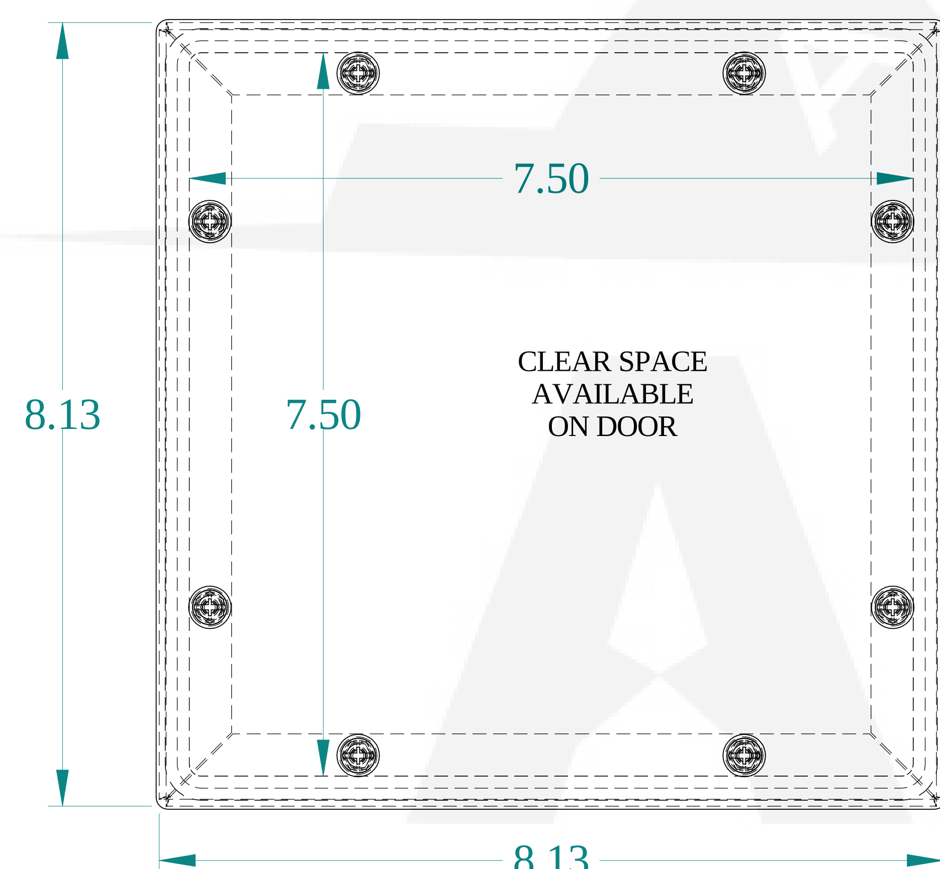
FRONT VIEW
