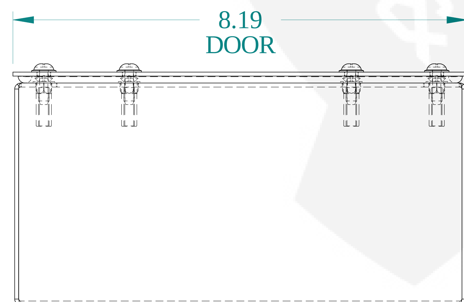
BOTTOM VIEW
