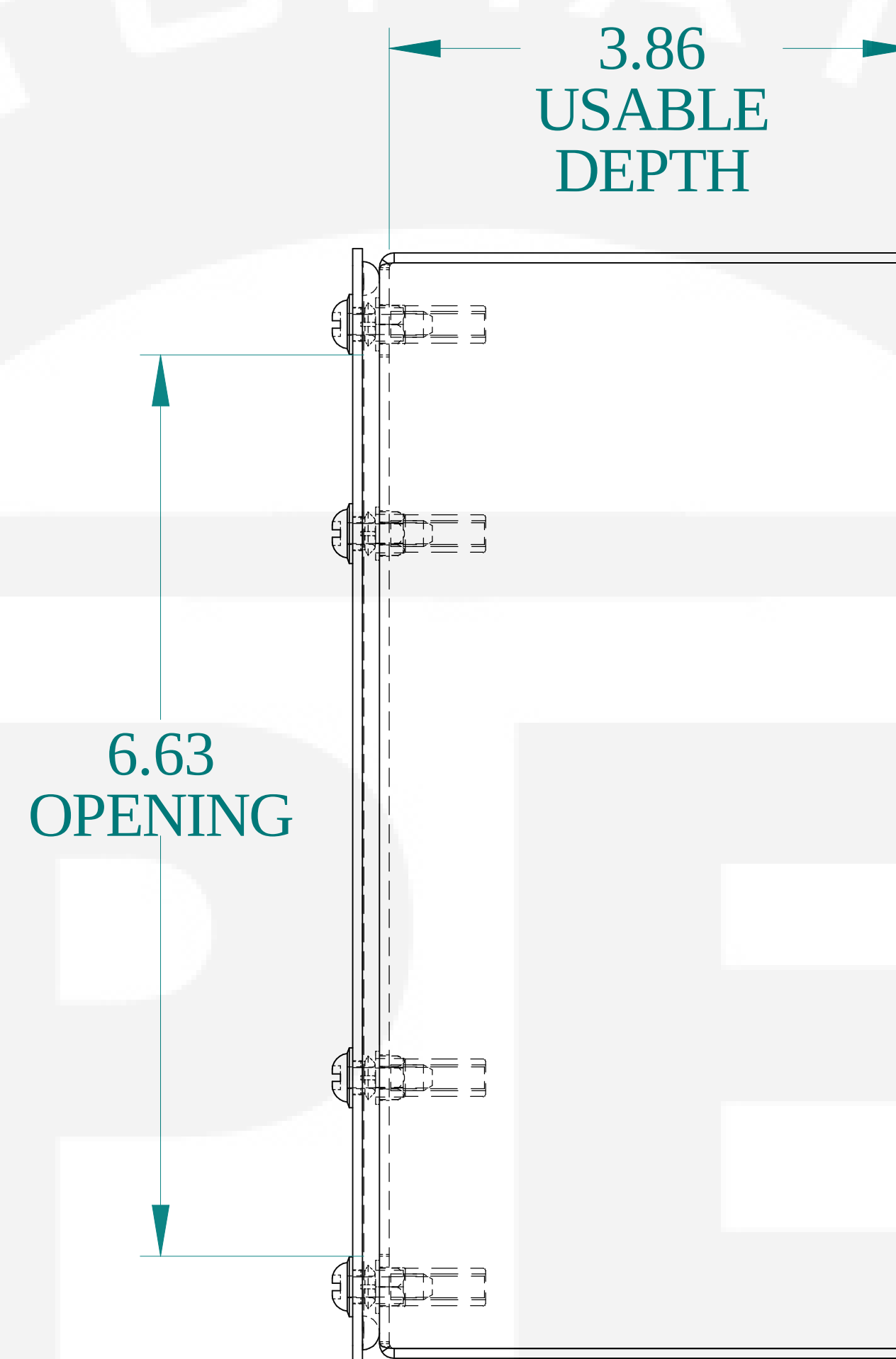
SIDE VIEW
