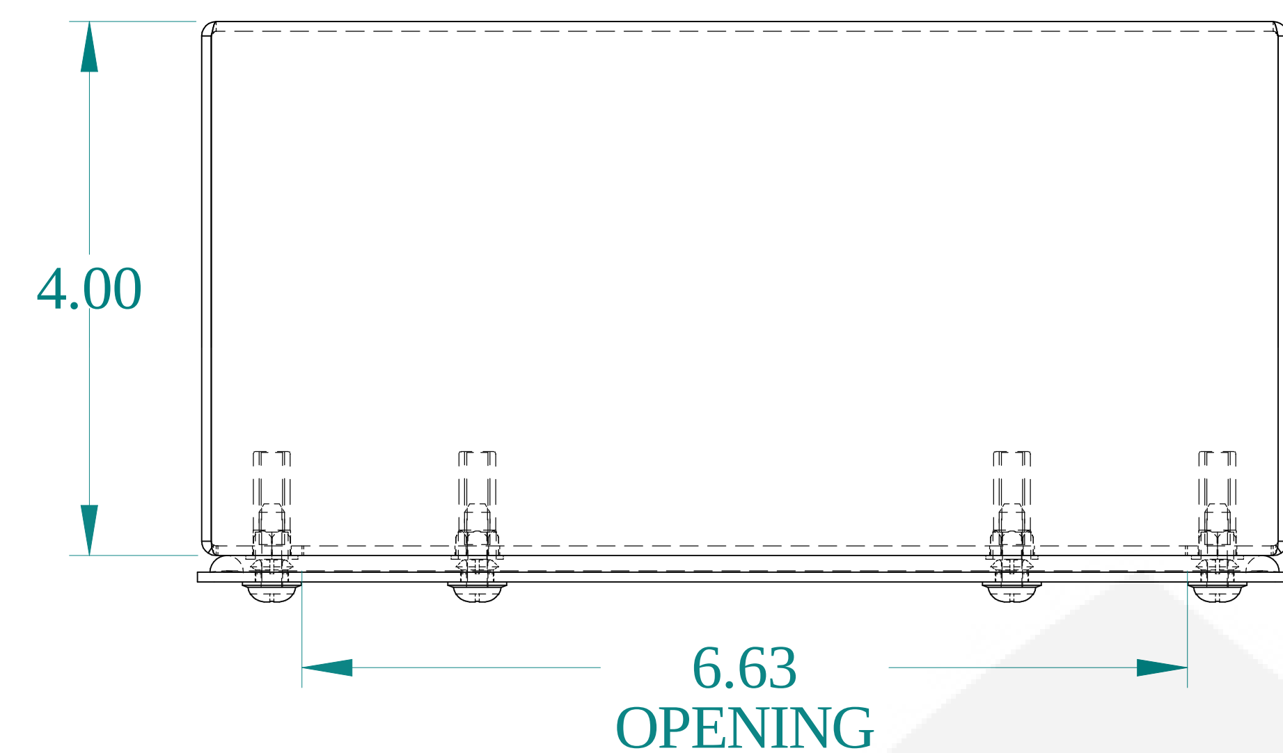
TOP VIEW
