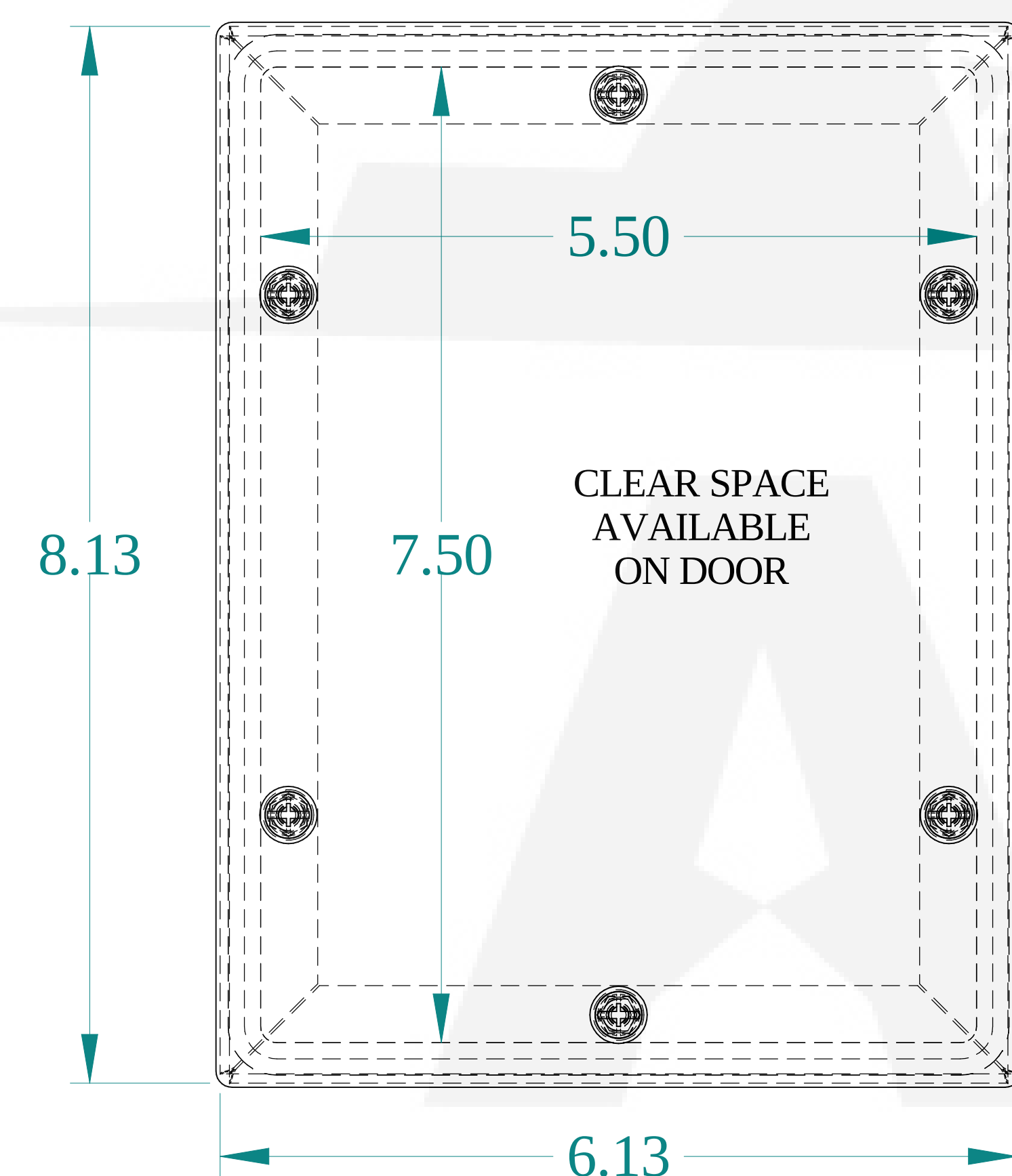
FRONT VIEW
