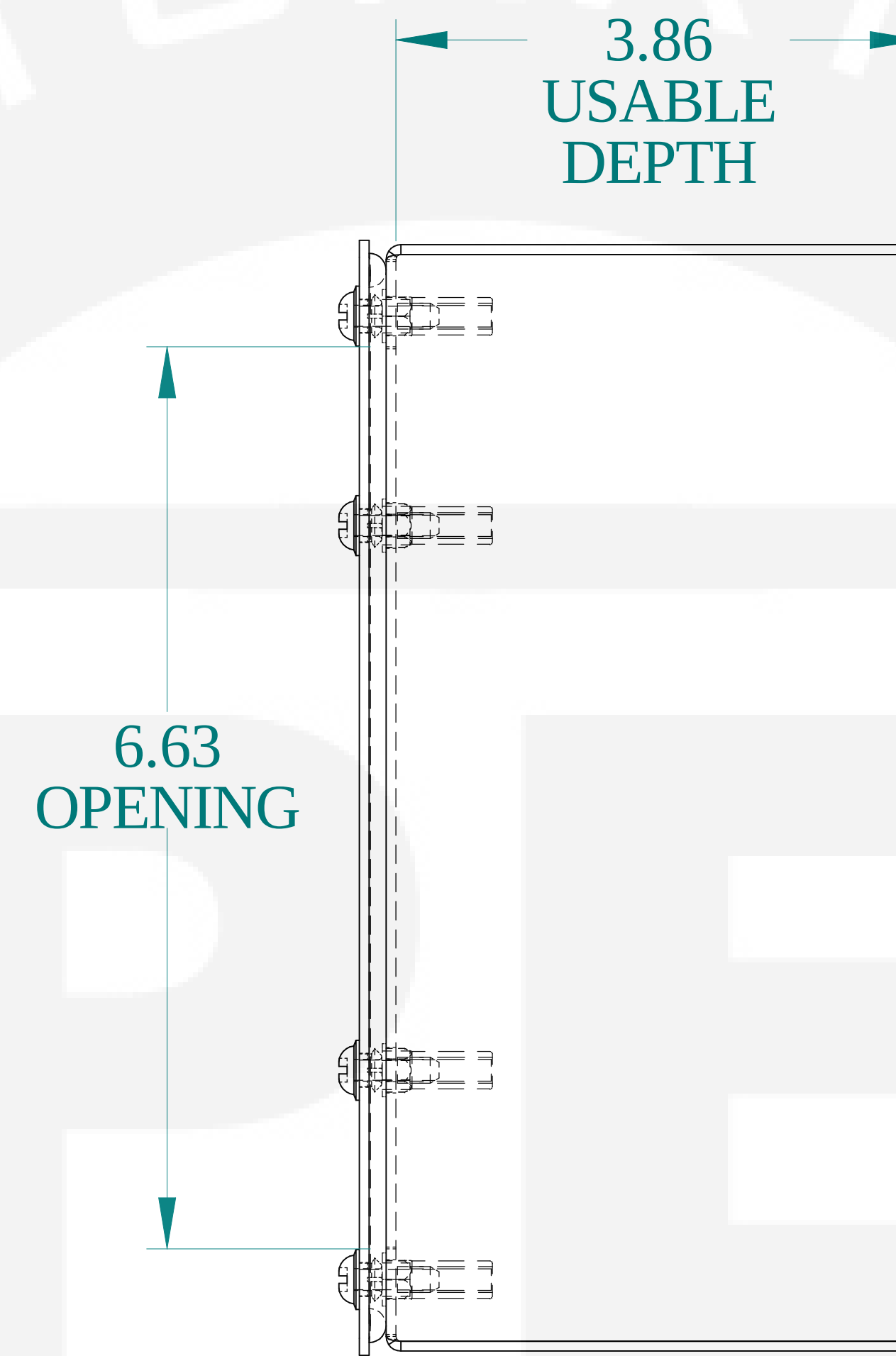
SIDE VIEW
