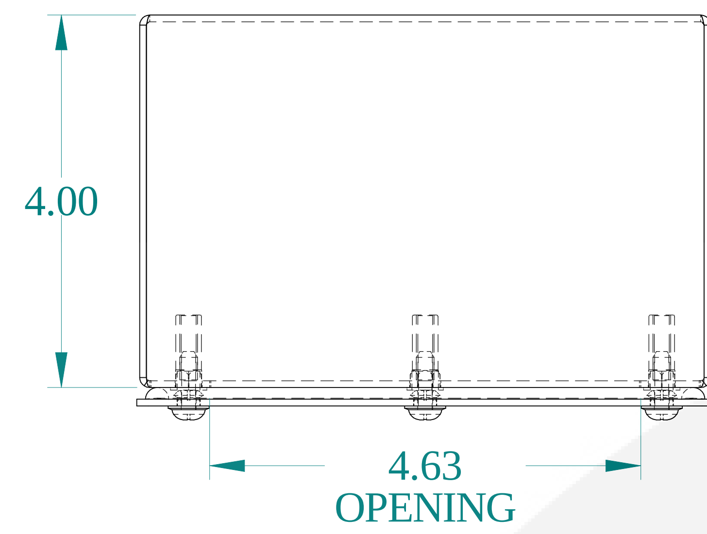
TOP VIEW
