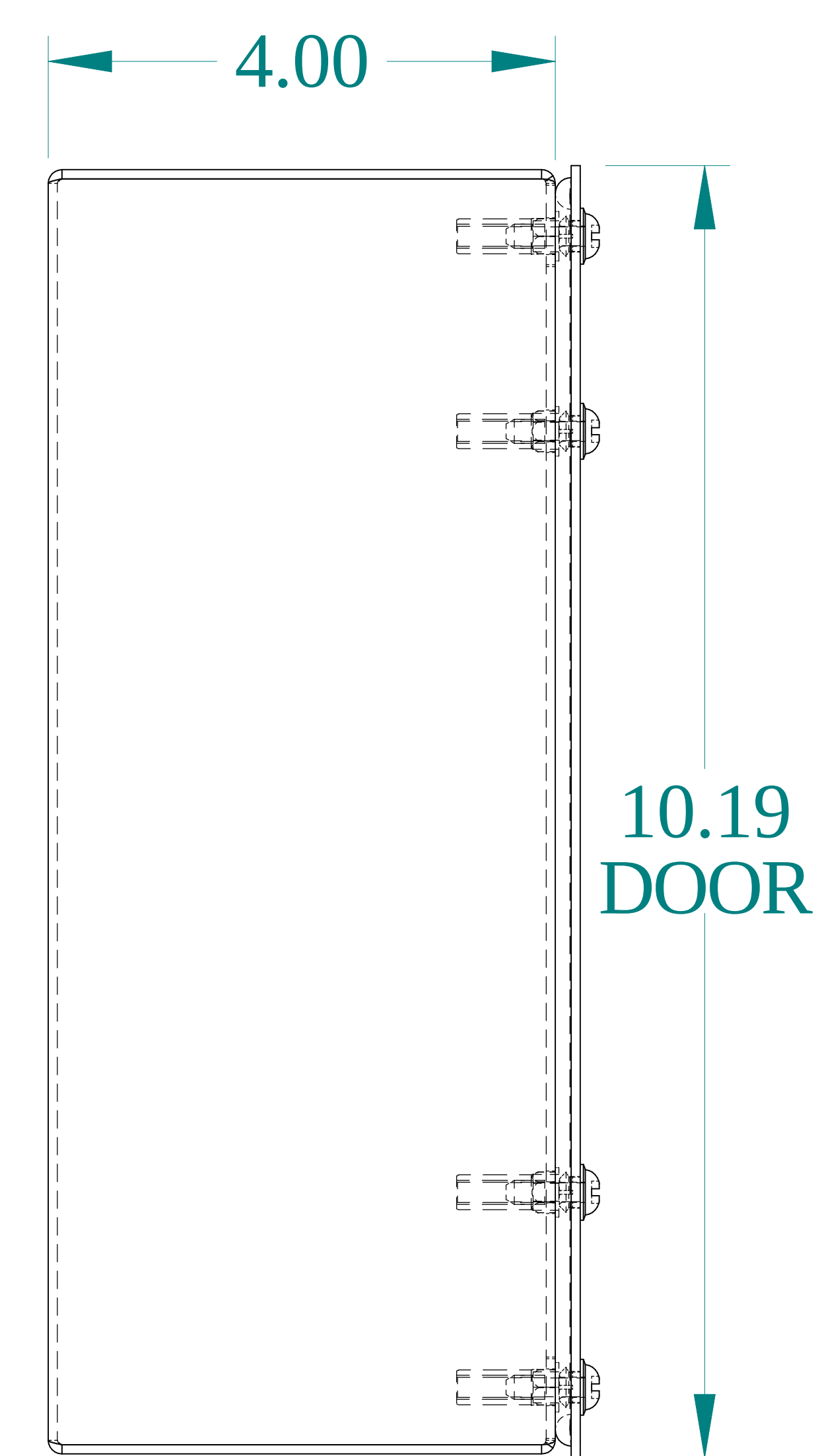
SIDE VIEW
