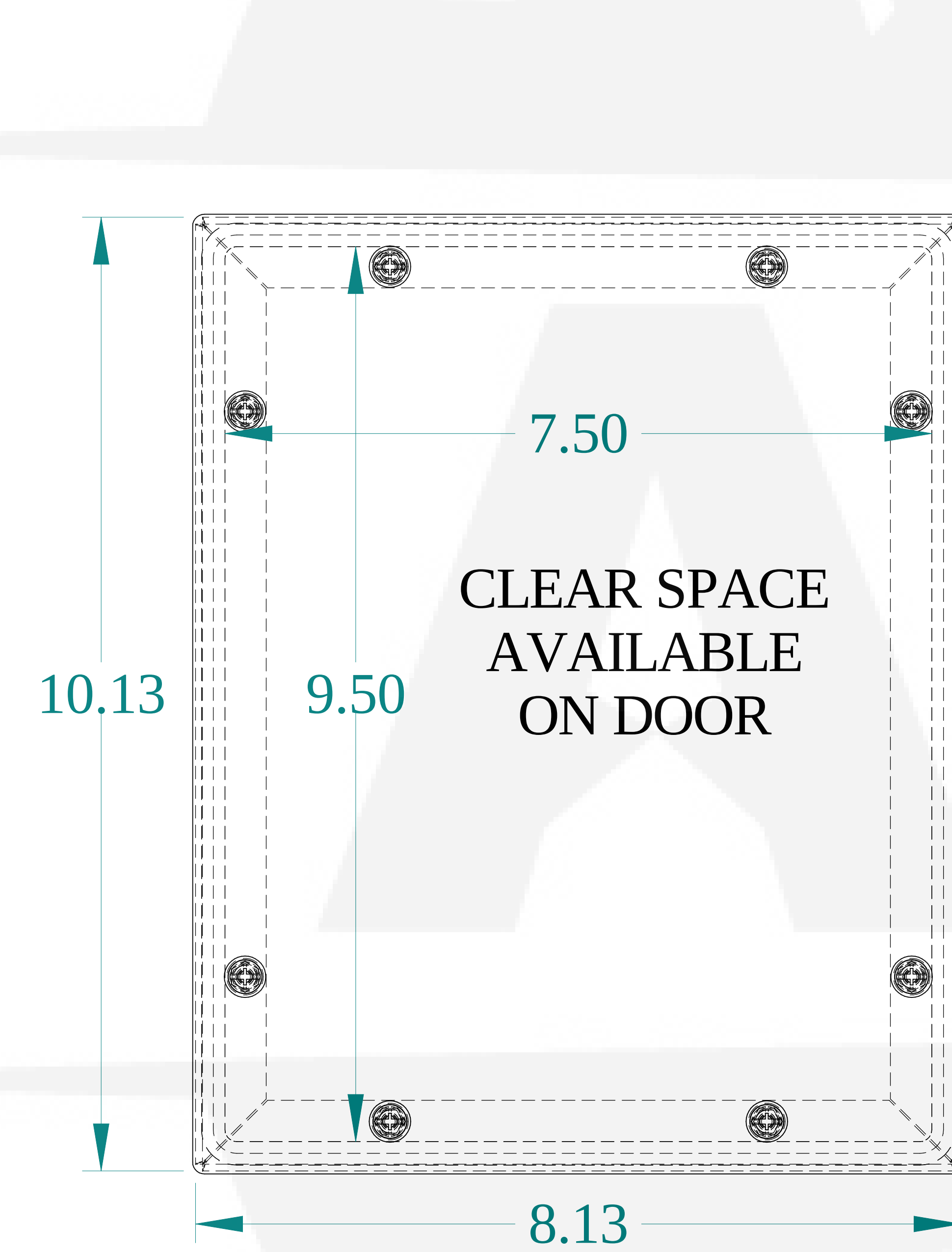
FRONT VIEW
