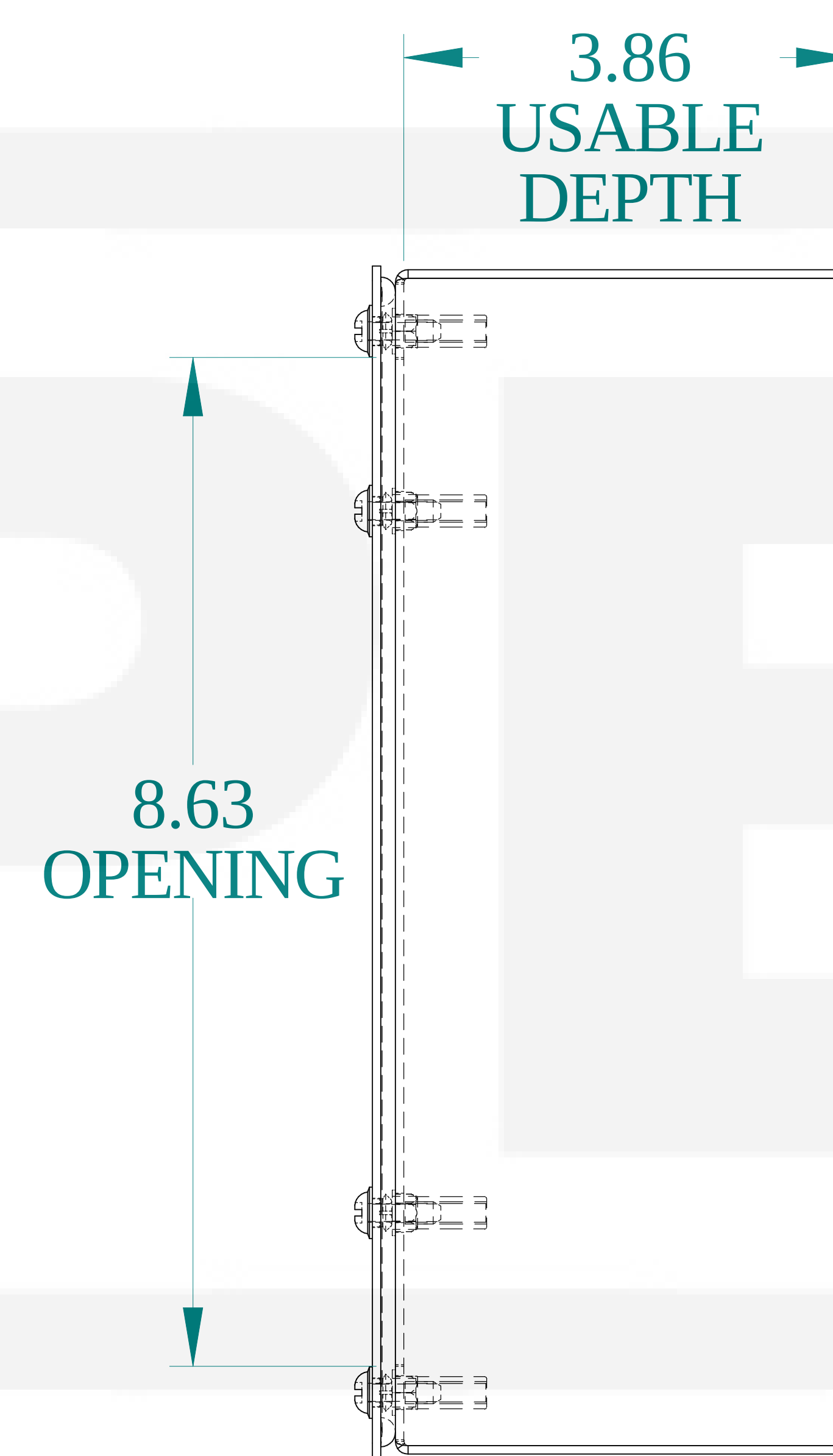
SIDE VIEW
